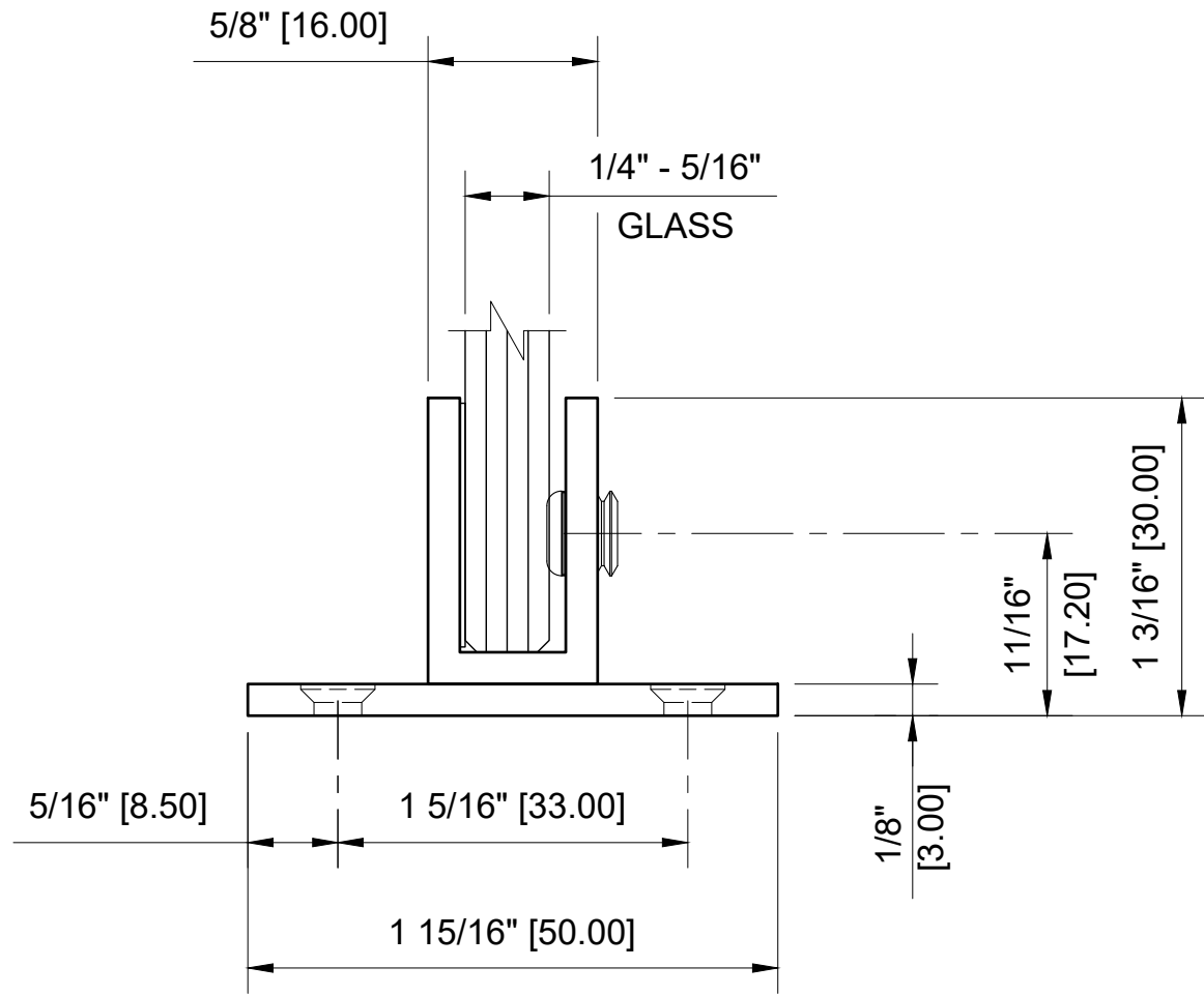
CRL - EH48 BRASS SHORT LEG SET SCREW CLAMP FOR 1/4" - 5/16" GLASS
