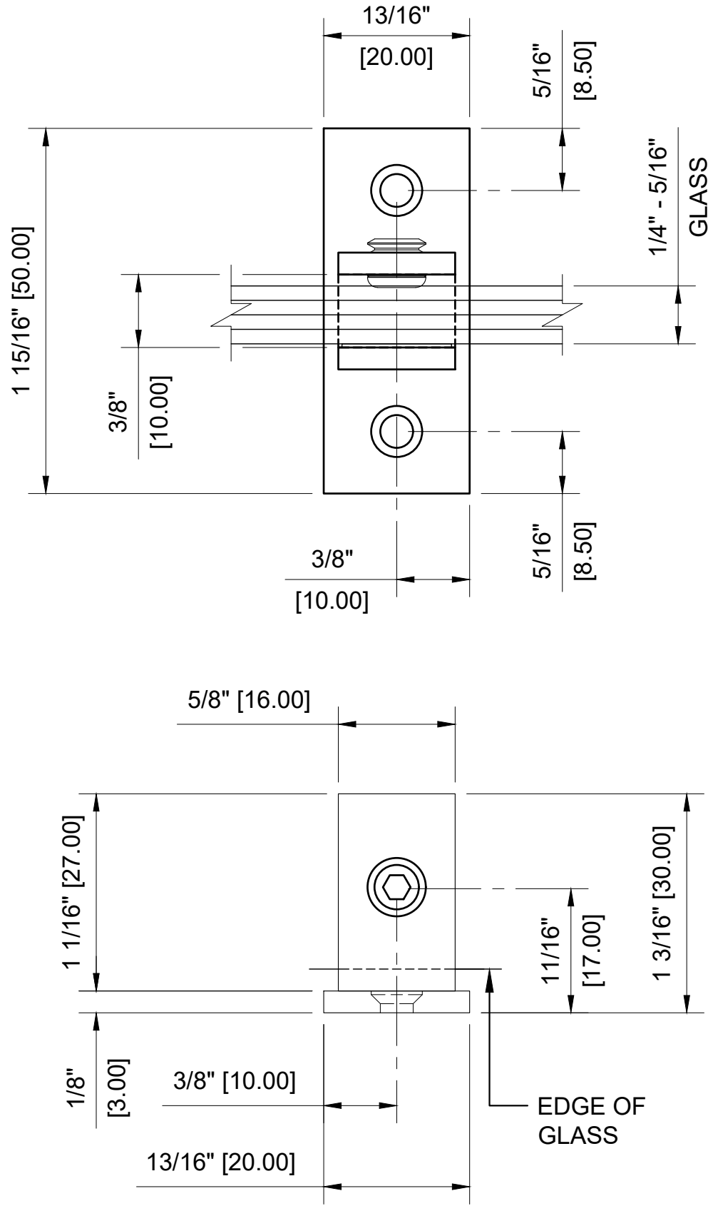
CRL - EH48 BRASS SHORT LEG SET SCREW CLAMP FOR 1/4" - 5/16" GLASS
