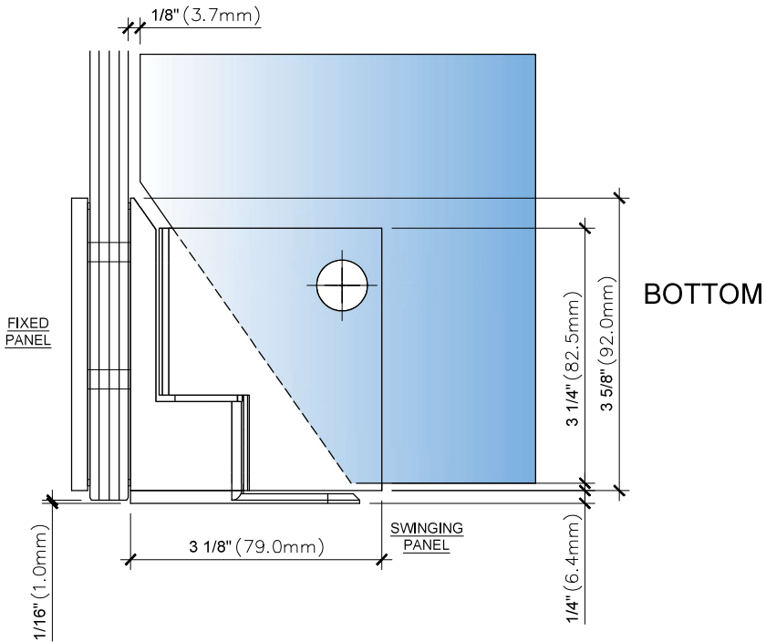
2A FRONT VIEW DETAIL - 1MM FIXED PANEL GAP
