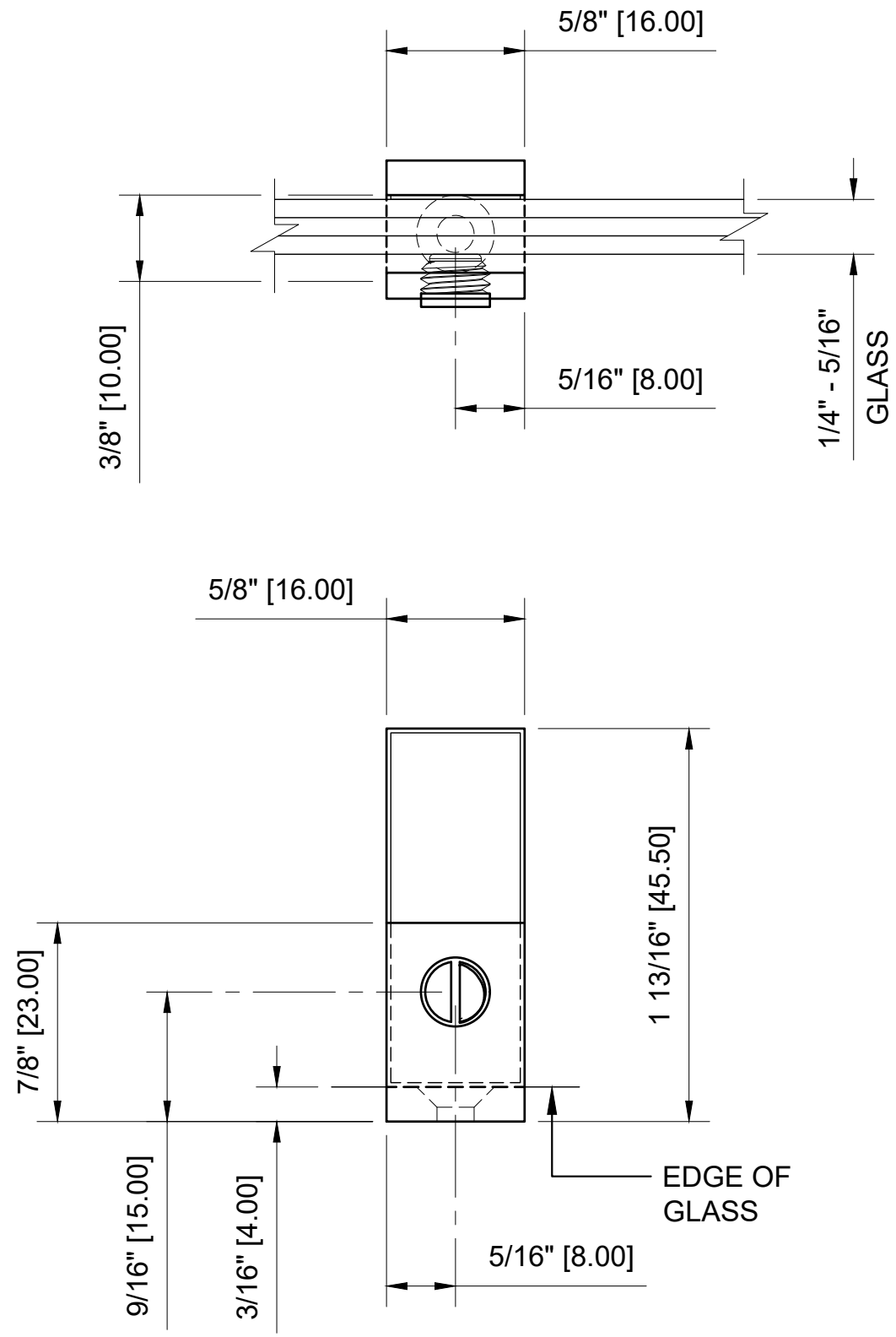
CRL - EH43 BRUSHED NICKEL SLIM LINE "J" SET SCREW CLAMPS FOR 1/4" TO 5/16" GLASS
