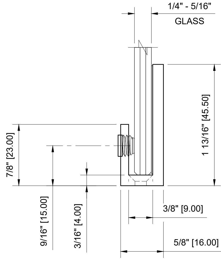
CRL - EH43 BRUSHED NICKEL SLIM LINE "J" SET SCREW CLAMPS FOR 1/4" TO 5/16" GLASS
