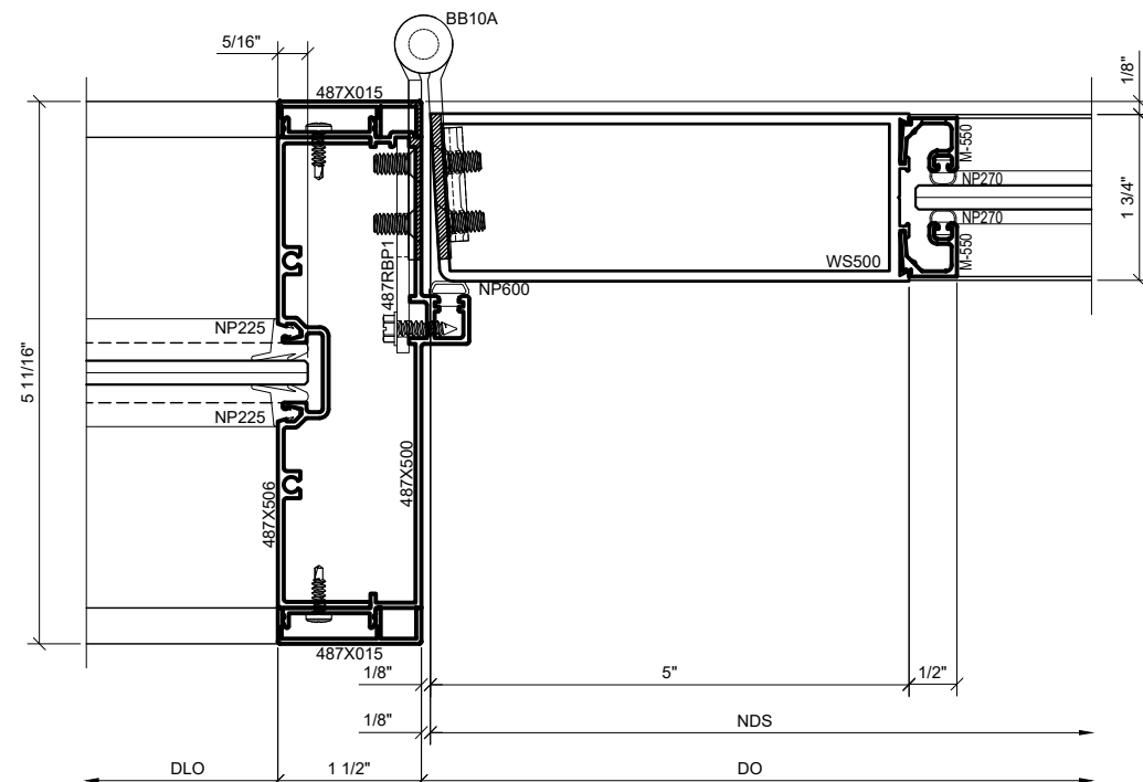
① DOOR JAMB DETAIL AT HINGE SIDE WITH SIDELITE W/ SERIES 550 WIDE STILE DOOR 1'-0" = 1'-0" ARCH. REF.: N/A
