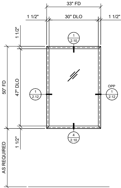
2 ELEVATION: BORROWED LITE ABOVE FLOOR 3/4" = 1'-0" ARCH. REF.: N/A
