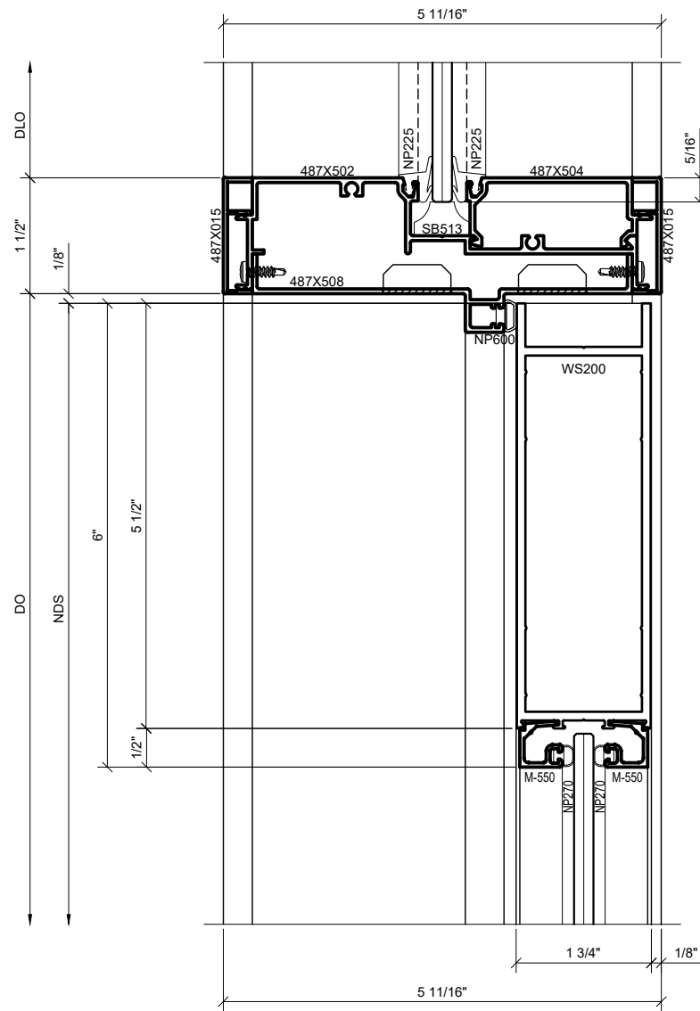
2 DOOR HEAD DETAIL AT TRANSOM WITH SERIES 550 WIDE STILE DOOR 1'-0" = 1'-0" ARCH. REF.: N/A
