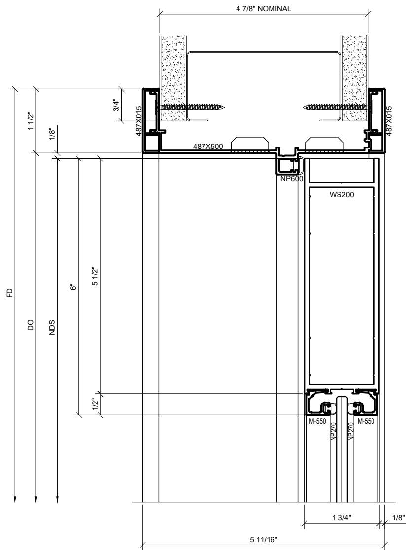
1 DOOR HEAD DETAIL WITH SERIES 550 WIDE STILE DOOR 1'-0" = 1'-0" ARCH. REF.: N/A
