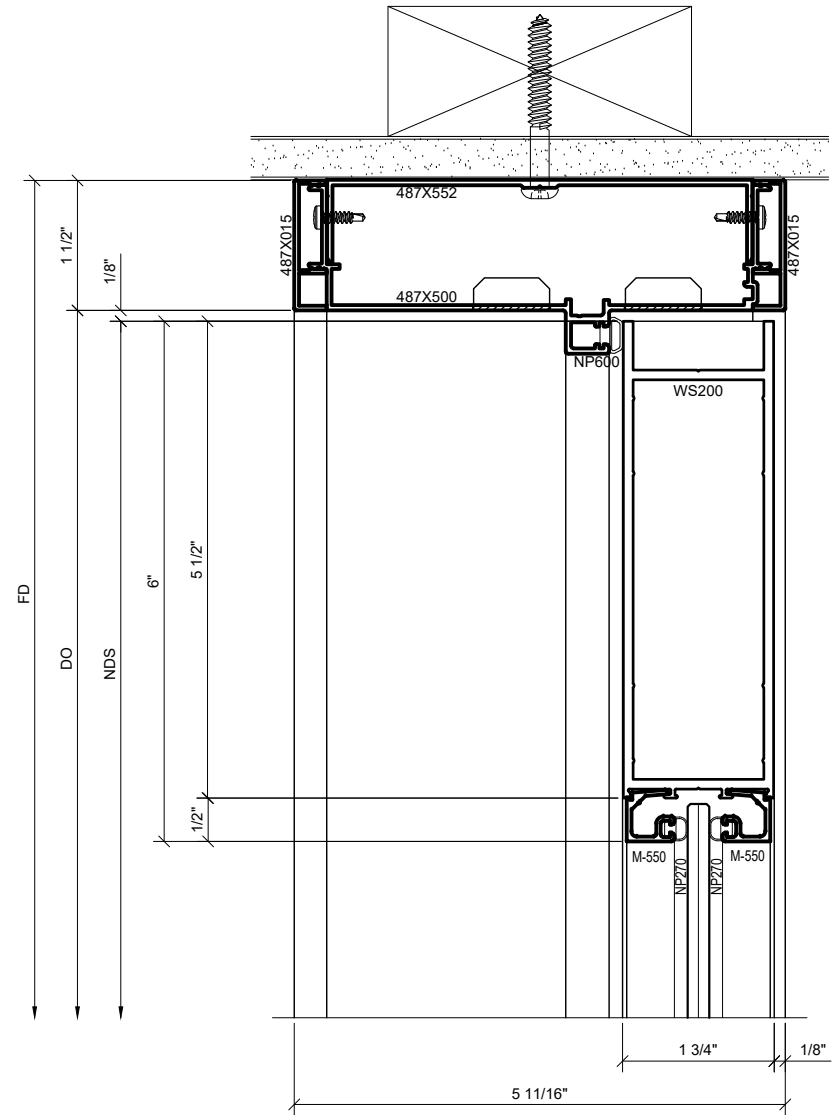
3 SURFACE MOUNTED DOOR HEAD DETAIL WITH SERIES 550 WIDE STILE DOOR 1'-0" = 1'-0" ARCH. REF.: N/A
