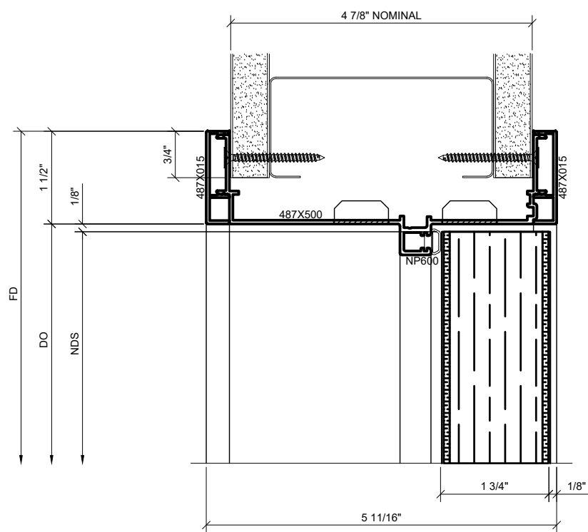
1 DOOR HEAD DETAIL WITH WOOD FLUSH DOOR
