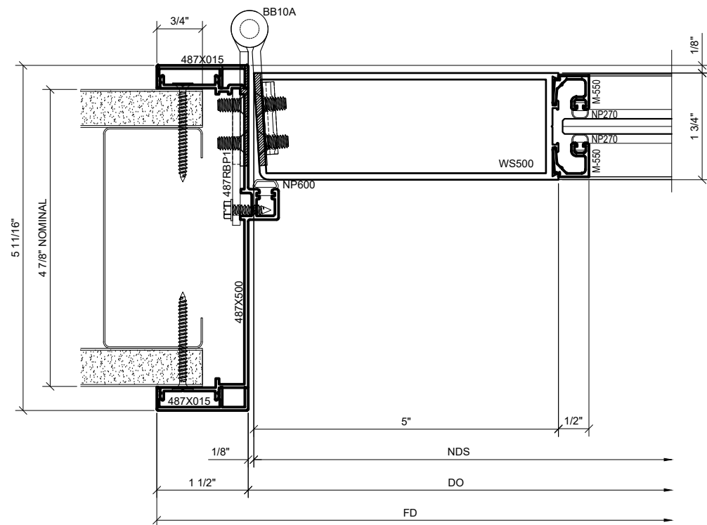
① DOOR JAMB DETAIL AT HINGE SIDE WITH SERIES 550 WIDE STILE DOOR 1'-0\"/>
