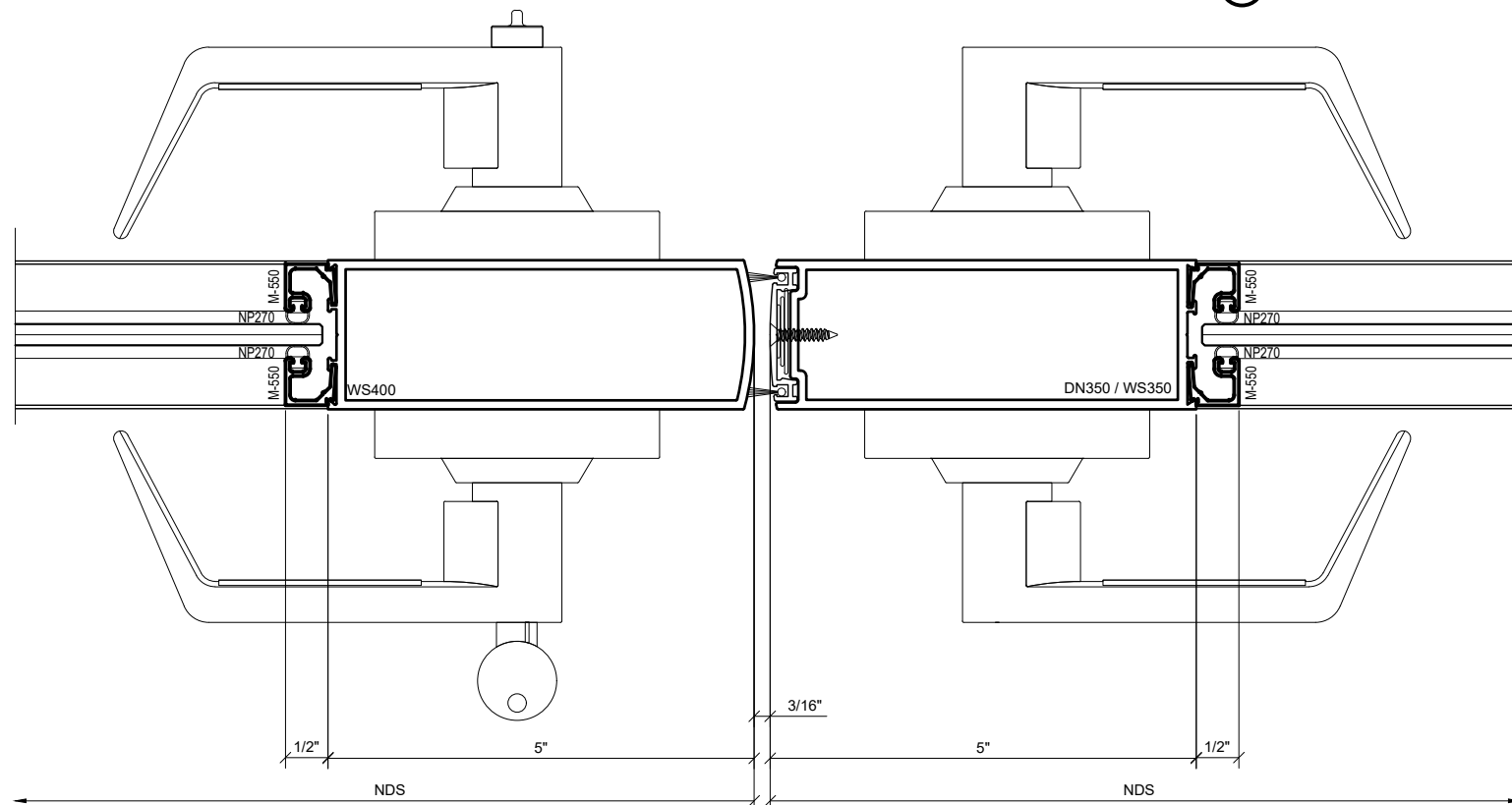
② MEETING STILES DETAIL WITH SERIES 550 WIDE STILE DOORS 1'-0\"/>
