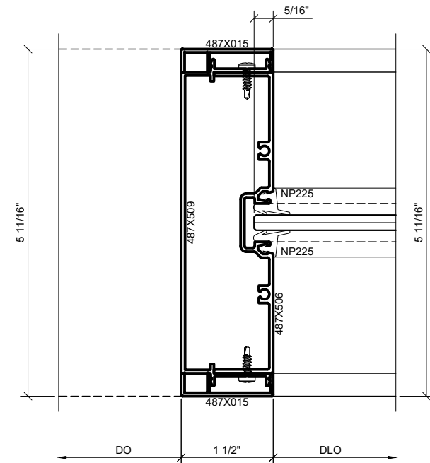
④ CASSED OPENING JAMB DETAIL AT SIDELITE 1'-0" = 1'-0" ARCH. REF.: N/A
