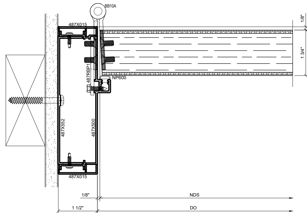
③ SURFACE MOUNT DOOR JAMB DETAIL AT HINGE SIDE WITH WOOD FLUSH DOOR 1'-0" = 1'-0" ARCH. REF.: N/A
