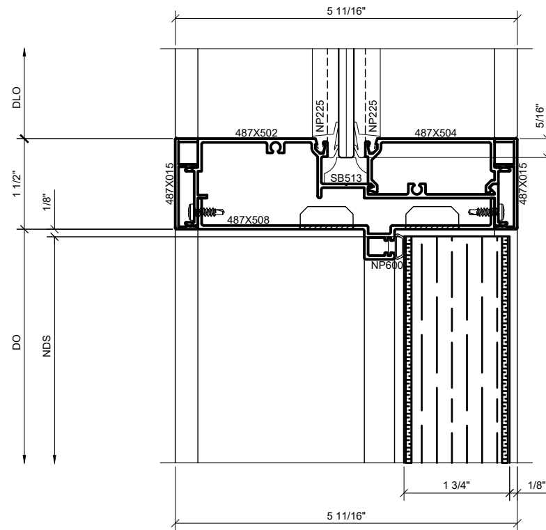
2 DOOR HEAD DETAIL AT TRANSOM WITH WOOD FLUSH DOOR
