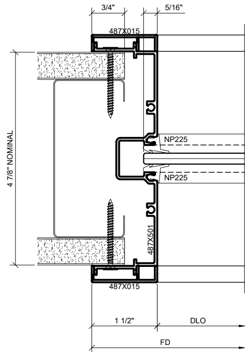
① WALL JAMB DETAIL AT SIDELITE / BORROWED LITE 1'-0" = 1'-0" ARCH. REF.: N/A
