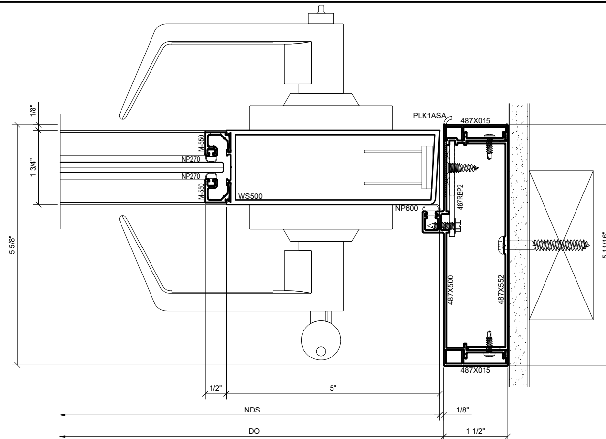
② SURFACE MOUNT DOOR JAMB DETAIL AT STRIKE SIDE W/ SERIES 550 WIDE STILE DOOR 1'-0" = 1'-0" ARCH. REF.: N/A
