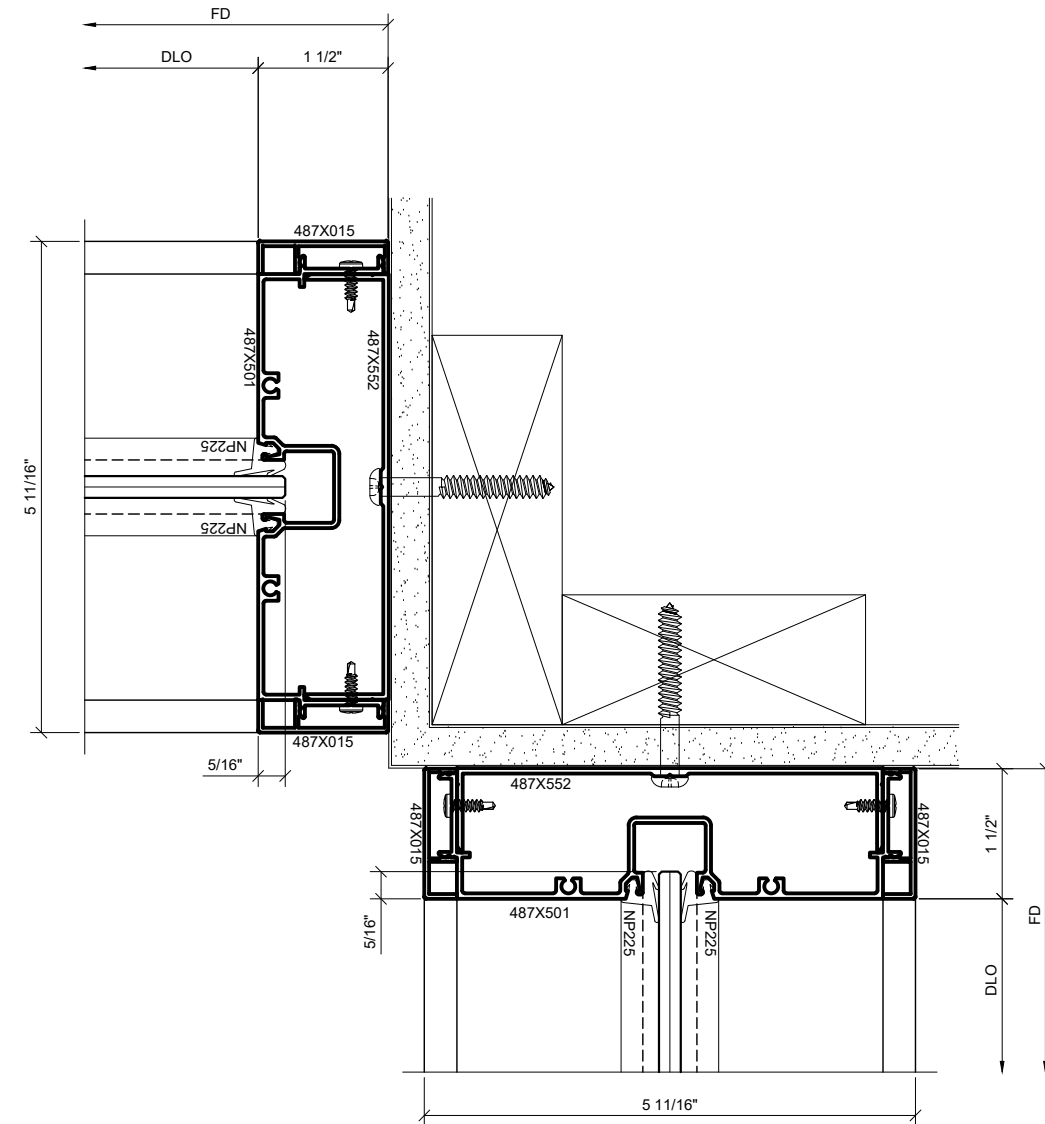
2 SURFACE MOUNT CORNER DETAIL: SIDELITE / BORROWED LITE 1'-0" = 1'-0" ARCH. REF.: N/A
