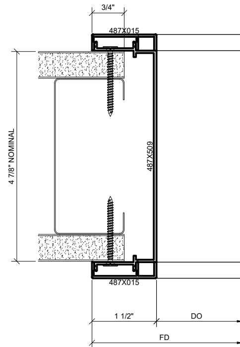
③ WALL JAM DETAIL AT CASSED OPENING 1'-0" = 1'-0" ARCH. REF.: N/A
