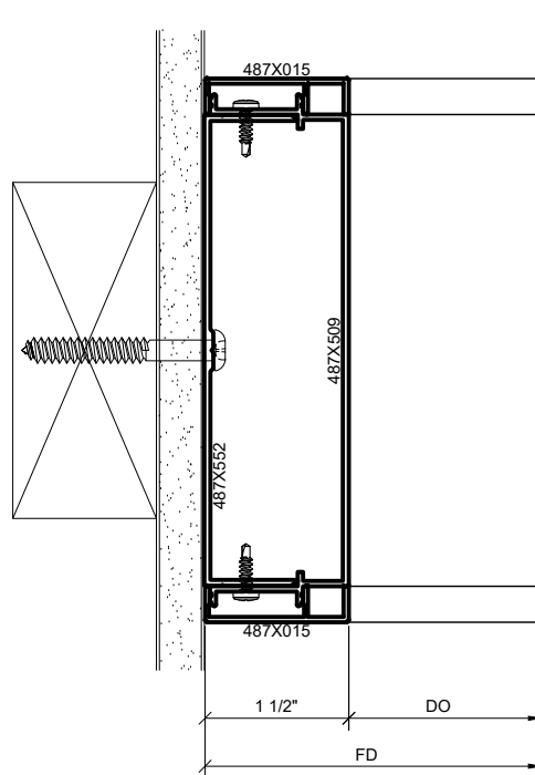
⑥ SURFACE MOUNT WALL JAMB DETAIL AT CASSED OPENING 1'-0" = 1'-0" ARCH. REF.: N/A
