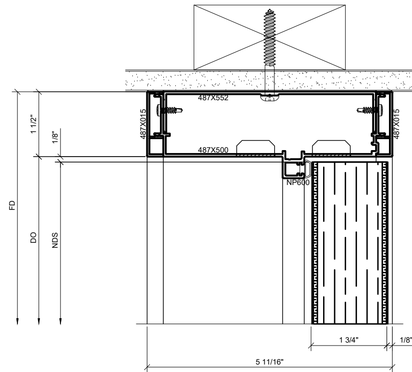
3 SURFACE MOUNTED DOOR HEAD DETAIL WITH WOOD FLUSH DOOR
