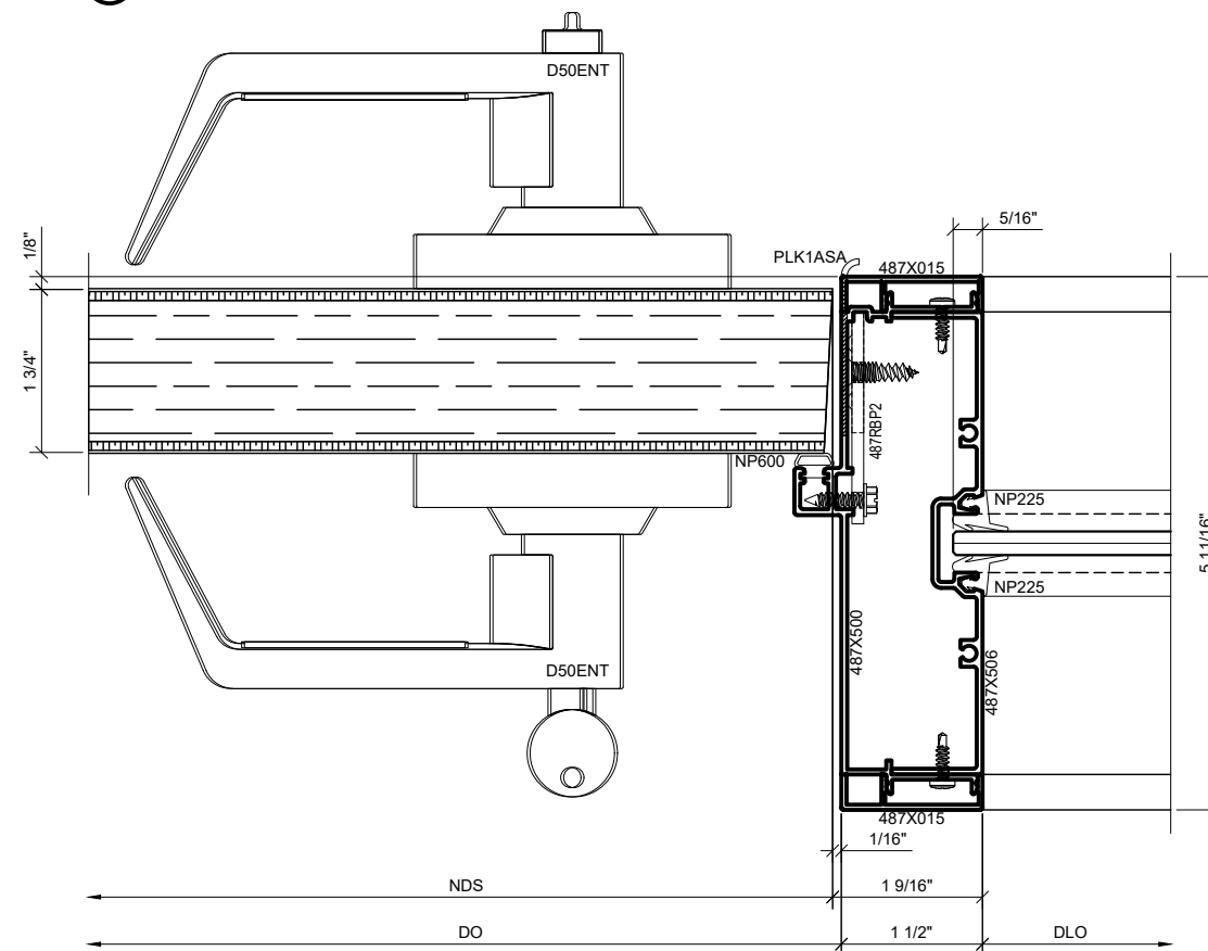
④ DOOR JAMB DETAIL AT STRIKE SIDE WITH SIDELITE W/ WOOD FLUSH DOOR 1'-0" = 1'-0" ARCH. REF.: N/A
