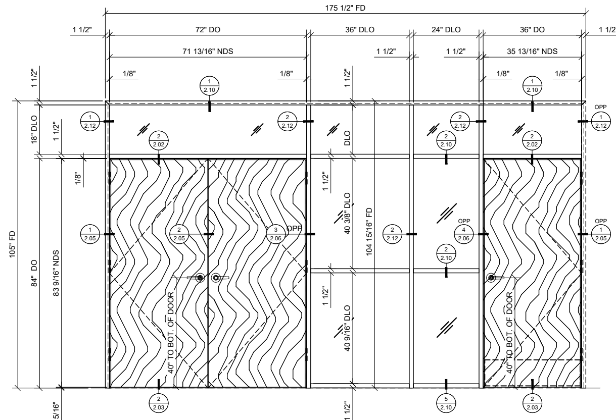
ELEVATION: WOOD DOORS WITH FULL HEIGHT SIDELITES AND TRANSOMS
