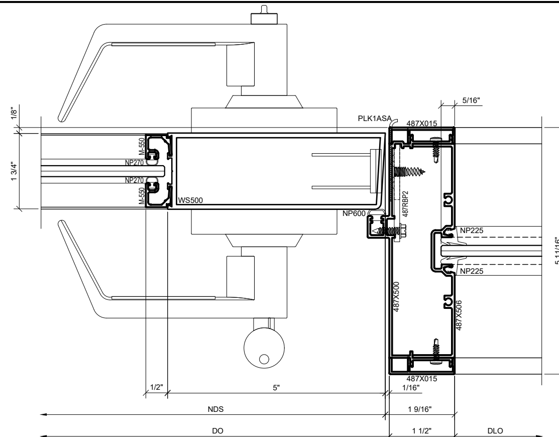
② DOOR JAMB DETAIL AT STRIKE SIDE WITH SIDELITE W/ SERIES 550 WIDE STILE DOOR 1'-0" = 1'-0" ARCH. REF.: N/A
