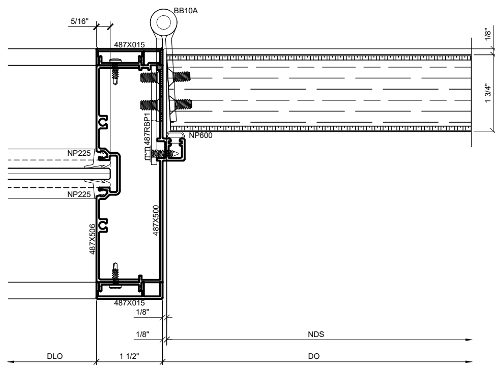
③ DOOR JAMB DETAIL AT HINGE SIDE WITH SIDELITE W/ WOOD FLUSH DOOR 1'-0" = 1'-0" ARCH. REF.: N/A
