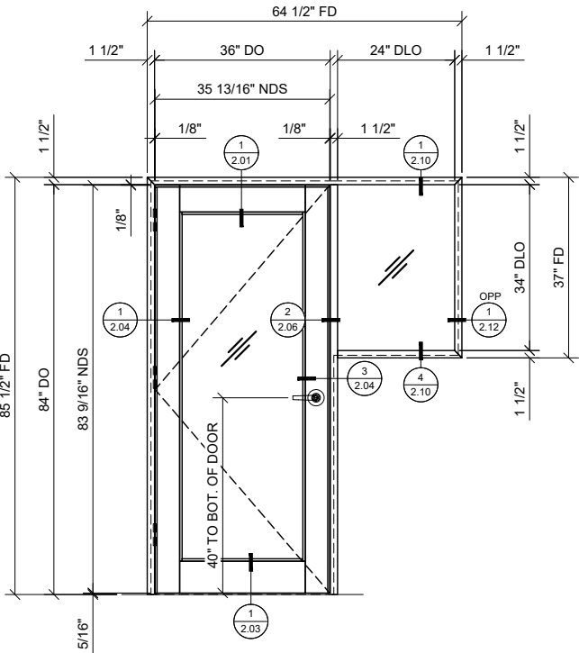
2 ELEVATION: ALUMINUM DOOR WITH ABOVE FLOOR SIDELITE 3/4" = 1'-0" ARCH. REF.: N/A
