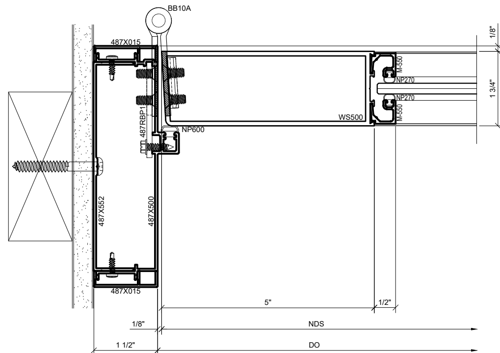
① SURFACE MOUNT DOOR JAMB DETAIL AT HINGE SIDE W/ SERIES 550 WIDE STILE DOOR 1'-0" = 1'-0" ARCH. REF.: N/A
