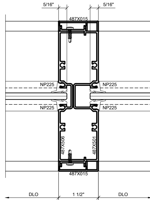
② INTERMEDIATE VERTICAL DETAIL AT SIDELITE 1'-0" = 1'-0" ARCH. REF.: N/A
