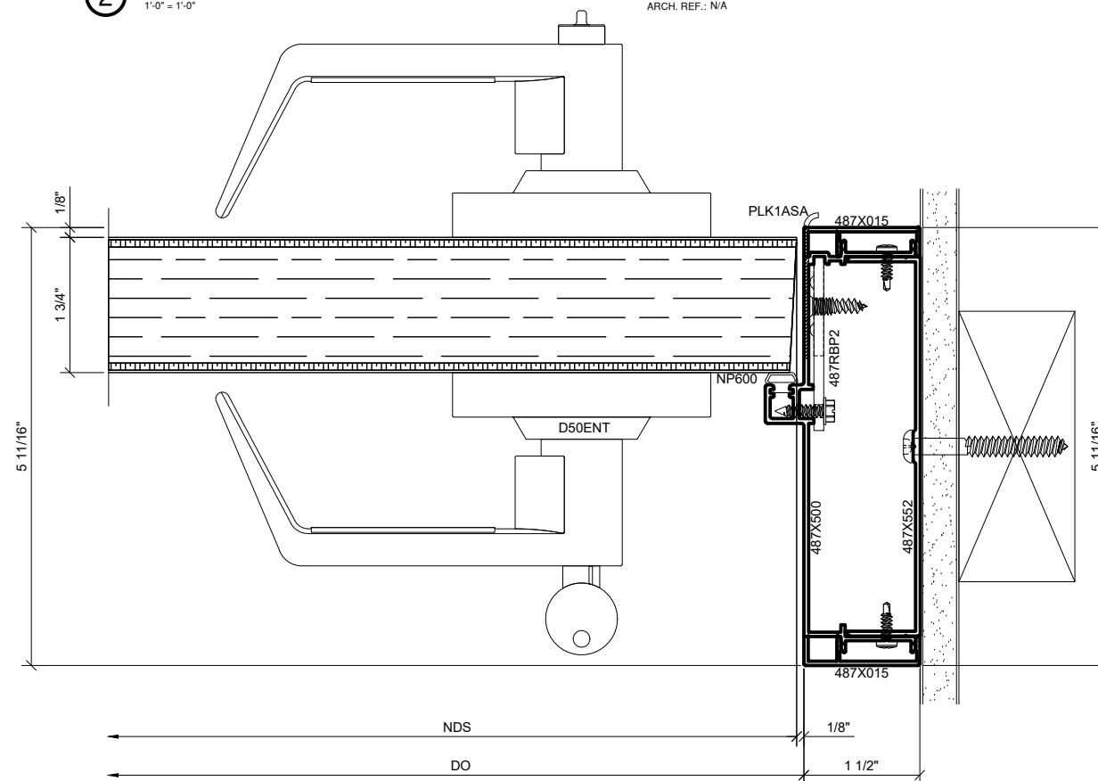
④ SURFACE MOUNT DOOR JAMB DETAIL AT STRIKE SIDE WITH WOOD FLUSH DOOR 1'-0" = 1'-0" ARCH. REF.: N/A
