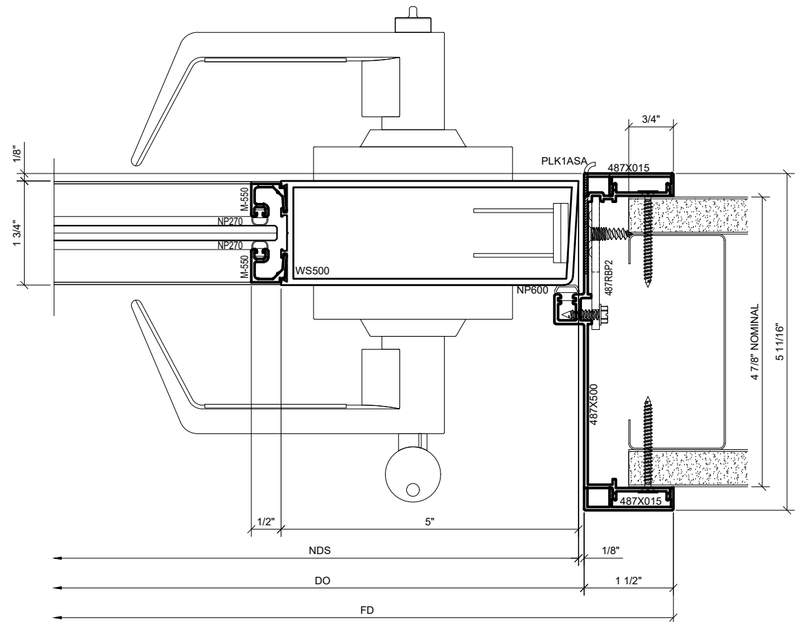
③ DOOR JAMB DETAIL AT STRIKE SIDE WITH SERIES 550 WIDE STILE DOOR 1'-0\"/>
