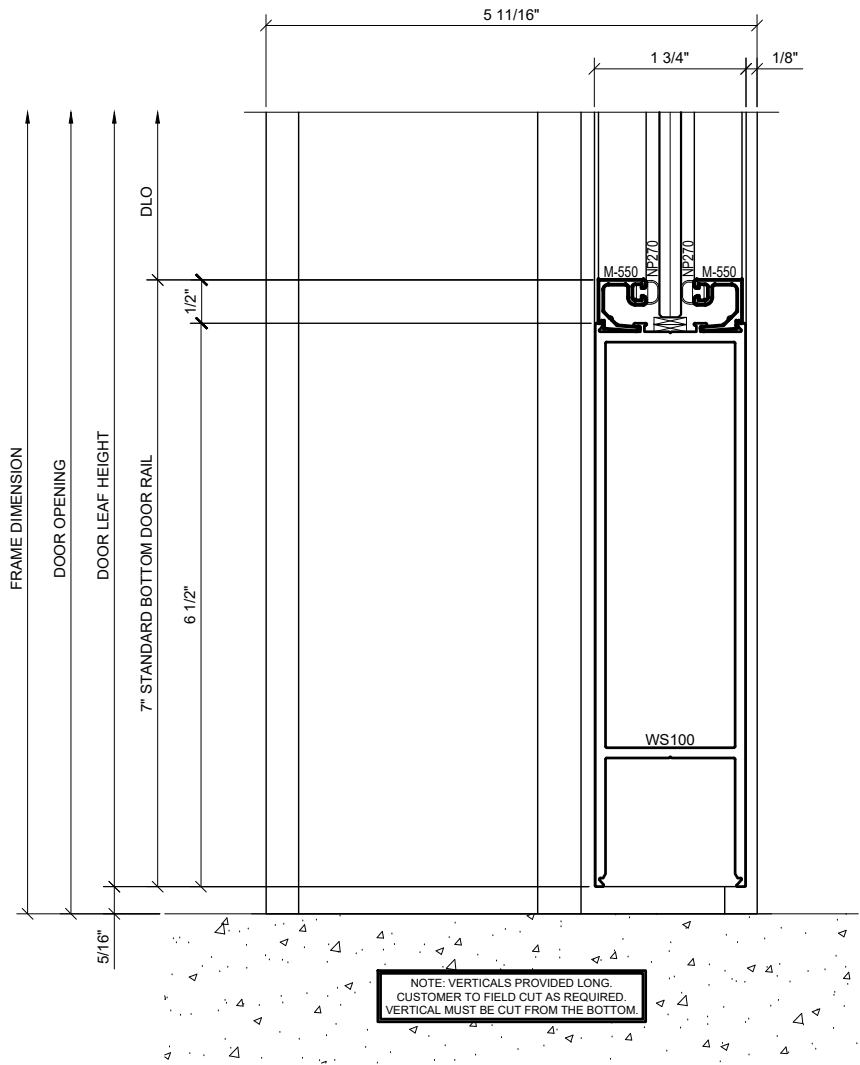
1 DOOR SILL DETAIL WITH SERIES 550 WIDE STILE DOOR 1'-0" = 1'-0" ARCH. REF.: N/A
