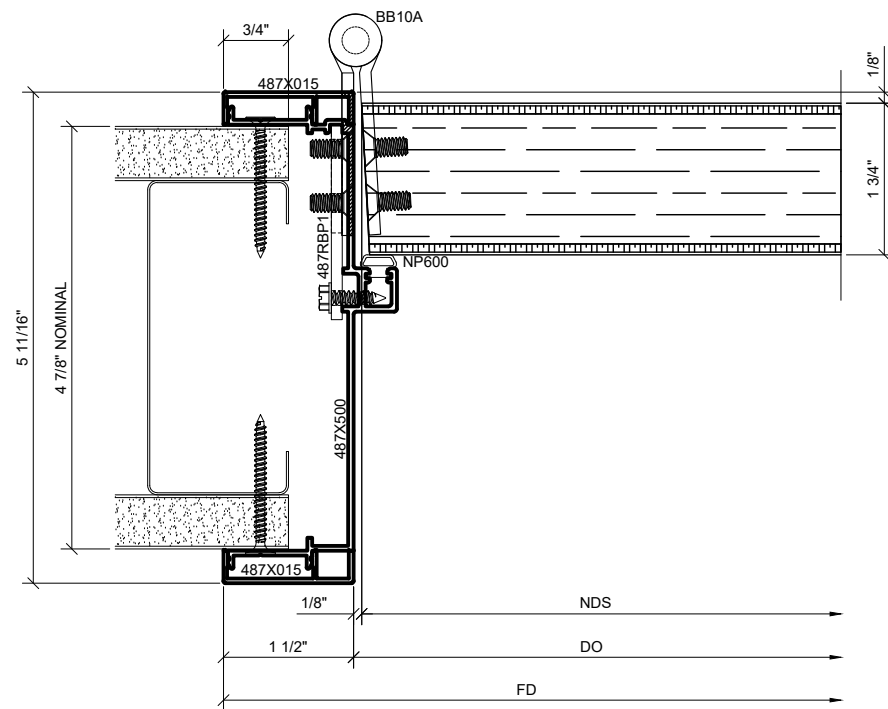
1 DOOR JAMB DETAIL AT HINGE SIDE WITH WOOD FLUSH DOOR 1'-0" = 1'-0" ARCH. REF.: N/A
