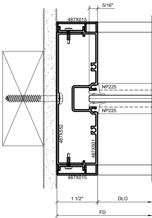
⑤ SURFACE MOUNT WALL JAMB DETAIL AT SIDELITE / BORROWED LITE 1'-0" = 1'-0" ARCH. REF.: N/A
