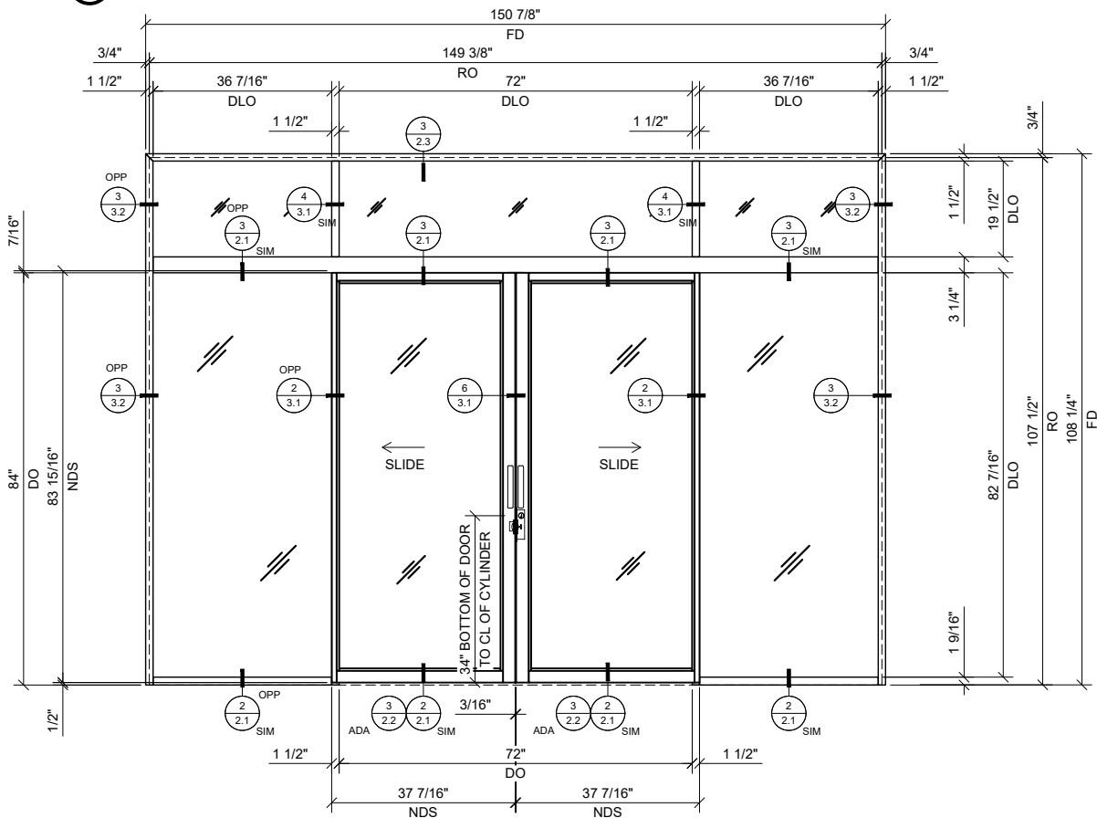
② BI-PART SLIDER WITH BAY & TRANSOM
