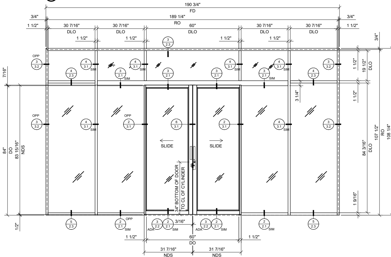
② BI-PART SLIDER WITH BAY, TRANSOM & SIDELITES AT EACH END
