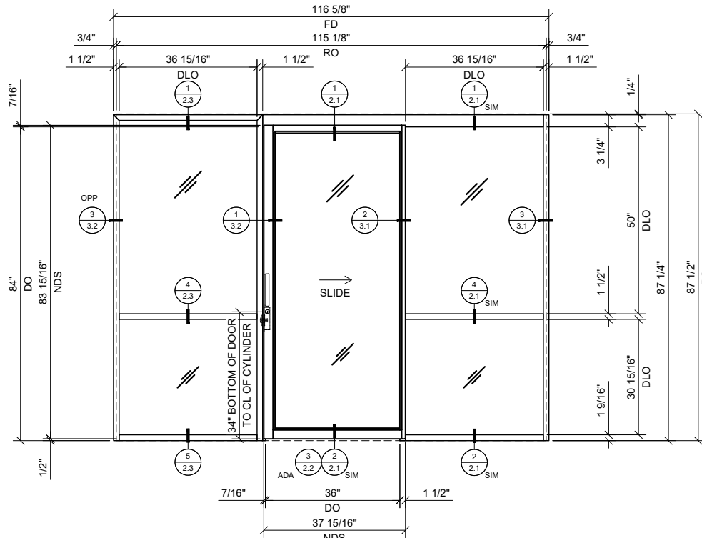
③ SINGLE SLIDER WITH BAY & SIDELITE 3/4\" = 1'-0\" ARCH. REF.: N/A
