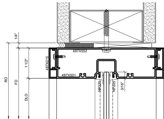
SERIES 487 OPS SURFACE MOUNT HEAD DETAIL AT SIDELITE (w/ SHIM)
