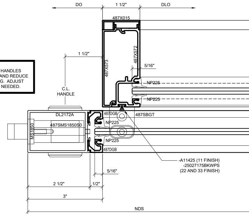
② SERIES 487 OPS INTEGRATED SLIDER TRANSITION VERTICAL-STANDARD TO INTERMEDIATE JAMB DETAIL (OPEN)
