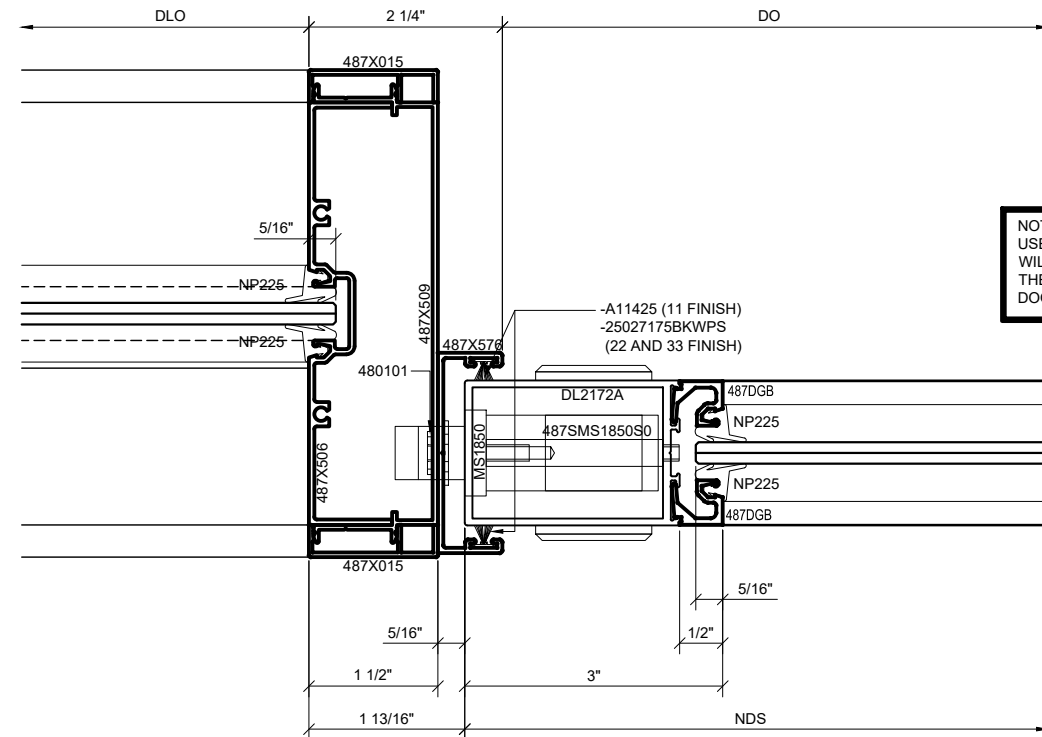
① SERIES 487 OPS INTEGRATED SLIDER TRANSITION VERTICAL-STANDARD TO STRIKE JAMB (CLOSED)
