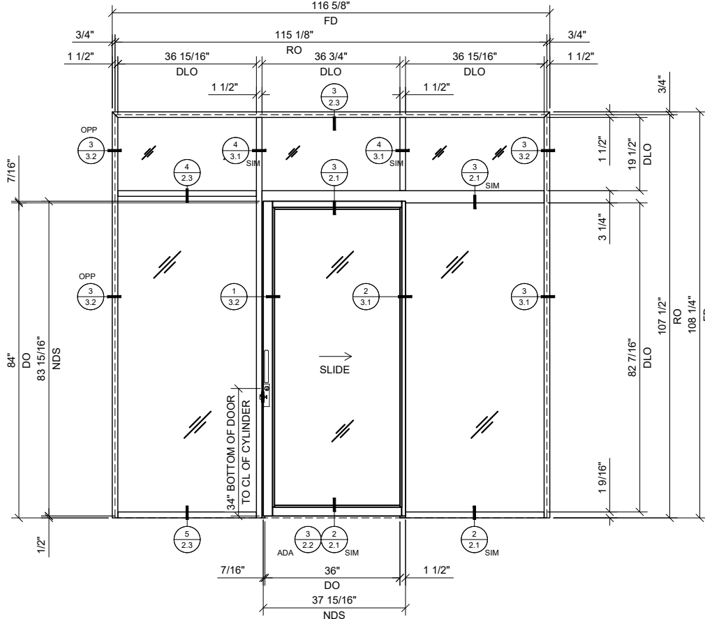
4 SINGLE SLIDER WITH BAY, TRANSOM & SIDELITE 3/4\" = 1'-0\" ARCH. REF.: N/A
