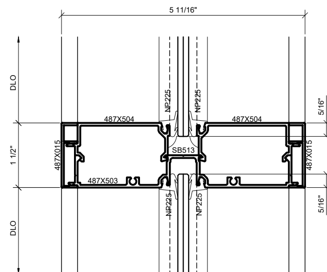
4 SERIES 487 OPS TYP HORIZONTAL DETAIL 1'-0"=1'-0" ARCH REF: N/A
