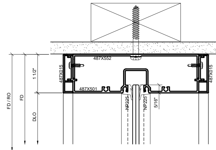
SERIES 487 OPS SURFACE MOUNT HEAD DETAIL AT SIDELITE (NO SHIM) 1'-0"=1'-0" ARCH REF: N/A
