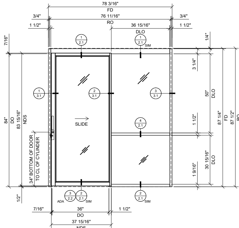
① SINGLE SLIDER WITH BAY 3/4\" = 1'-0\" ARCH. REF.: N/A
