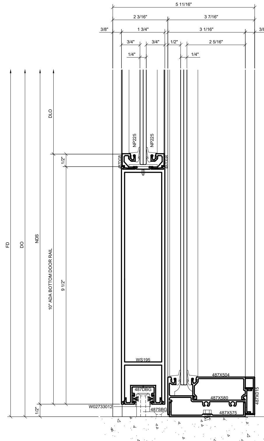
③ ADA SILL AT SLIDER DOOR OPENING 1'-0"=1'-0" ARCH REF: N/A
