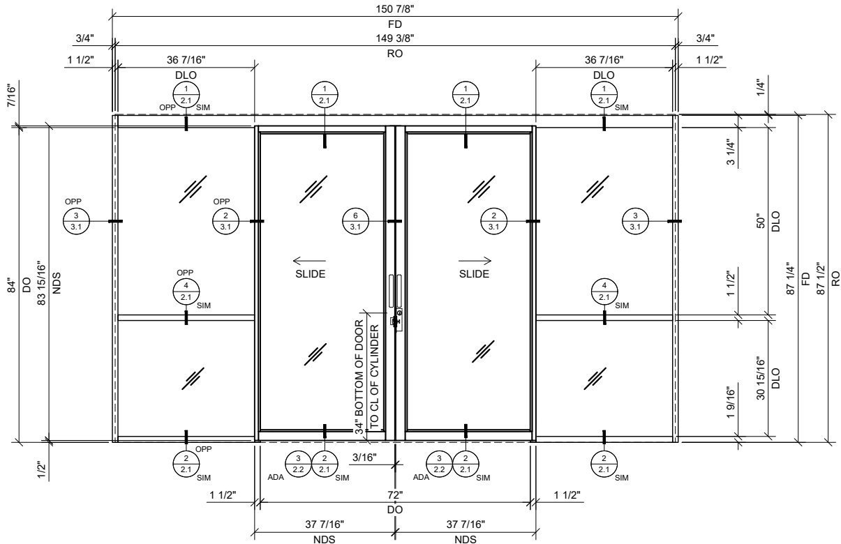
1 BI-PART SLIDER WITH BAYS 3/4\"=1'-0\" ARCH REF: N/A
