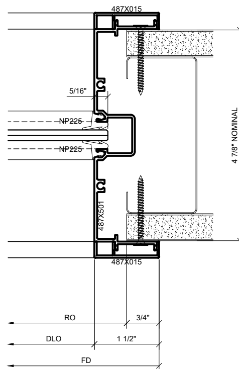
③ SERIES 487 OPS STANDARD JAMB DETAIL
