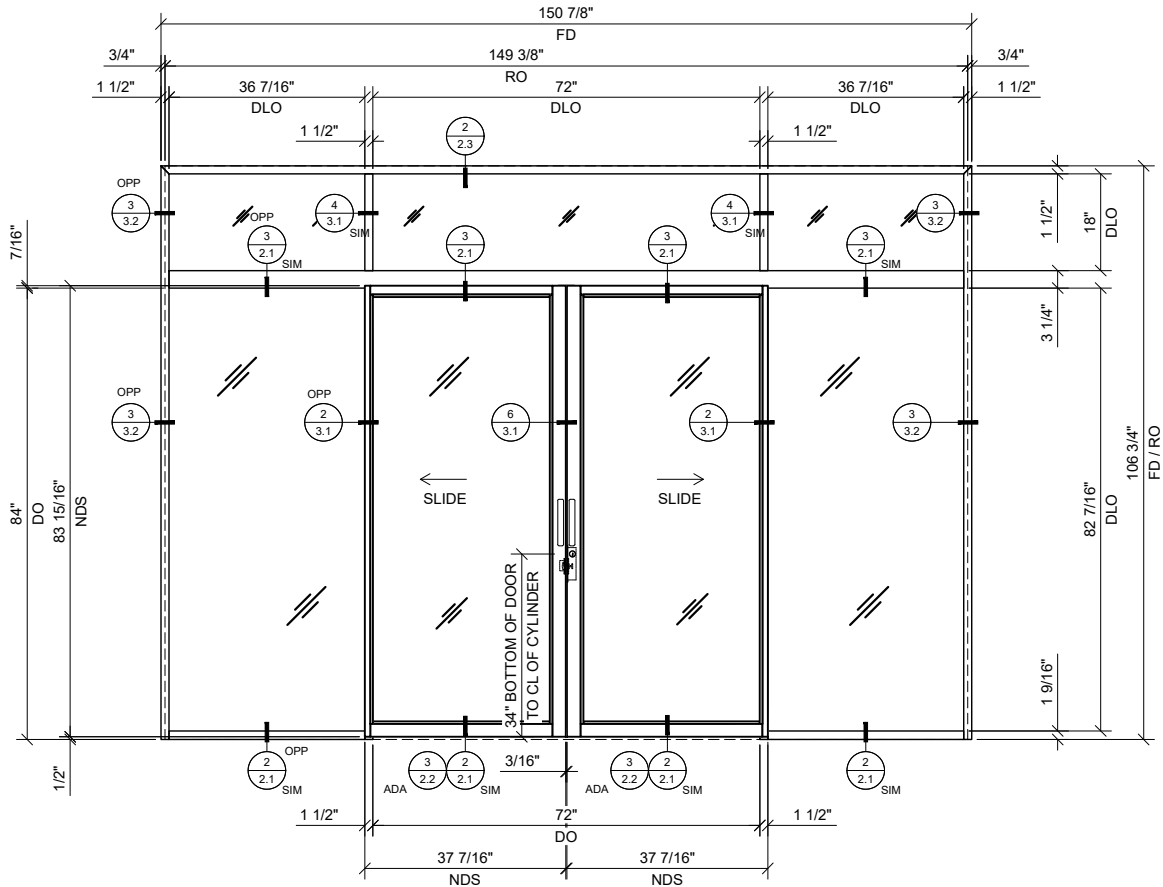
2 BI-PART SLIDER WITH BAY, TRANSOM 3/4\"=1'-0\" ARCH REF: N/A
