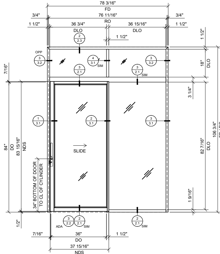
② SINGLE SLIDER WITH BAY & TRANSOM 3/4\" = 1'-0\" ARCH. REF.: N/A
