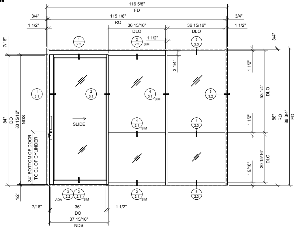
1 SINGLE SLIDER WITH BAY & SIDELITE
