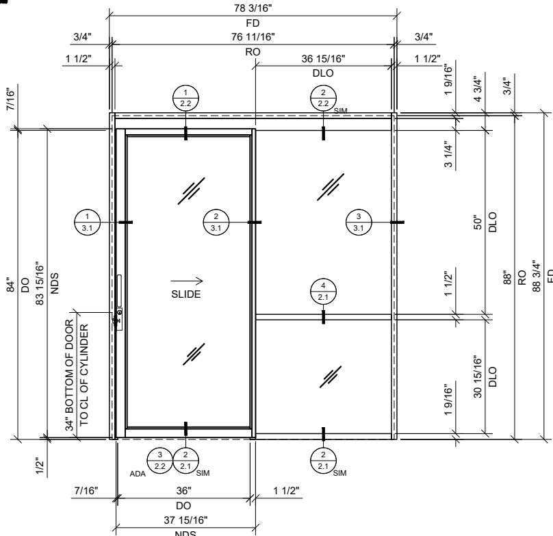
1 SINGLE SLIDER WITH BAY 3/4\" = 1'-0\" ARCH. REF.: N/A
