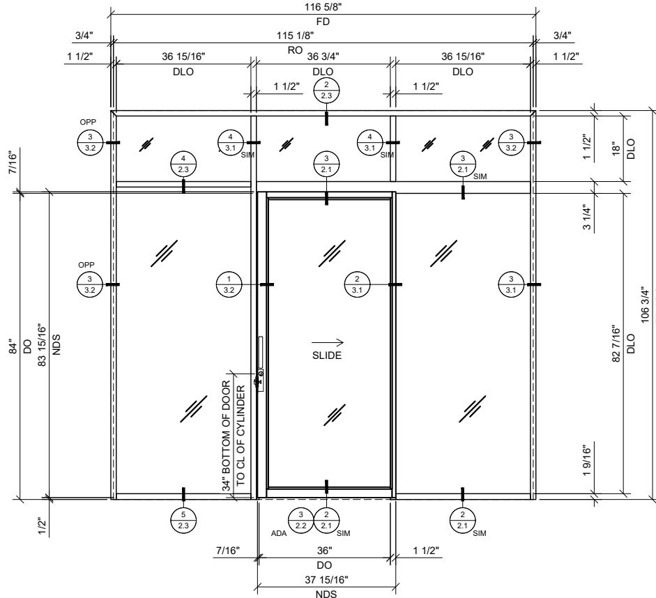
④ SINGLE SLIDER WITH BAY, TRANSOM & SIDELITE 3/4\" = 1'-0\" ARCH. REF.: N/A
