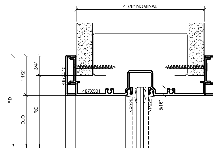
3 SERIES 487 OPS TRANSOM HEAD DETAIL AT INT. VERTICAL 1'-0"=1'-0" ARCH REF: N/A
