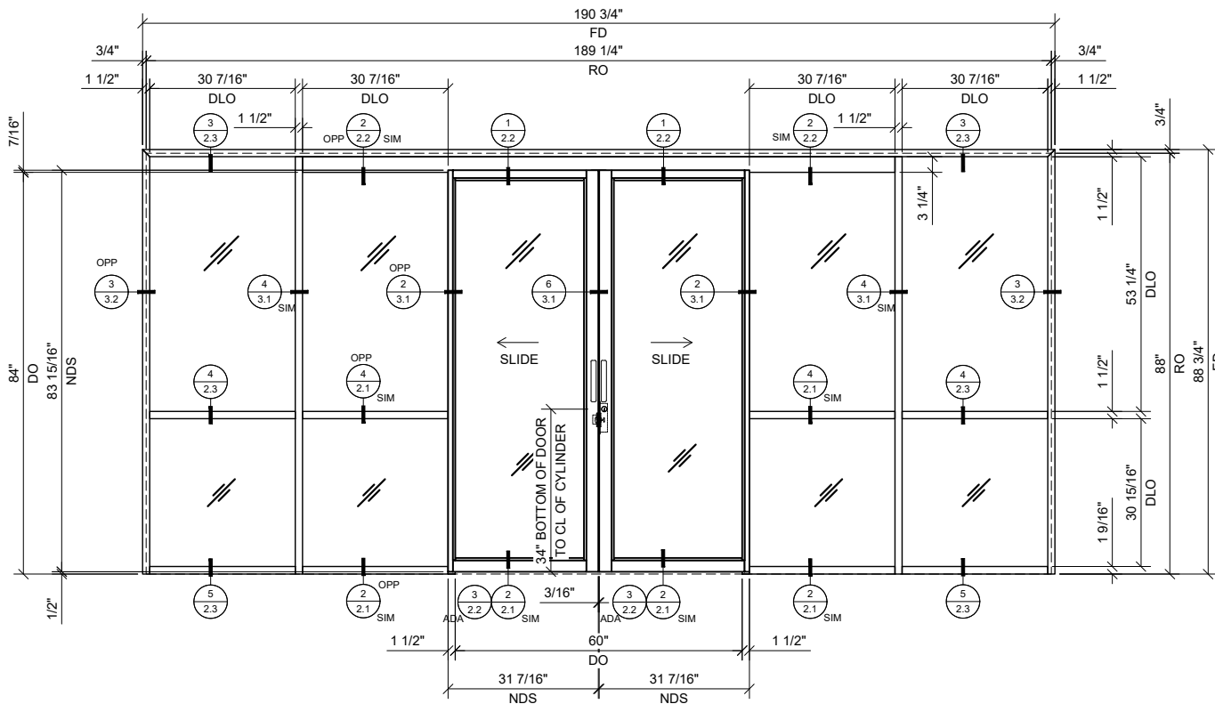
③ BI-PART SLIDER WITH BAY & SIDELITES AT EACH END
