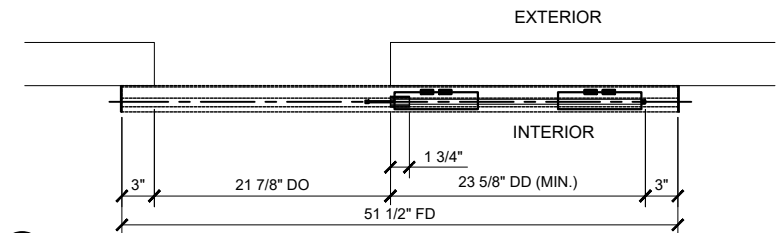
④ CRL690 PLAN (OPEN POSITION)
