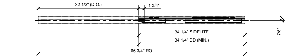
④ CRL6951 PLAN (OPEN POSITION)
