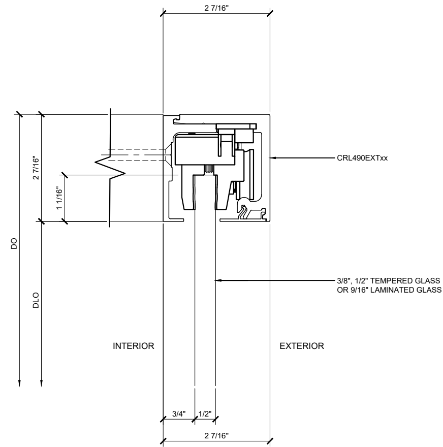
③ WALL MOUNTING CRL690, CRL690BSA, CRL695 & CRL695BSA HEADER DETAIL ARCH REF: NONE 1'-0"=1'-0"
