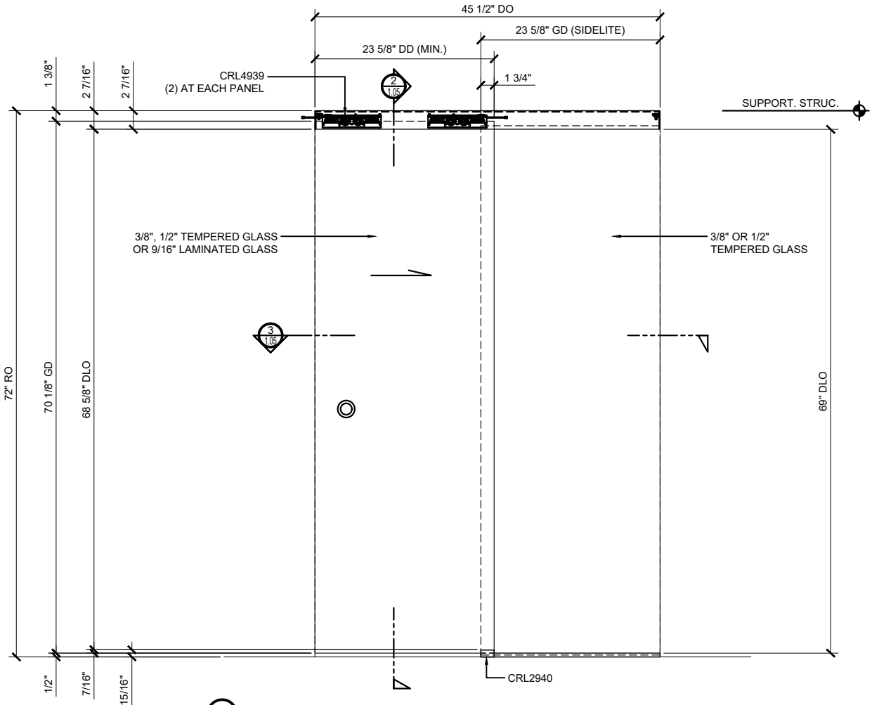
① CRL6901 SLIDING DOOR ELEVATION
