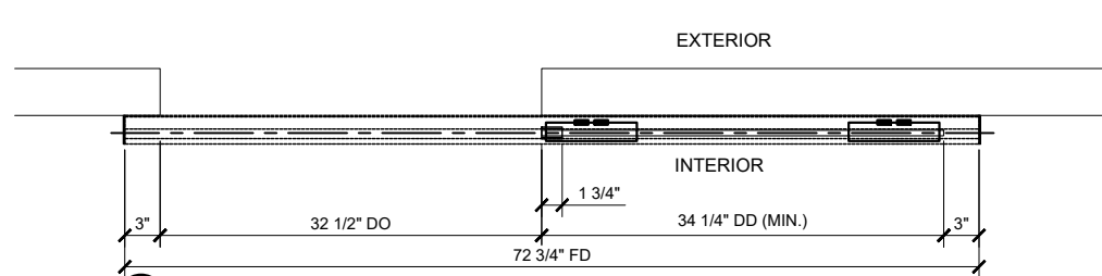
④ CRL695 PLAN (OPEN POSITION)
