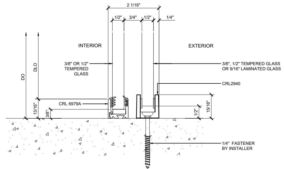
④ CRL6901, CRL6901BSA, CRL6951 & CRL6951BSA SILL DETAIL
