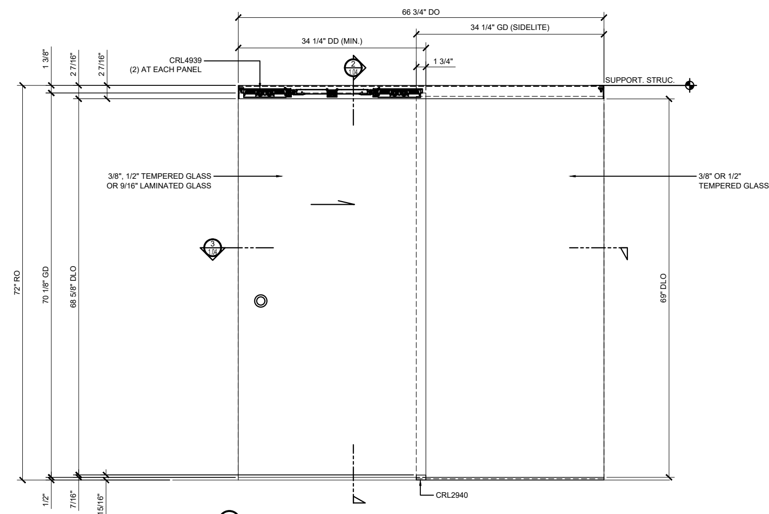
① CRL6951 SLIDING DOOR ELEVATION
