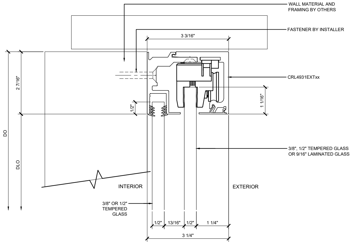
① WALL MOUNT WITH FIXED GLASS CRL6901, CRL6901BSA, CRL6951 & CRL6951BSA HEADER DETAIL ARCH REF: NONE 1'-0"=1'-0"
