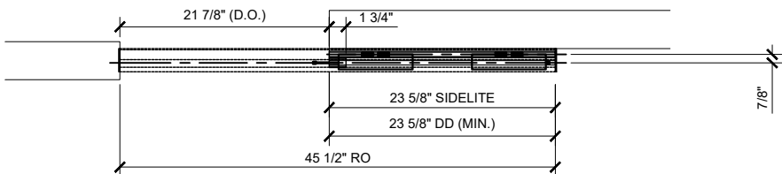
④ CRL6901 PLAN (OPEN POSITION)
