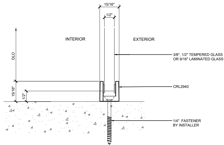
② CRL690, CRL690BSA, CRL695 & CRL695BSA SILL DETAIL
