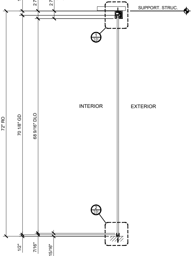
② SLIDER SECTION
