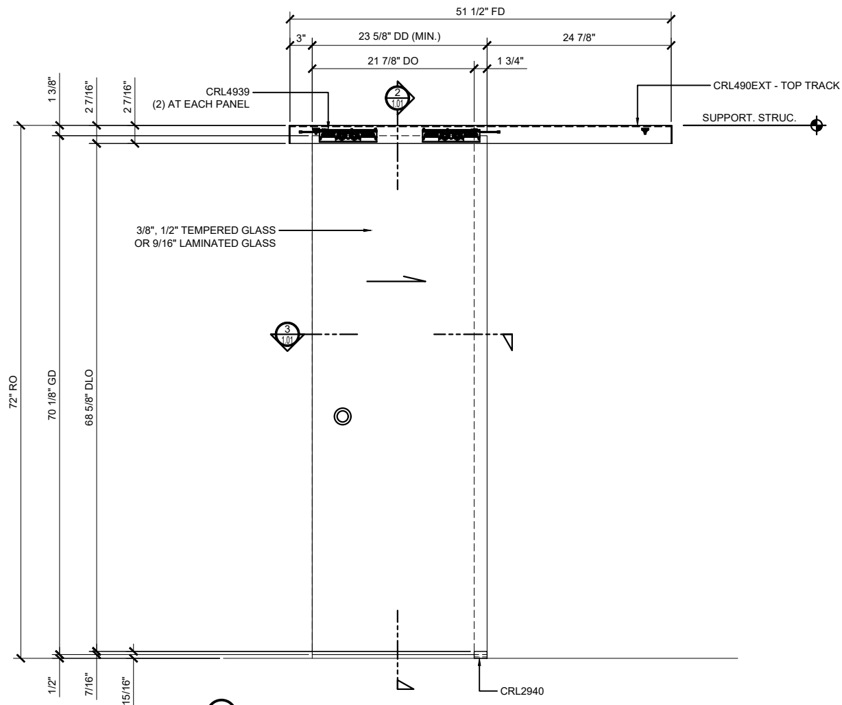
① CRL690 SLIDING DOOR ELEVATION
