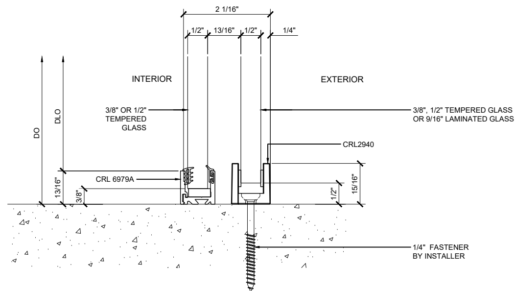
② CRL6901, CRL6901BSA, CRL6951 & CRL6951BSA SILL DETAIL ARCH REF: NONE 1'-0"=1'-0"
