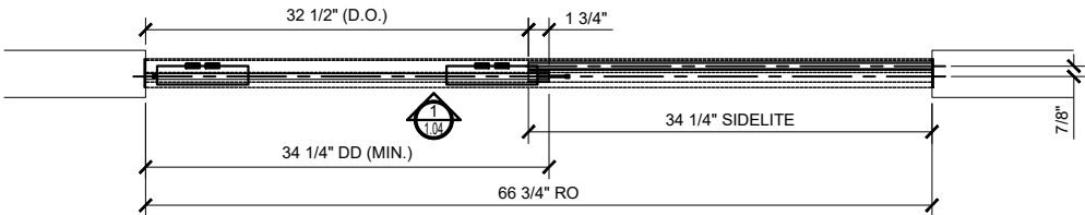
③ CRL6951 PLAN (CLOSED POSITION)
