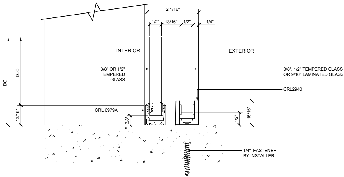
② CRL6901, CRL6901BSA, CRL6951 & CRL6951BSA SILL DETAIL ARCH REF: NONE 1'-0"=1'-0"
