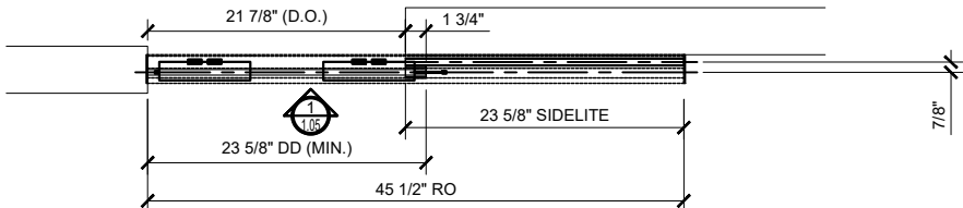
③ CRL6901 PLAN (CLOSED POSITION)
