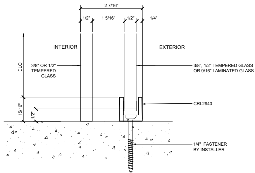
④ CRL6901, CRL6901BSA, CRL6951 & CRL6951BSA SILL DETAIL ARCH REF: NONE 1'-0"=1'-0"
