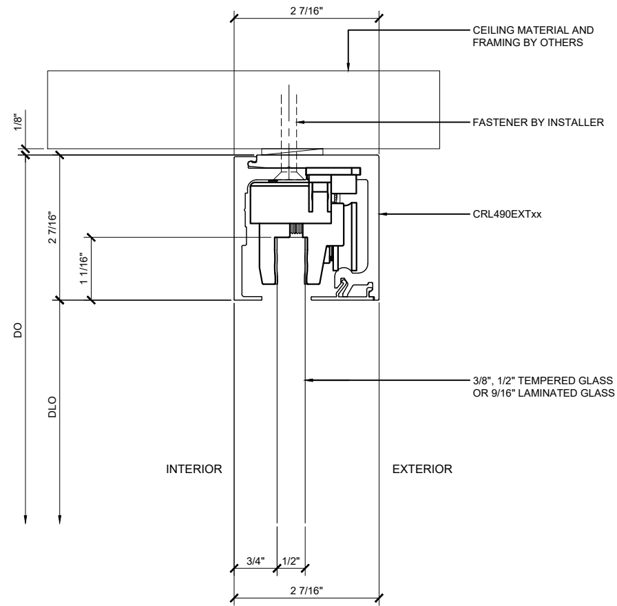
① CEILING MOUNTING CRL690, CRL690BSA, CRL695 & CRL695BSA HEADER DETAIL ARCH REF: NONE 1'-0"=1'-0"
