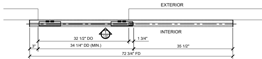
③ CRL695 PLAN (CLOSED POSITION)
