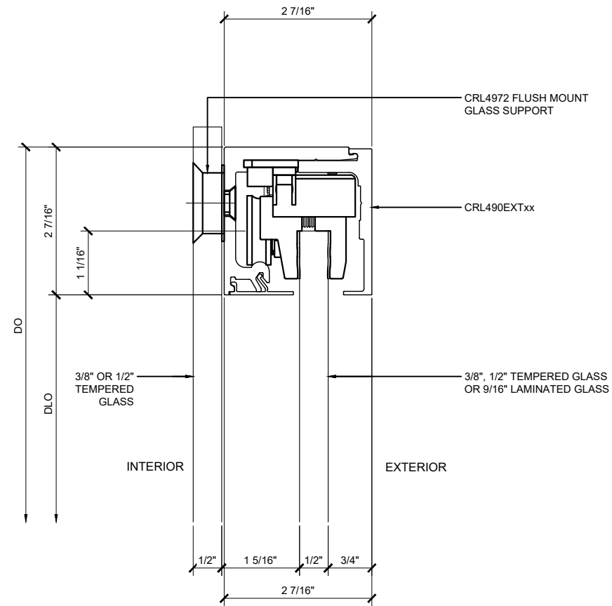
③ GLASS WALL MOUNT CRL6901, CRL6901BSA, CRL6951 & CRL6951BSA HEADER DETAIL ARCH REF: NONE 1'-0"=1'-0"
