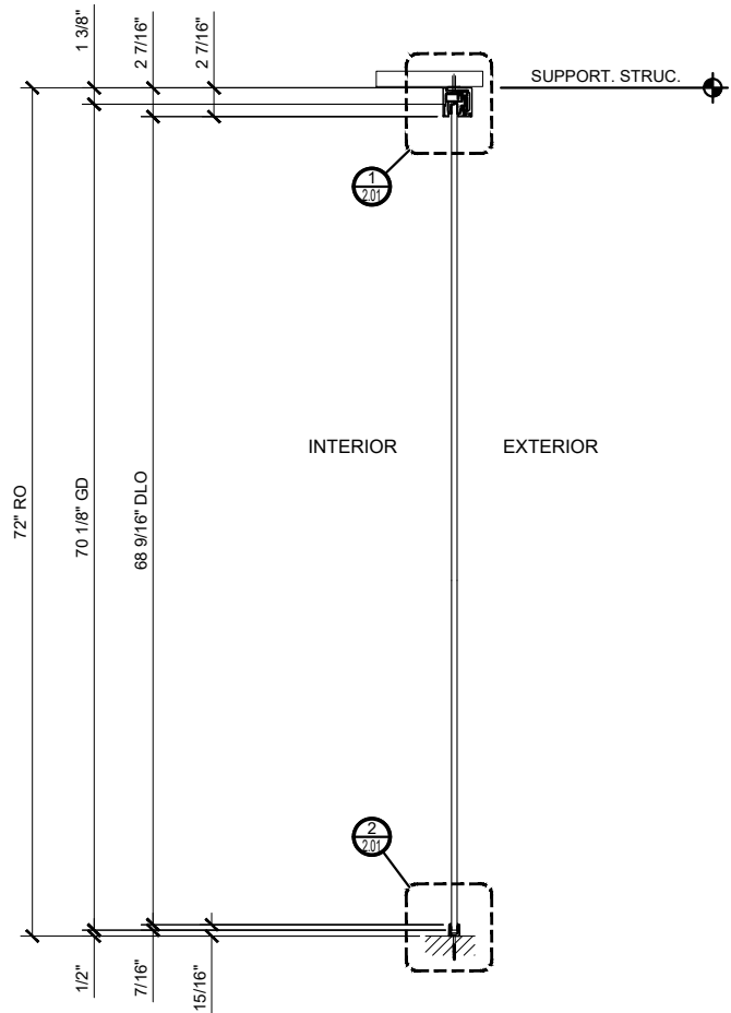
② SLIDER SECTION
