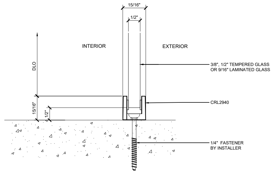
② CRL690, CRL690BSA, CRL695 & CRL695BSA SILL DETAIL ARCH REF: NONE 1'-0"=1'-0"
