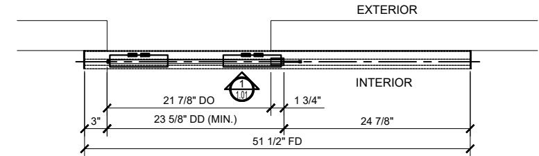
③ CRL690 PLAN (CLOSED POSITION)
