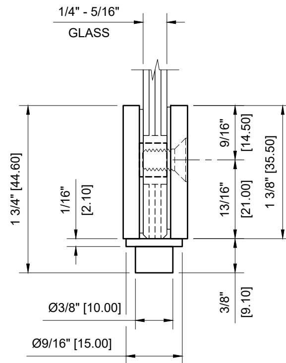
CRL - FA55 FLUSH MOUNT CABINET PIVOT HINGE FOR 1/4" - 5/16" GLASS
