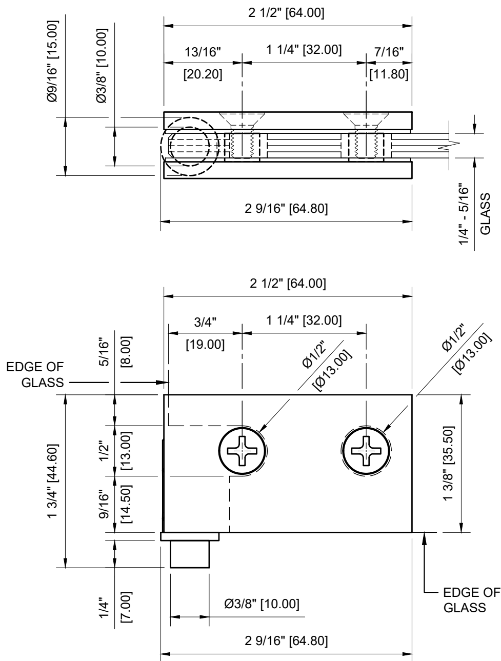
CRL - FA55 FLUSH MOUNT CABINET PIVOT HINGE FOR 1/4" - 5/16" GLASS
