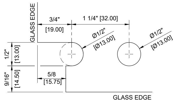
GLASS FABRICATION TEMPLATE
