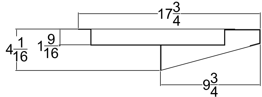
SECTION OUTSIDE SHELF & TRAY
