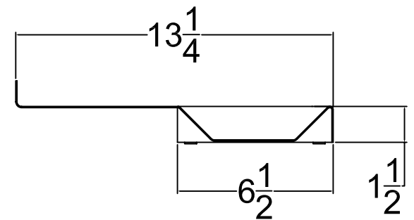
SECTION SLIDING CASH TRAY
