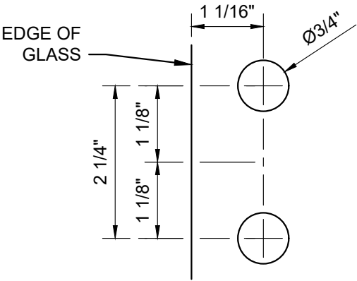
GLASS FABRICATION FIXED PANEL TEMPLATE
