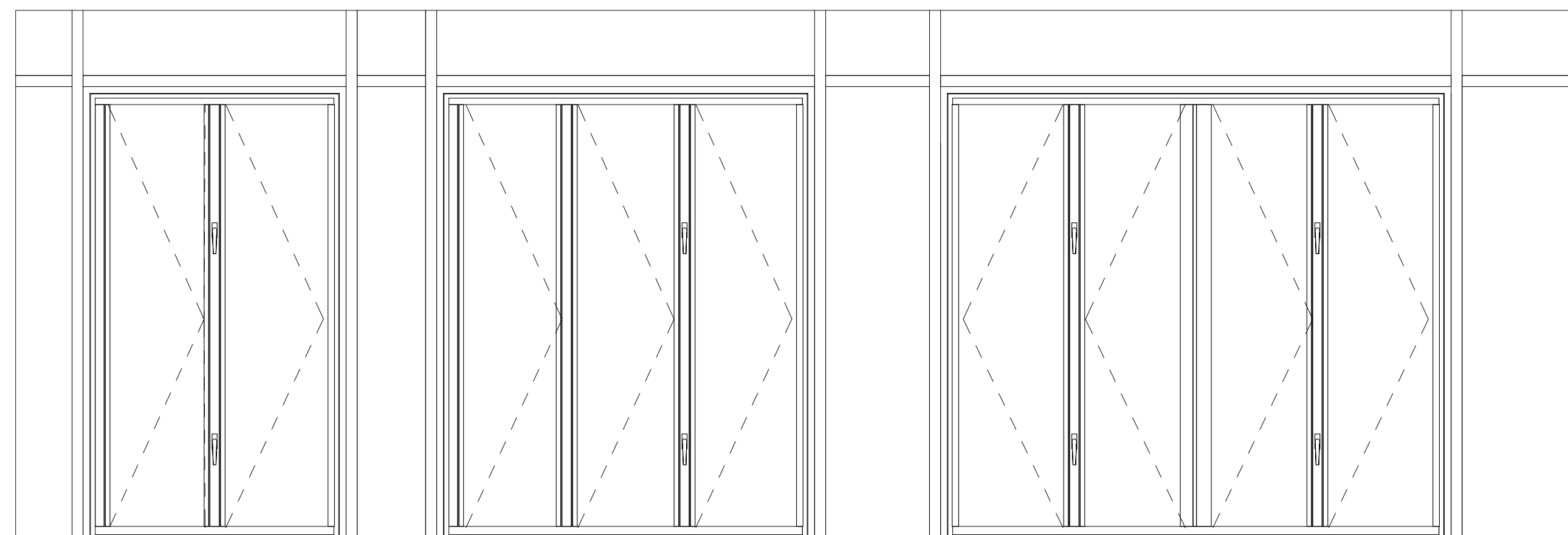
① S90 2, 3, & 4 sample panel configurations 1/2" = 1'-0"
