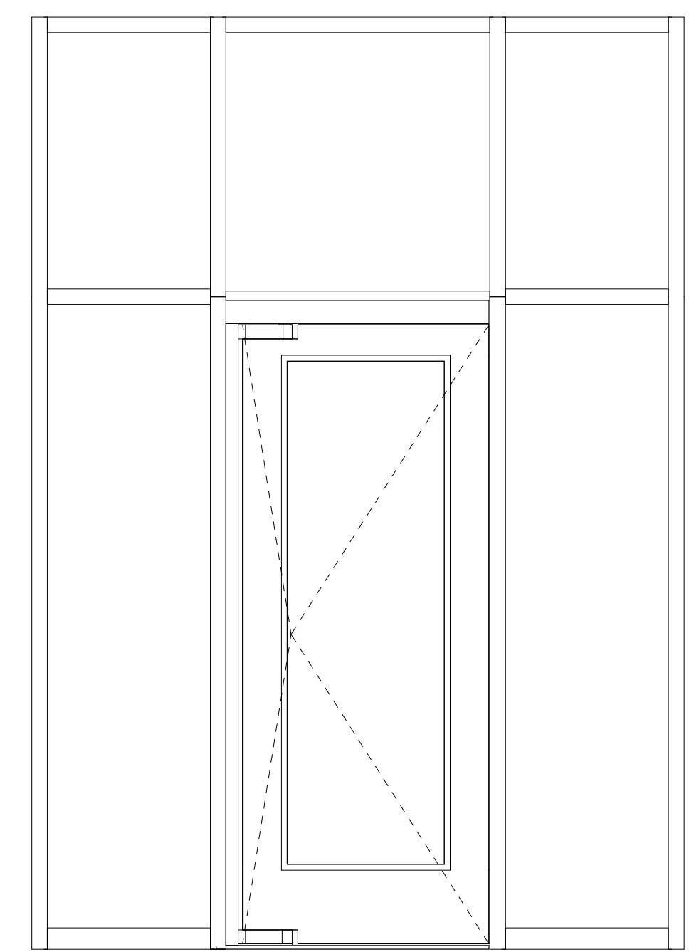
1 Balancer Single Elevation 3/4" = 1'-0"
