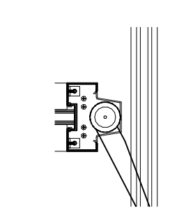
12 Balancer Jamb-Concealed 1 1/2" = 1'-0"
