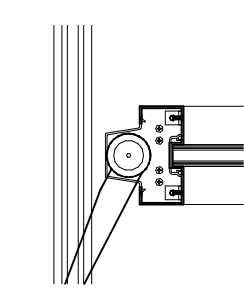
7 Balancer Hinge Jamb 1 1/2" = 1'-0"
