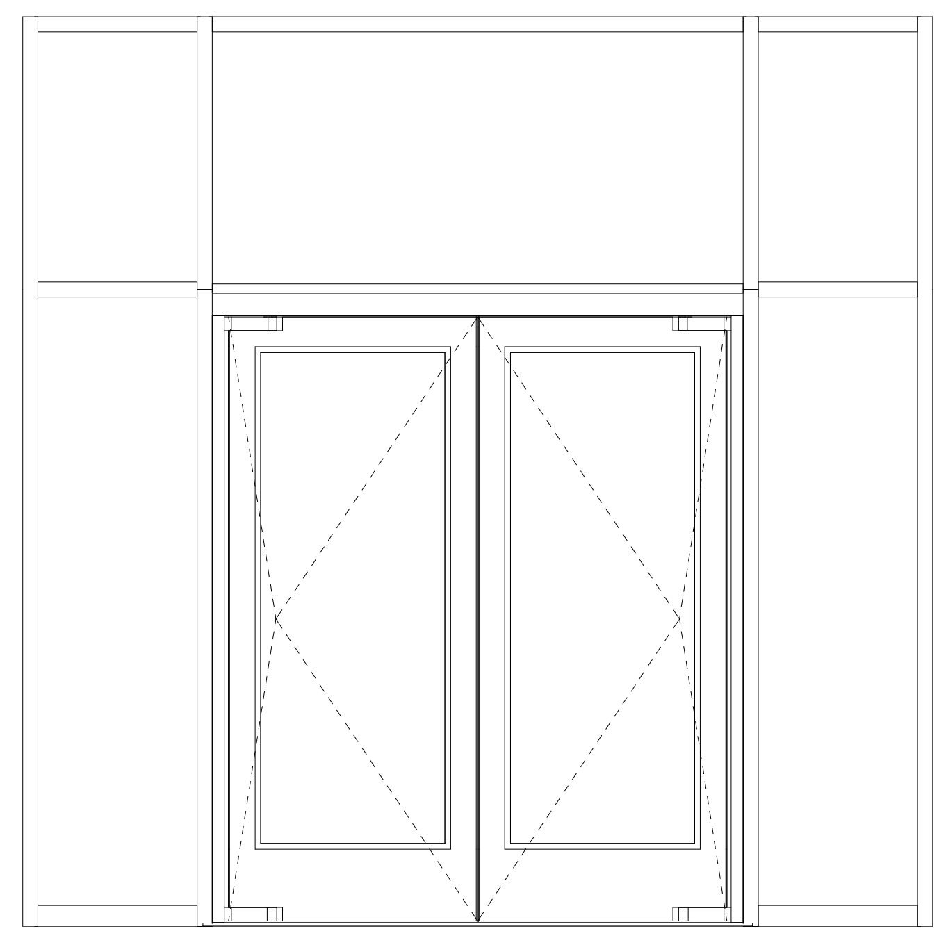
2 Balancer Double Elevation Concealed 3/4" = 1'-0"
