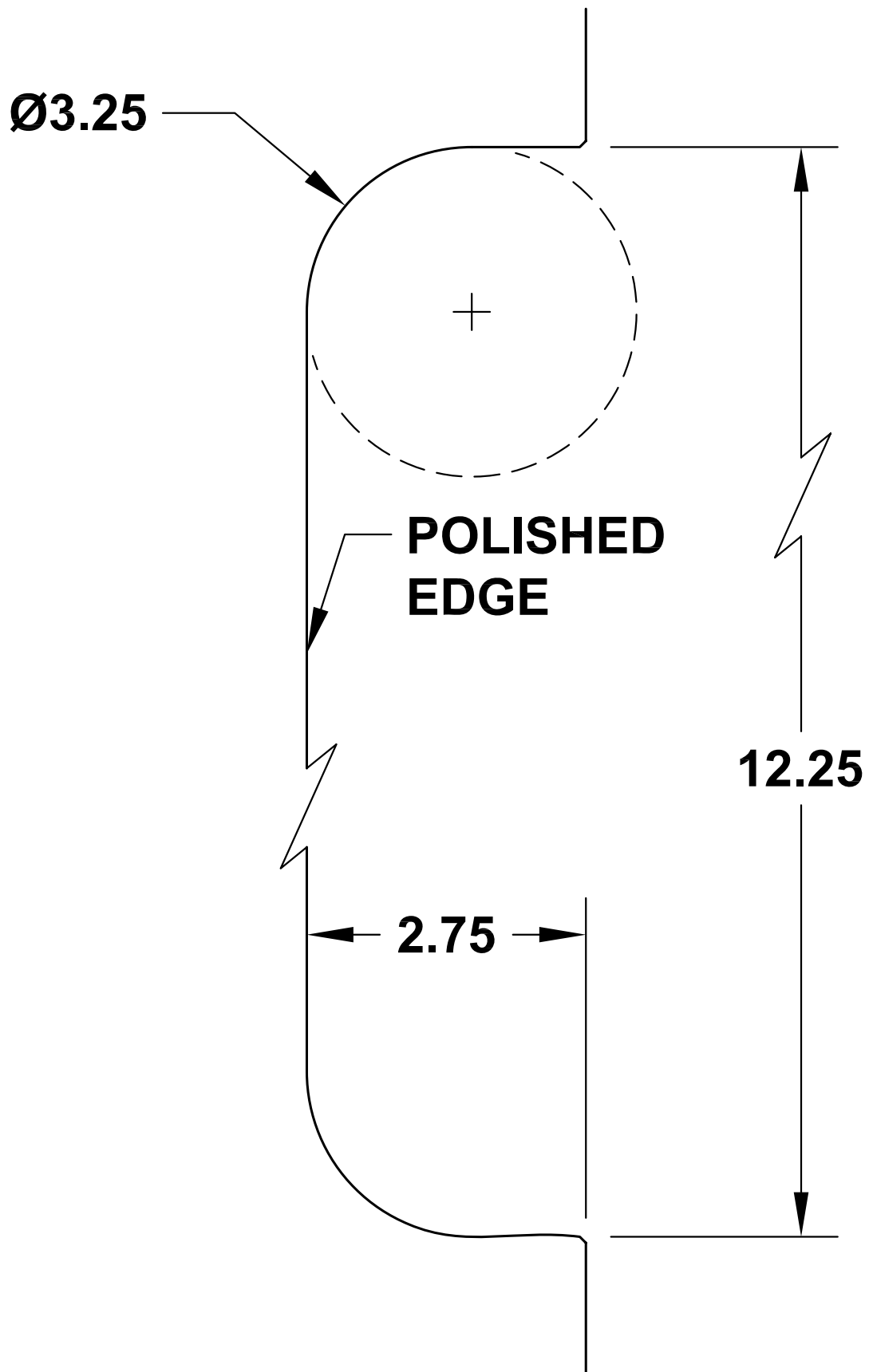
FRAMELESS MAIL SLOT GLASS CUT-OUT TEMPLATE
