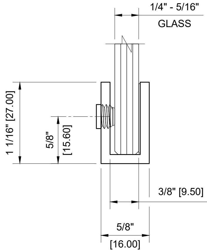
CRL EH35 - BRUSHED NICKEL FINISH DOUBLE SET SCREW GLASS CLAMP
