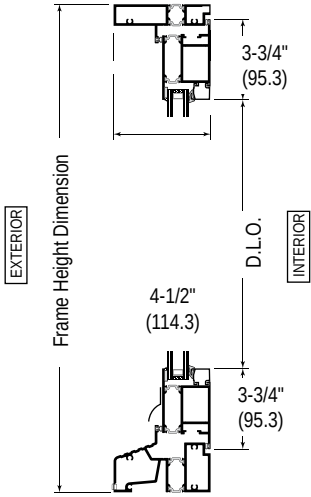
TYPE B STANDARD BOTTOM RAIL AND THRESHOLD SHOWN
