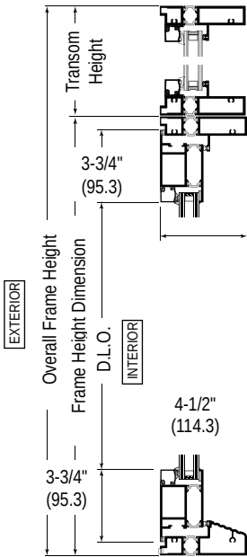
TYPE A STANDARD BOTTOM RAIL AND THRESHOLD SHOWN
