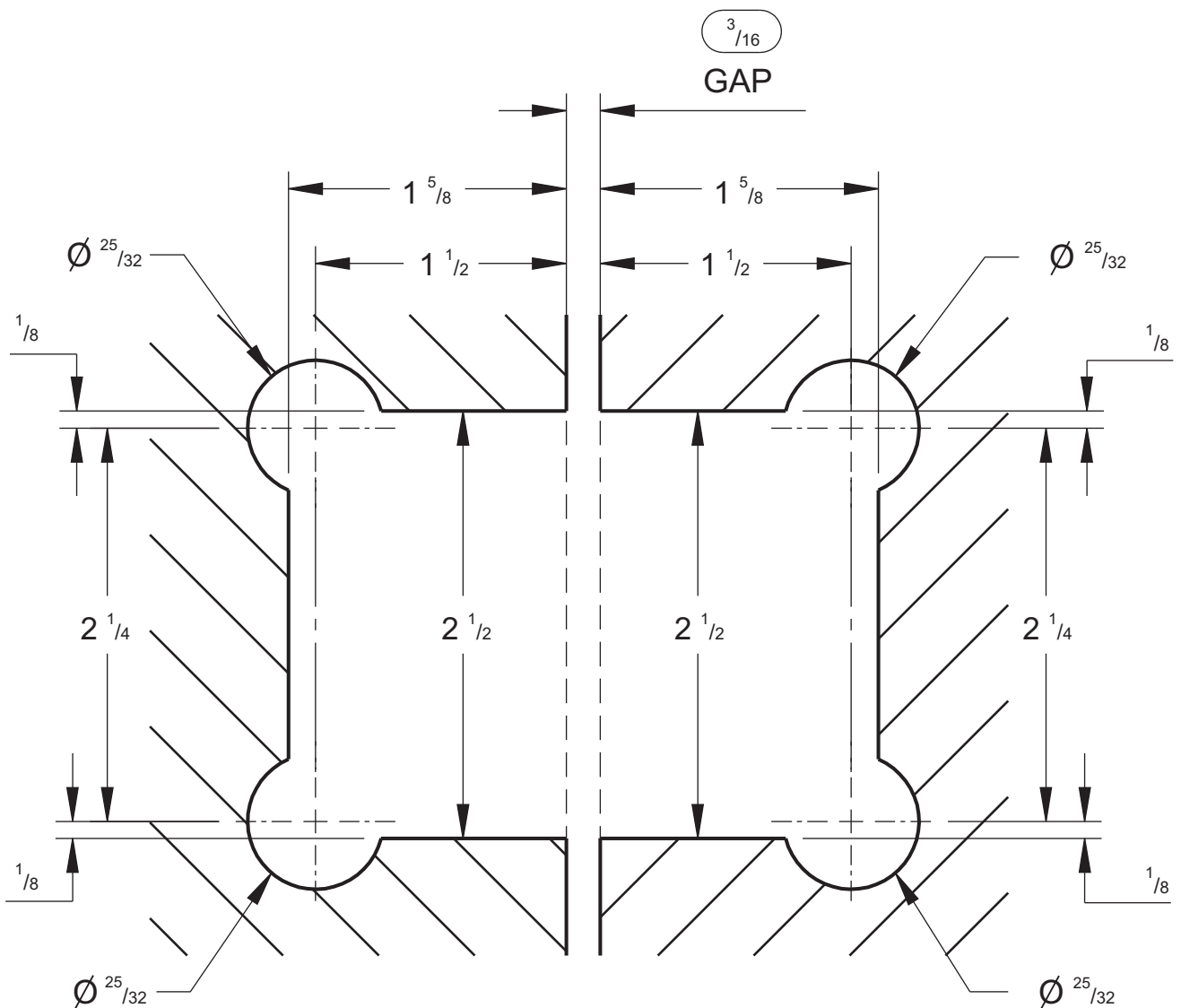
GLASS CUT-OUT TOP AND BOTTOM
