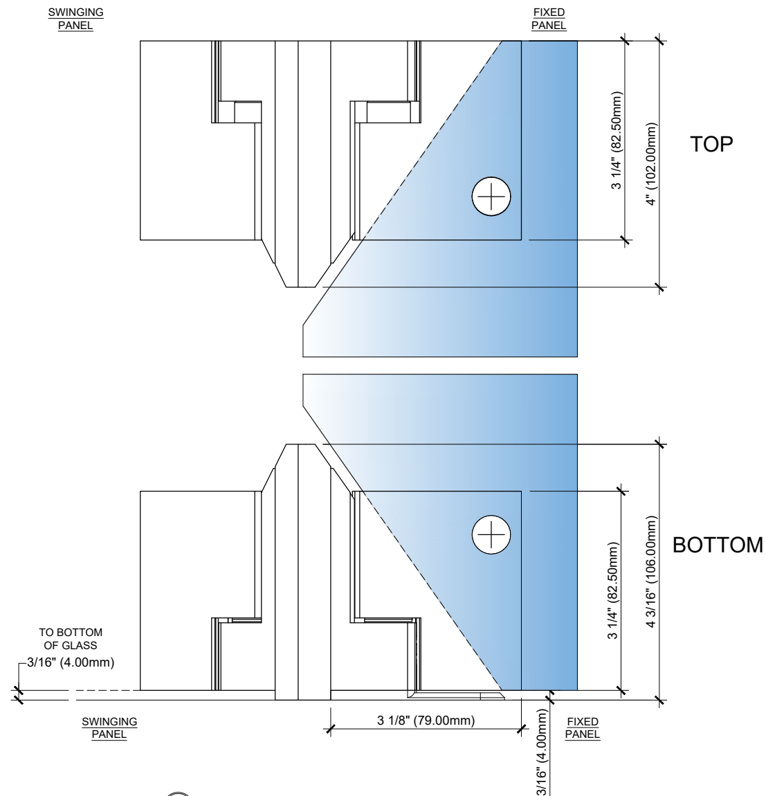
2B FRONT VIEW DETAIL @4MM FIXED PANEL GAP ARCH REF: (SWINGING PANEL GLASS NOT SHOWN) SCALE: 1'-0"=1'-0"
