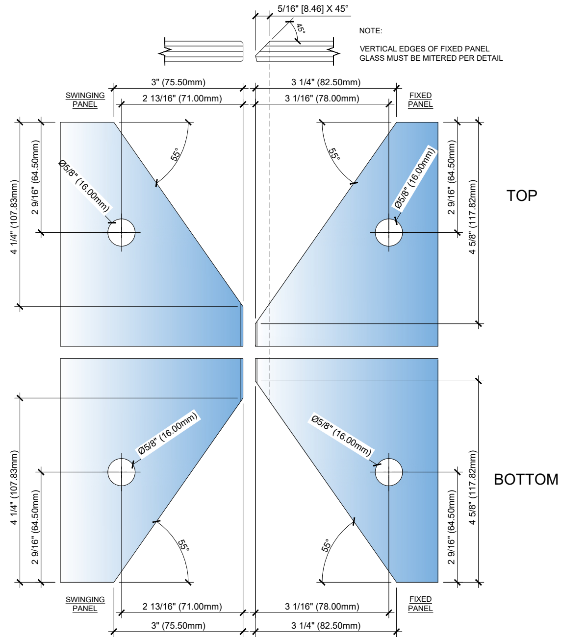
3B GLASS CUT OUT DETAIL - 4MM FIXED PANEL GAP ARCH REF: SCALE: 1'-0"=1'-0"
