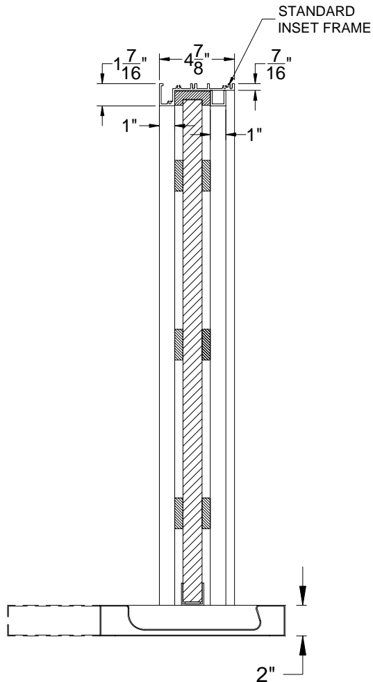
VERTICAL SECTION
