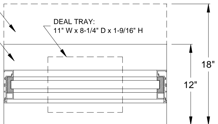
HORIZONTAL SECTION
