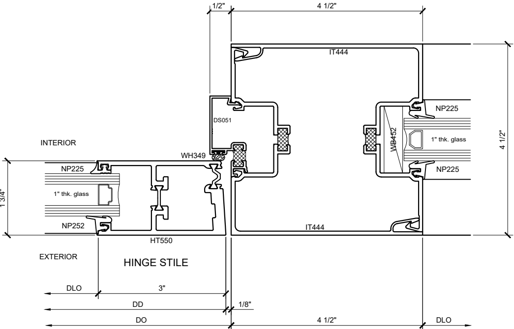
SECTION DETAIL AT WIDE STYLE INTERMEDIATE VERTICAL (20) SCALE: FULL SIZE
