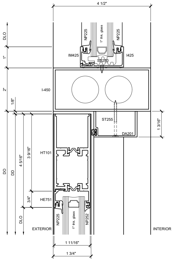
SECTION DETAIL @ 4-5/16" TOP RAIL w/ OHCC ④ SCALE: FULL SIZE
