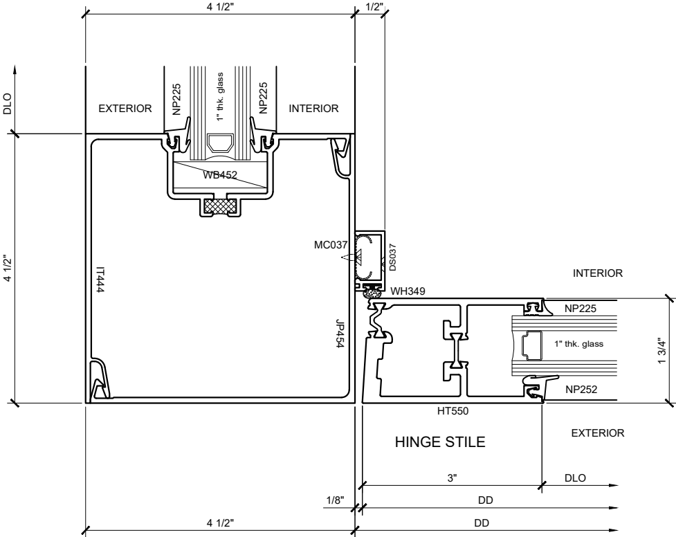
SECTION DETAIL AT WIDE STYLE CORNER VERTICAL (18) SCALE: FULL SIZE
