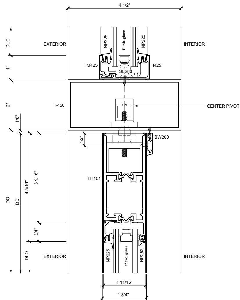
SECTION DETAIL @ 4-5/16" TO RAIL w/ OHCC (25) SCALE: FULL SIZE
