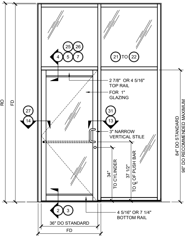
NARROW STILE SERIES 250T DOOR TYP. ELEVATION (SINGLE DOOR @ TRANSOM FRAME ) 3/4" =1'-0"
