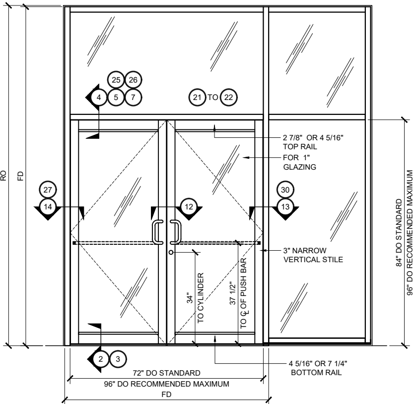
NARROW STILE SERIES 250T DOOR TYP. ELEVATION (DOUBLE DOOR @ TRANSOM FRAME ) 3/4" =1'-0"
