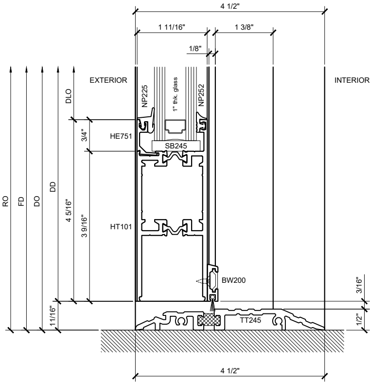
SECTION DETAIL @ 4 5/16" DOOR SILL ③
