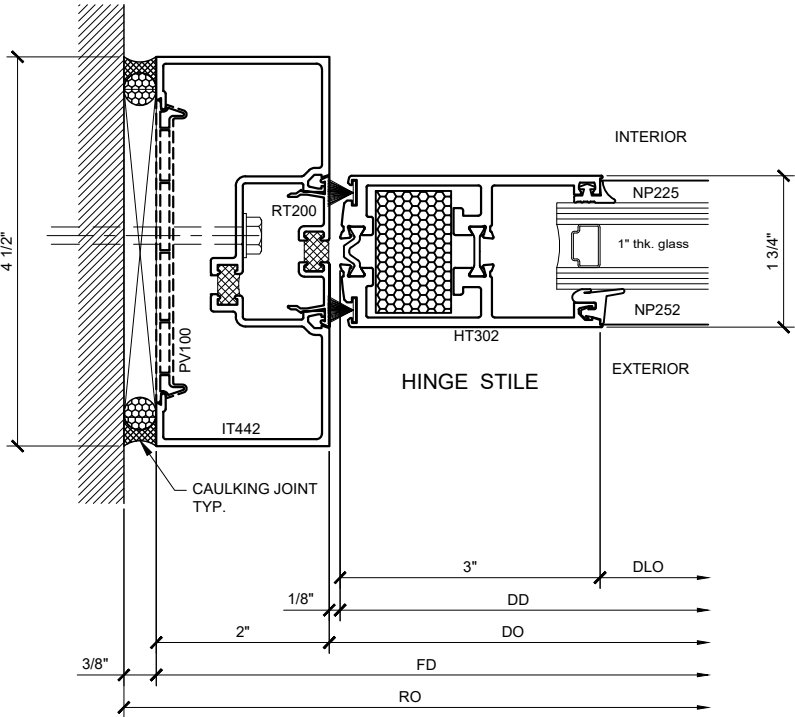
SECTION DETAIL @ DOOR JAMB 27 SCALE: FULL SIZE
