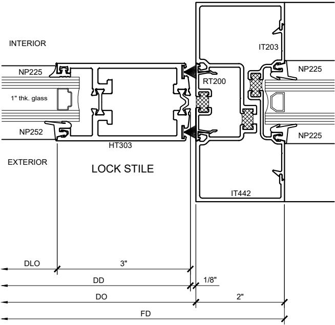
SECTION DETAIL @ DOOR JAMB 31 SCALE: FULL SIZE
