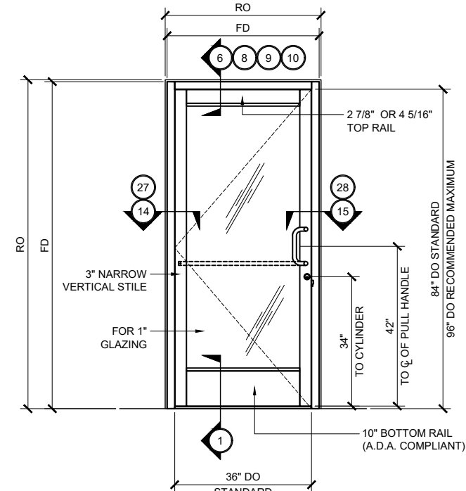
NARROW STILE SERIES 250T DOOR TYP. ELEVATION (SINGLE DOOR @ UP / OVER FRAME ) (SHOWN W/ 10\"/>
