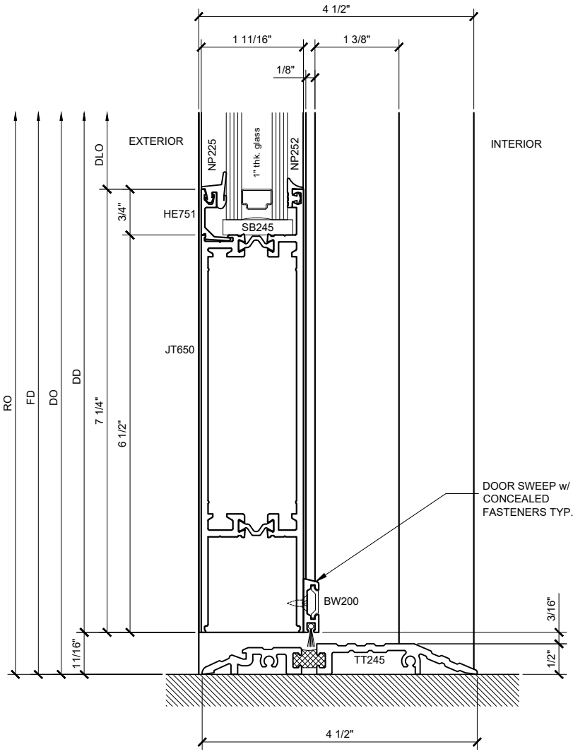
SECTION DETAIL @ 7 1/4" DOOR SILL ②
