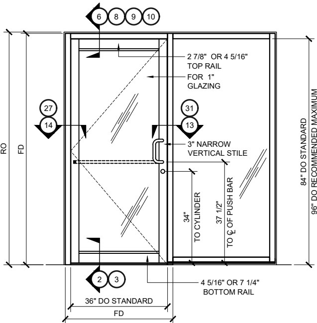
NARROW STILE SERIES 250T DOOR TYP. ELEVATION (SINGLE DOOR @ UP / OVER FRAME WITH SIDELITE) 3/4" =1'-0"
