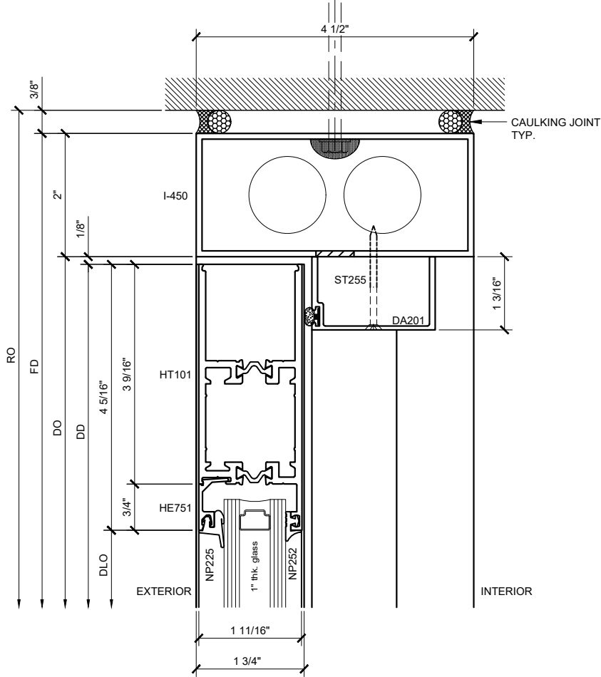
SECTION DETAIL @ 4-5/16" TO RAIL w/ OHCC ⑥ SCALE: FULL SIZE
