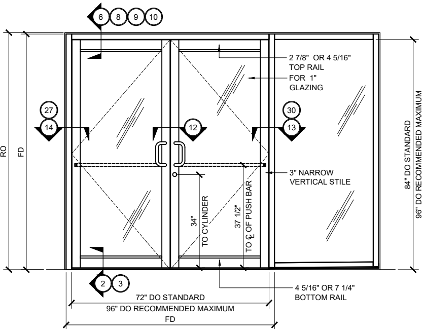
NARROW STILE SERIES 250T DOOR TYP. ELEVATION (DOUBLE DOOR @ UP / OVER FRAME WITH SIDELITE) 3/4" =1'-0"
