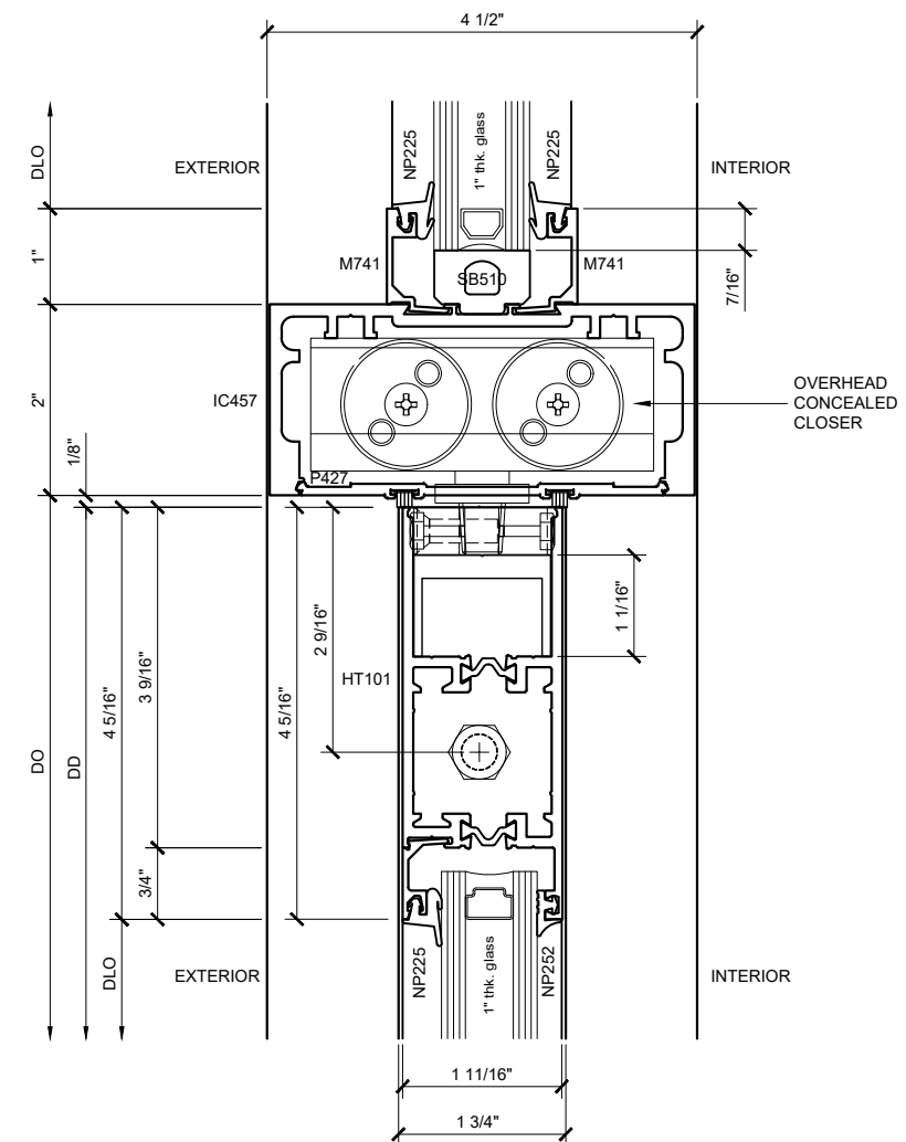
SECTION DETAIL @ 4-5/16" TO RAIL w/ OHCC (26) SCALE: FULL SIZE
