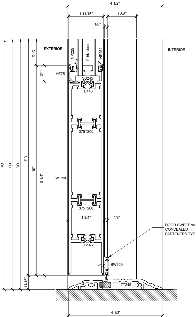
SECTION DETAIL @ 10" DOOR SILL ①
