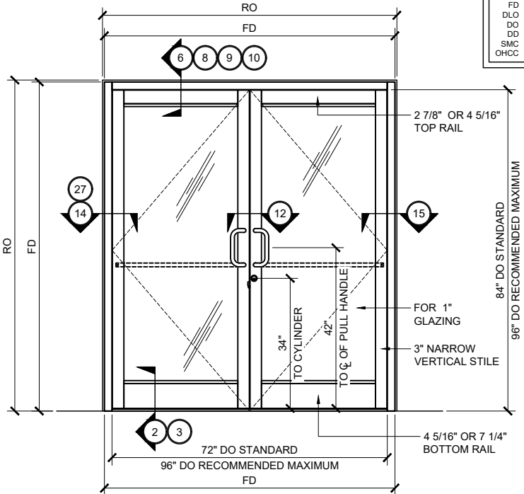
NARROW STILE SERIES 250T DOOR TYP. ELEVATION (DOUBLE DOOR @ UP / OVER FRAME ) 3/4" =1'-0"
