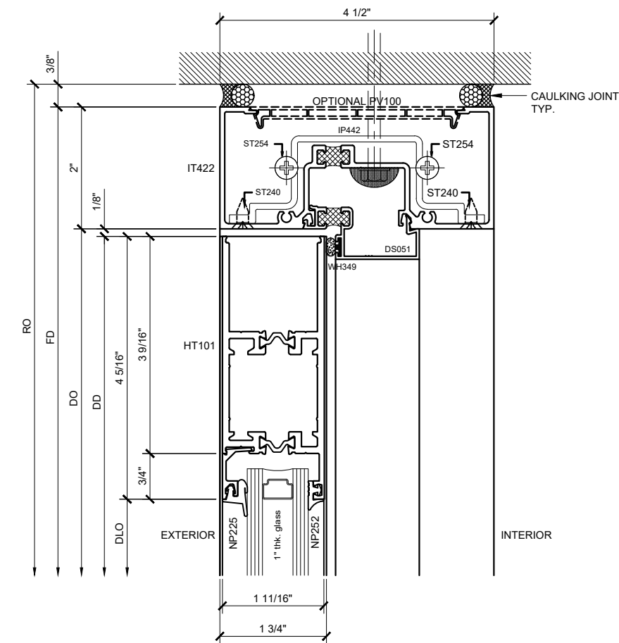
SECTION DETAIL @ 4-5/16" TOP RAIL ⑧ SCALE: FULL SIZE
