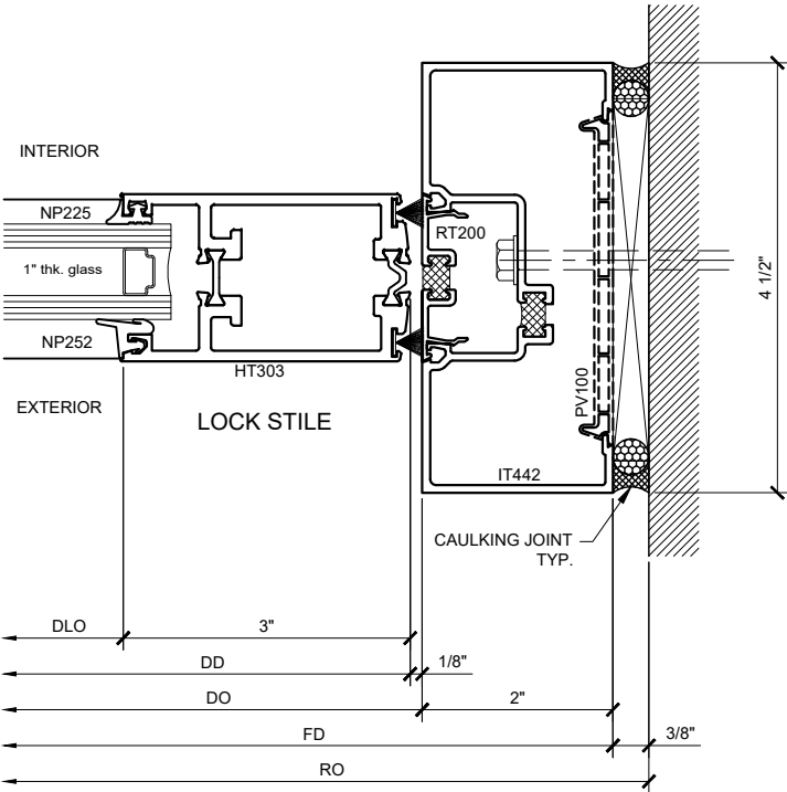
SECTION DETAIL @ DOOR JAMB 28 SCALE: FULL SIZE
