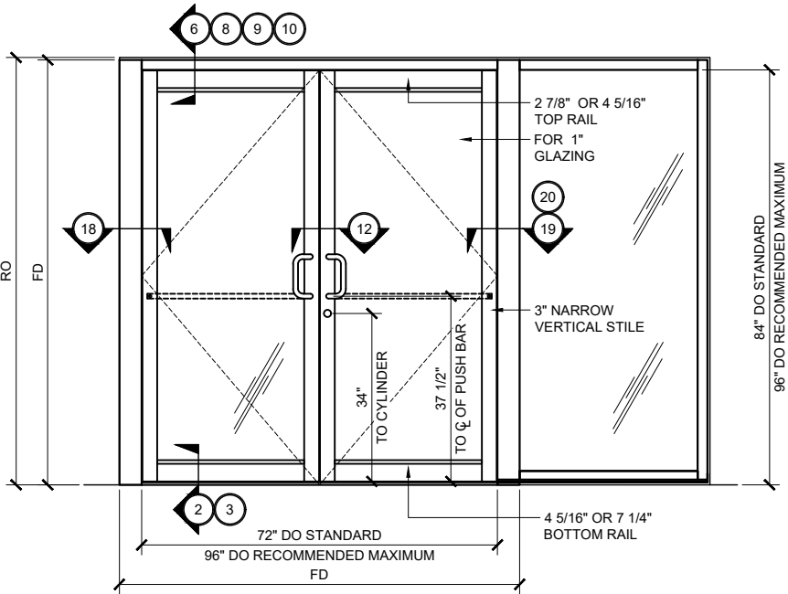
NARROW STILE SERIES 250T DOOR TYP. ELEVATION (DOUBLE DOOR @ UP / OVER FRAME WITH SIDELITE) 3/4" =1'-0"
