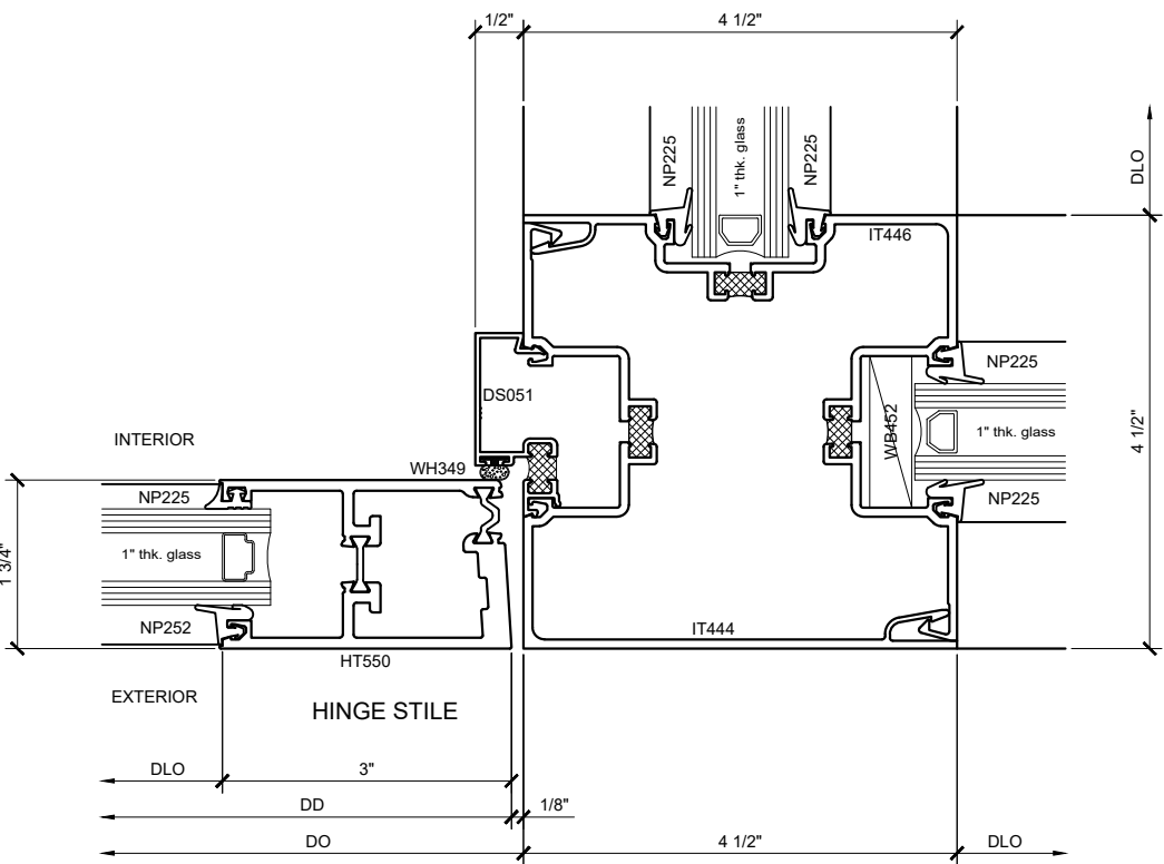
SECTION DETAIL AT WIDE STYLE "T" VERTICAL (19) SCALE: FULL SIZE
