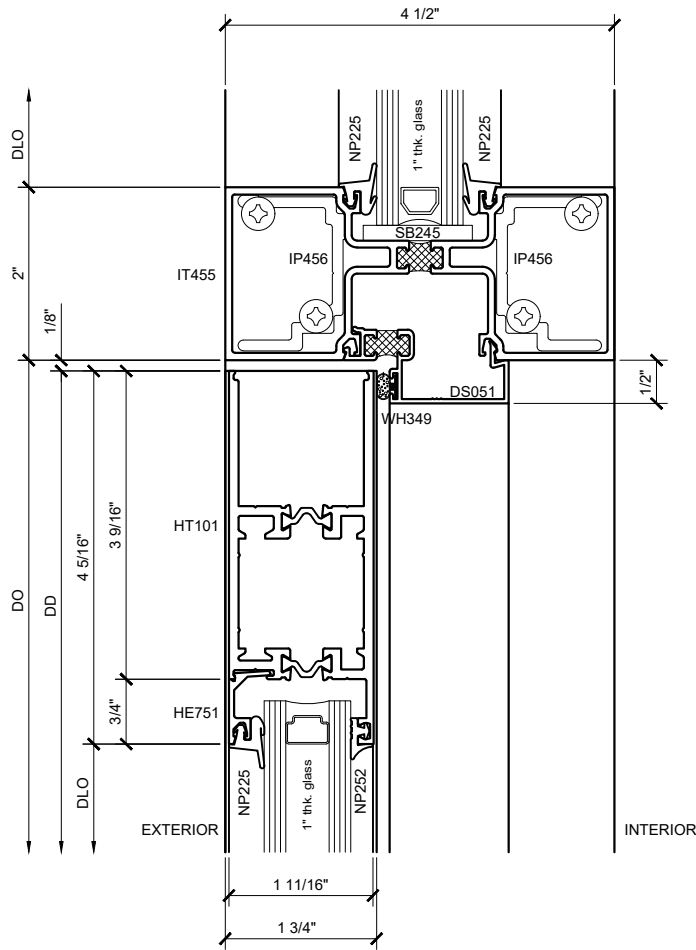
SECTION DETAIL @ 4-5/16" TOP RAIL ⑤ SCALE: FULL SIZE
