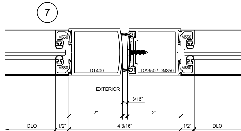
SECTION DETAIL @ MEETING STILES
