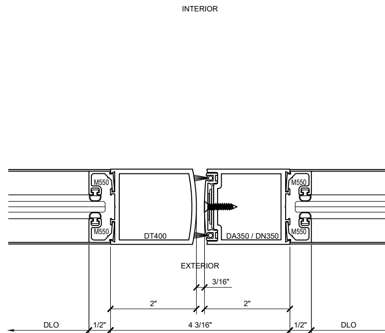
SECTION DETAIL @ MEETING STILES
