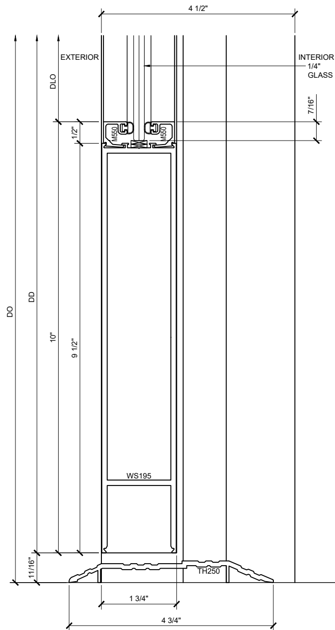
SECTION DETAIL @ ADA DOOR SILL (16) (7 1/2" VERSION IS ALSO AVAILABLE)
