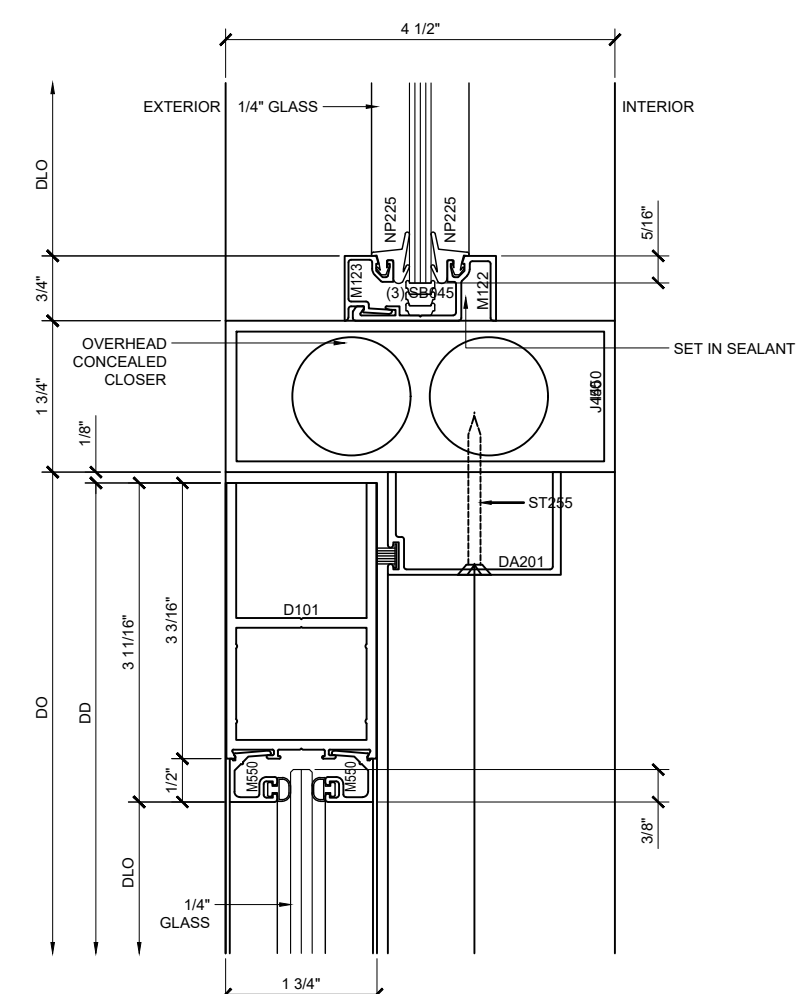
SECTION DETAIL @ DOOR HEAD WITH OHCC 14
