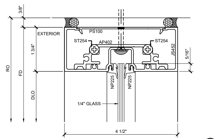
SECTION DETAIL @ STOREFRONT HEAD 12
