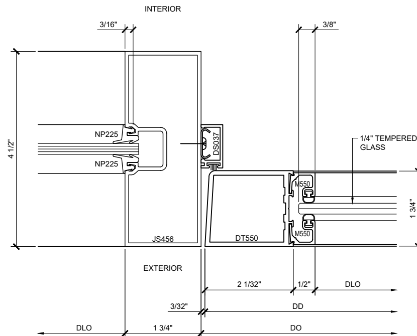
SECTION DETAIL @ MEETING STILES
