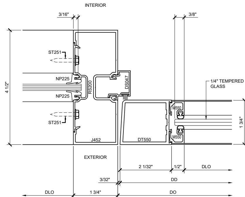
SECTION DETAIL @ DOOR JAMB
