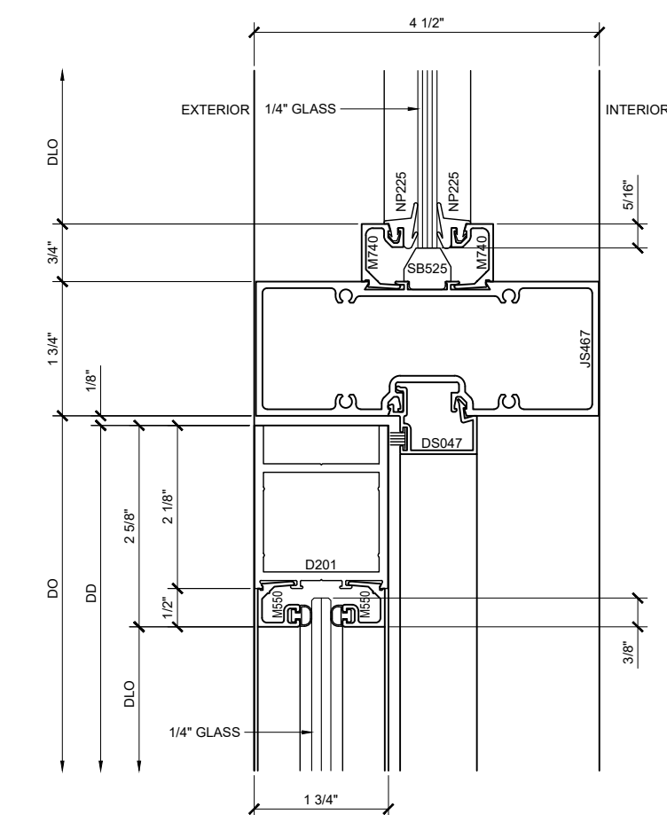
SECTION DETAIL @ DOOR HEAD WITH SMC OR FLOOR CLOSER 13
