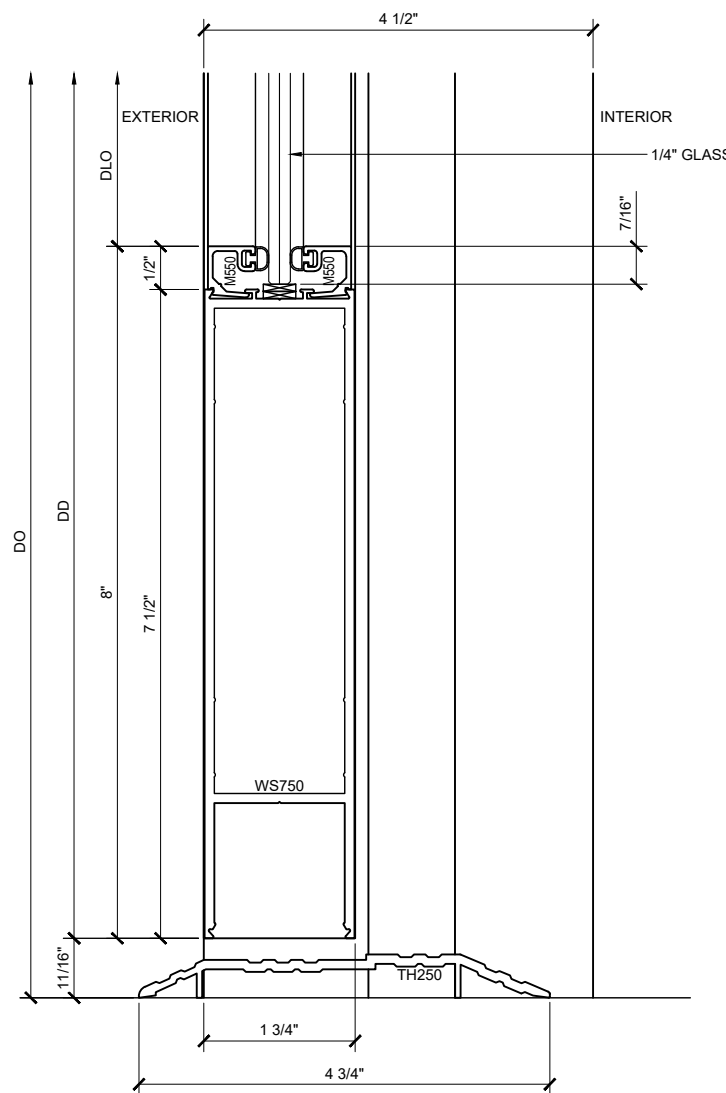
SECTION DETAIL @ DOOR SILL (16A)
