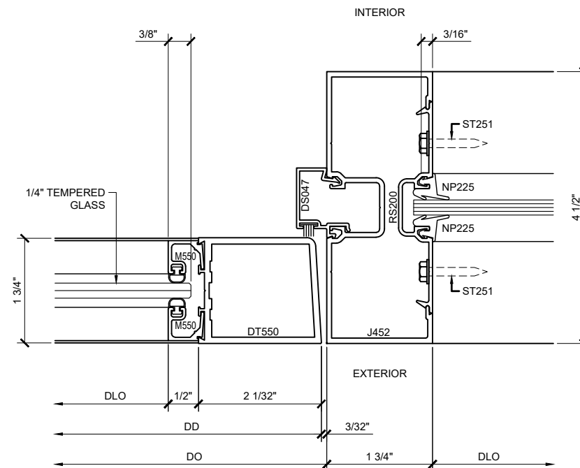
SECTION DETAIL @ DOOR JAMB
