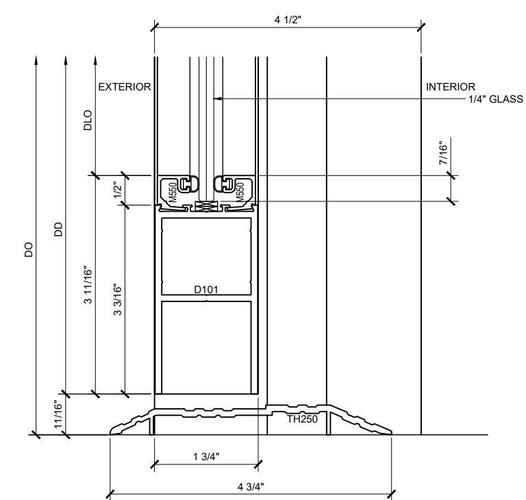
SECTION DETAIL @ DOOR SILL 15
