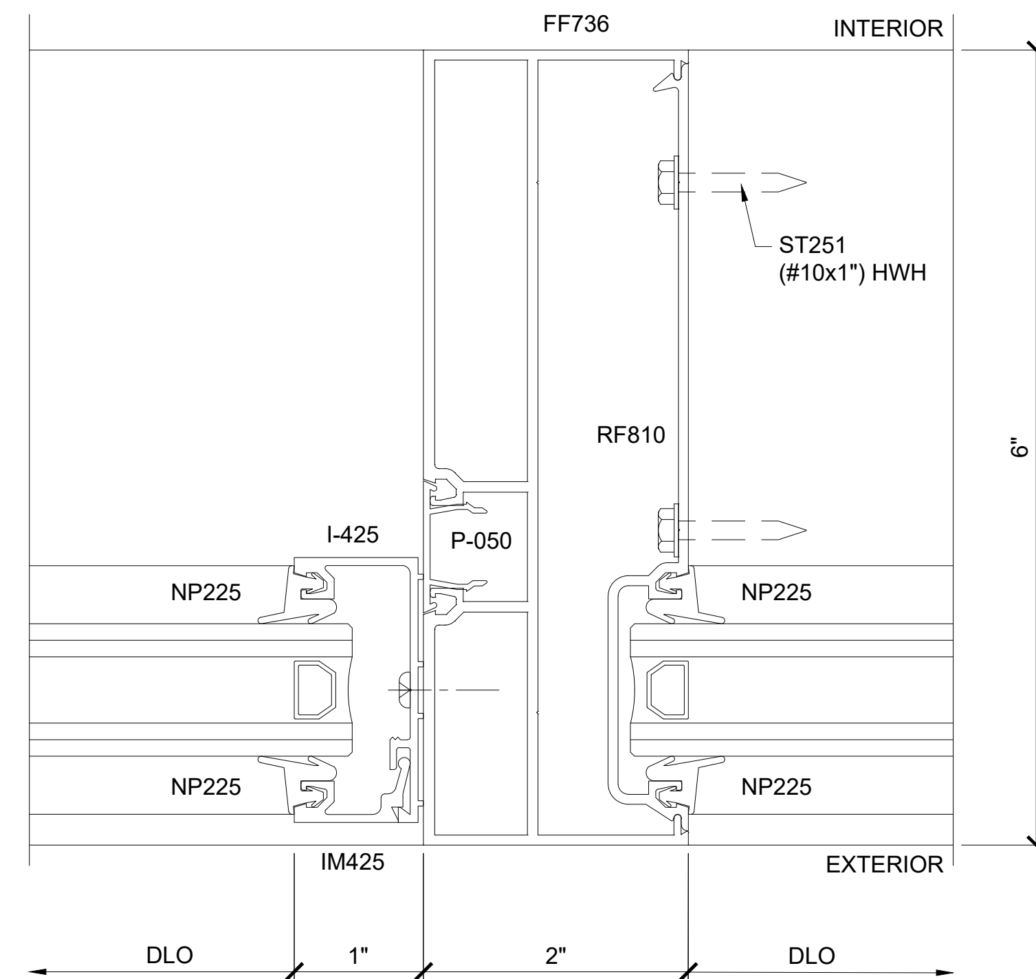
SECTION DETAIL AT INTERMEDIATE VERTICAL
