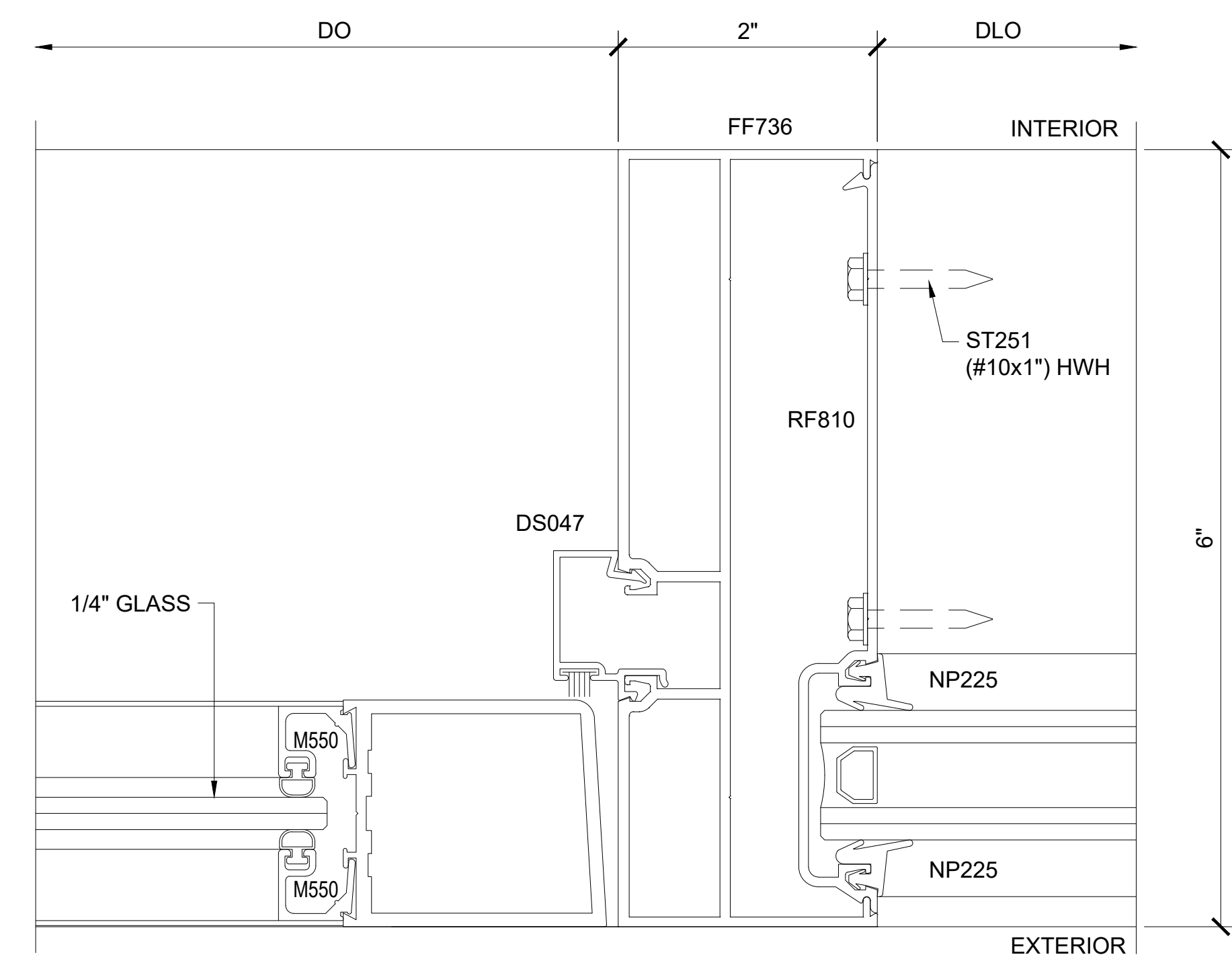
SECTION DETAIL AT DOOR INTERMEDIATE VERTICAL ④
