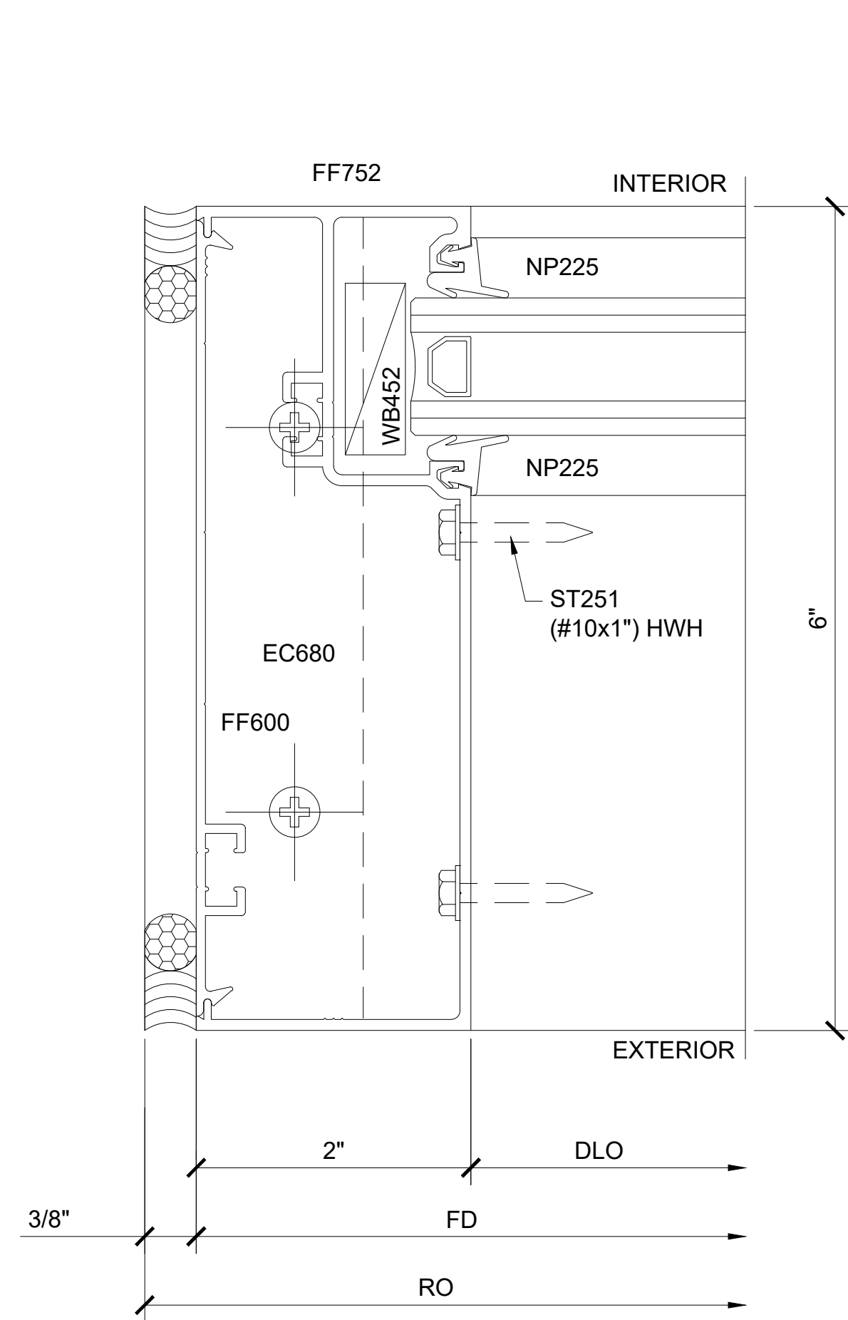
SECTION DETAIL AT JAMB 8
