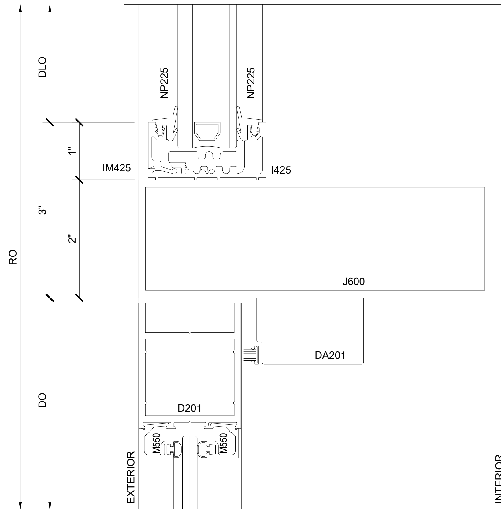
SECTION DETAIL AT DOOR HEADER 8
