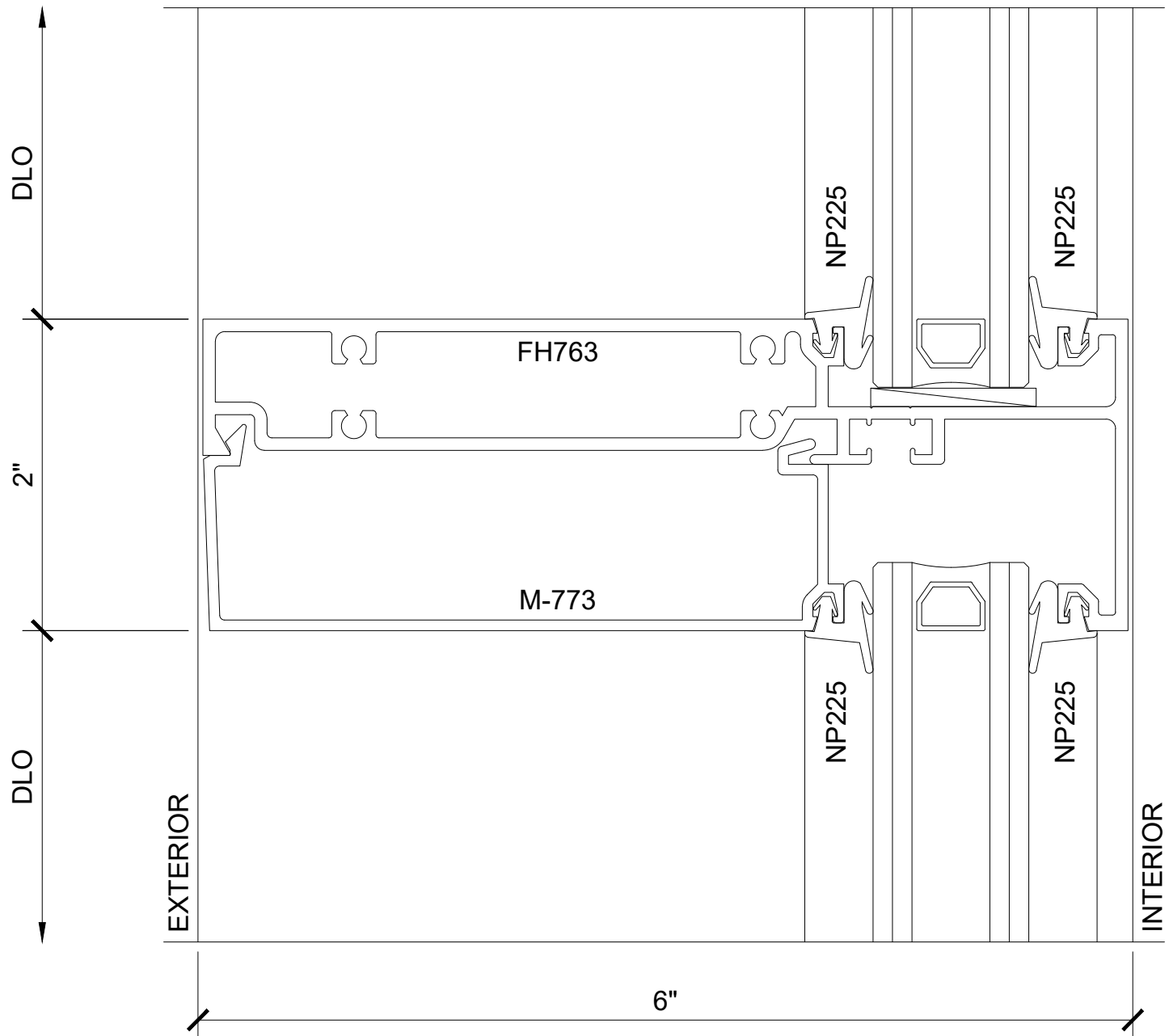
SECTION DETAIL AT INTERMEDIATE HORIZONTAL 13
