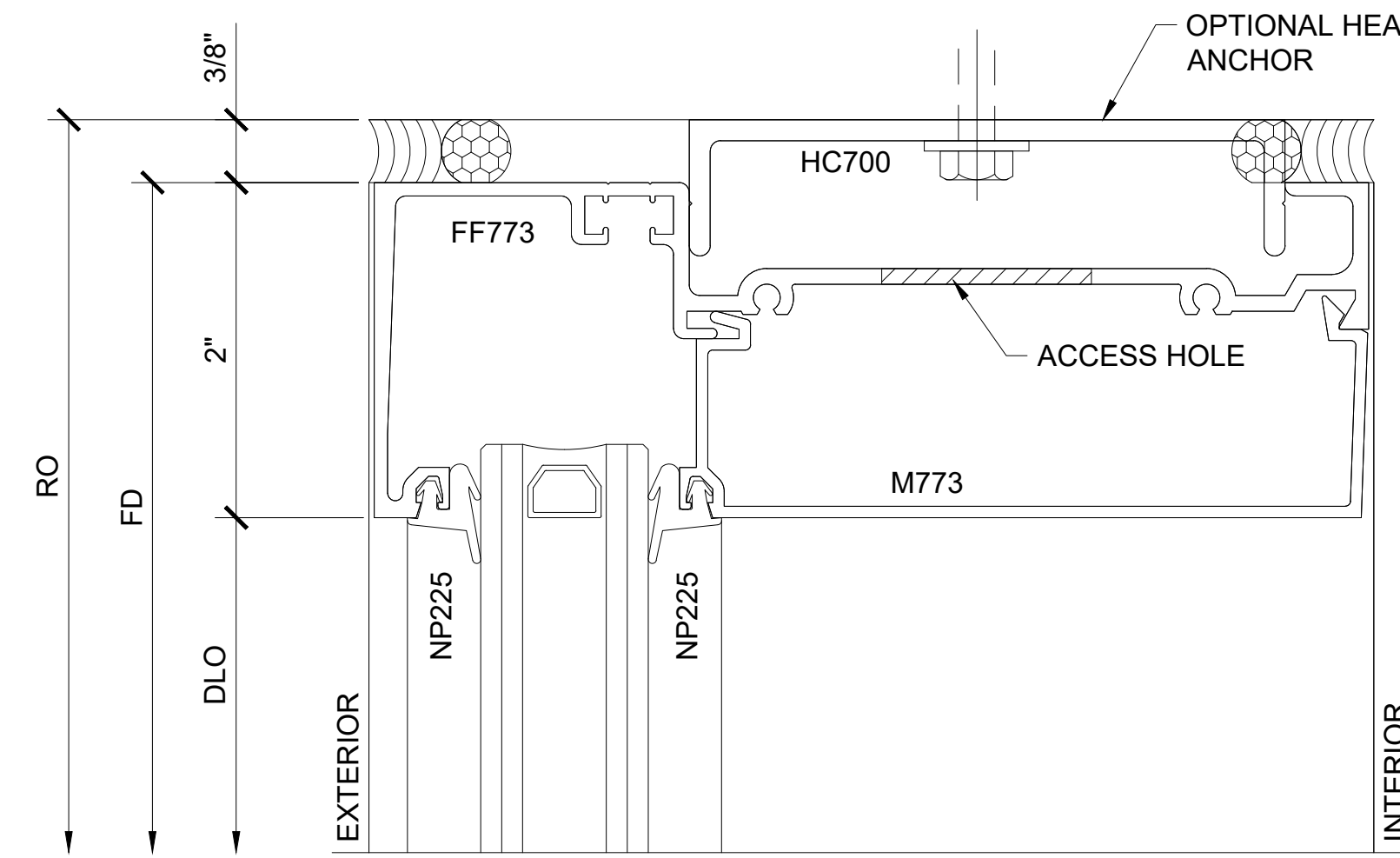
SECTION DETAIL AT HEAD WITH ANCHOR
