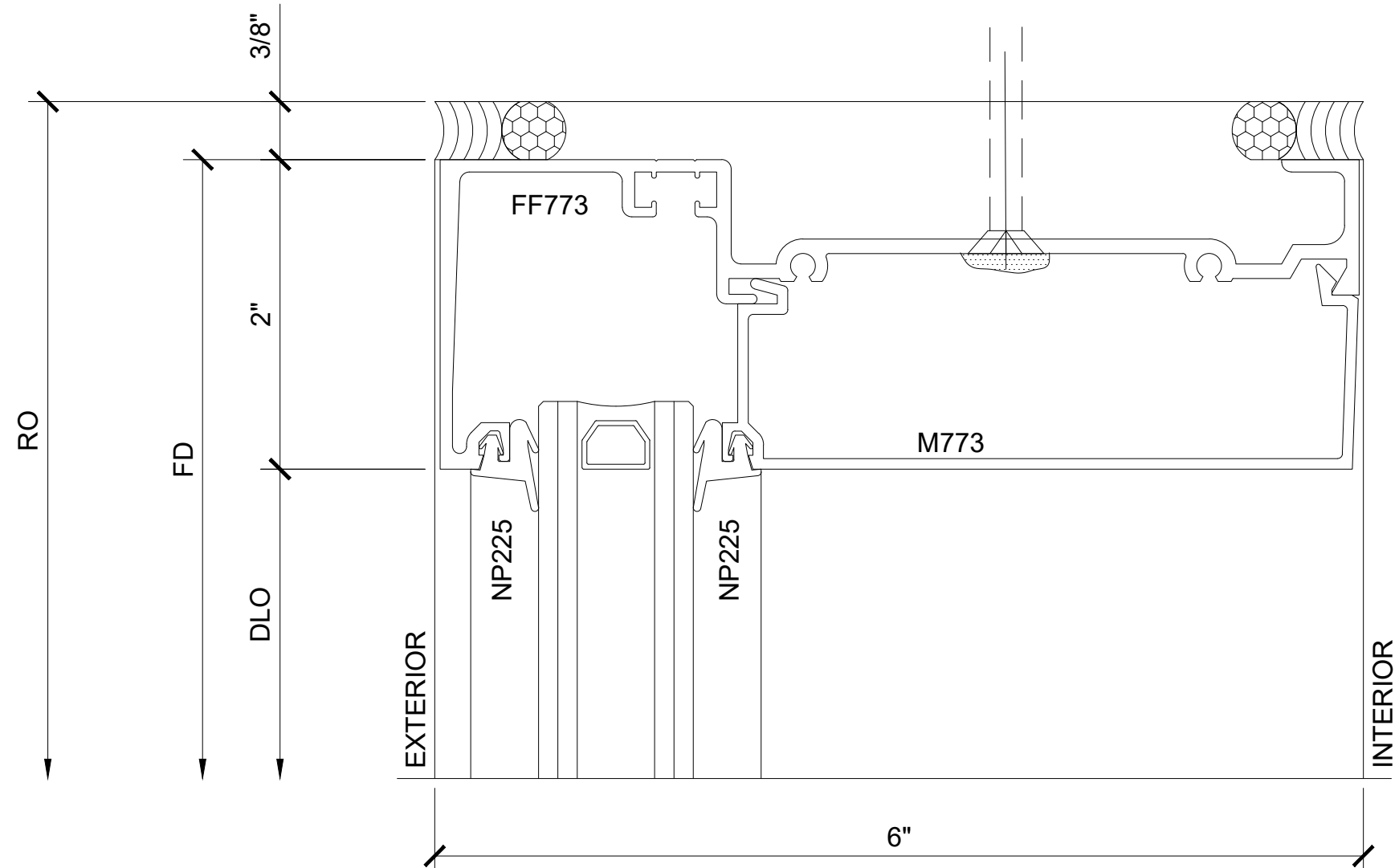
SECTION DETAIL AT HEAD 9
