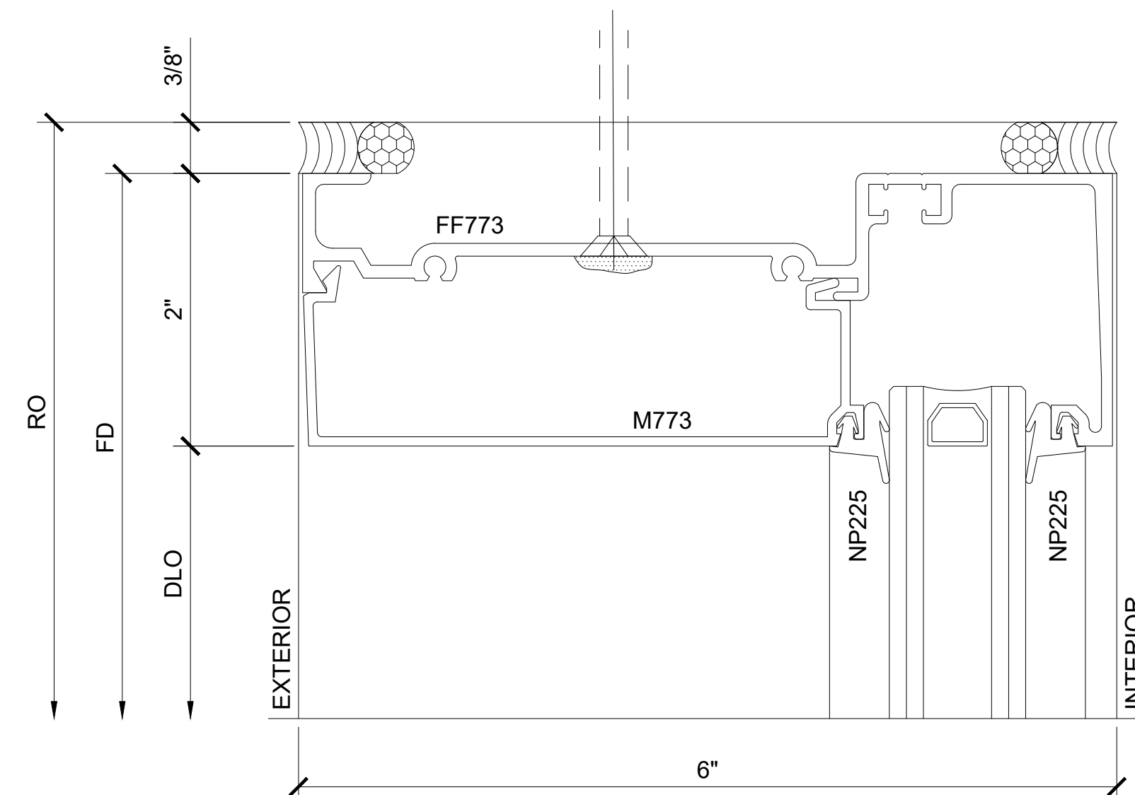
SECTION DETAIL AT HEAD
