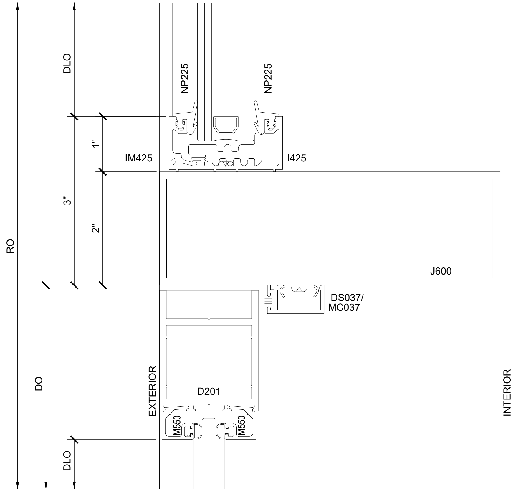
SECTION DETAIL AT DOOR HEADER 10
