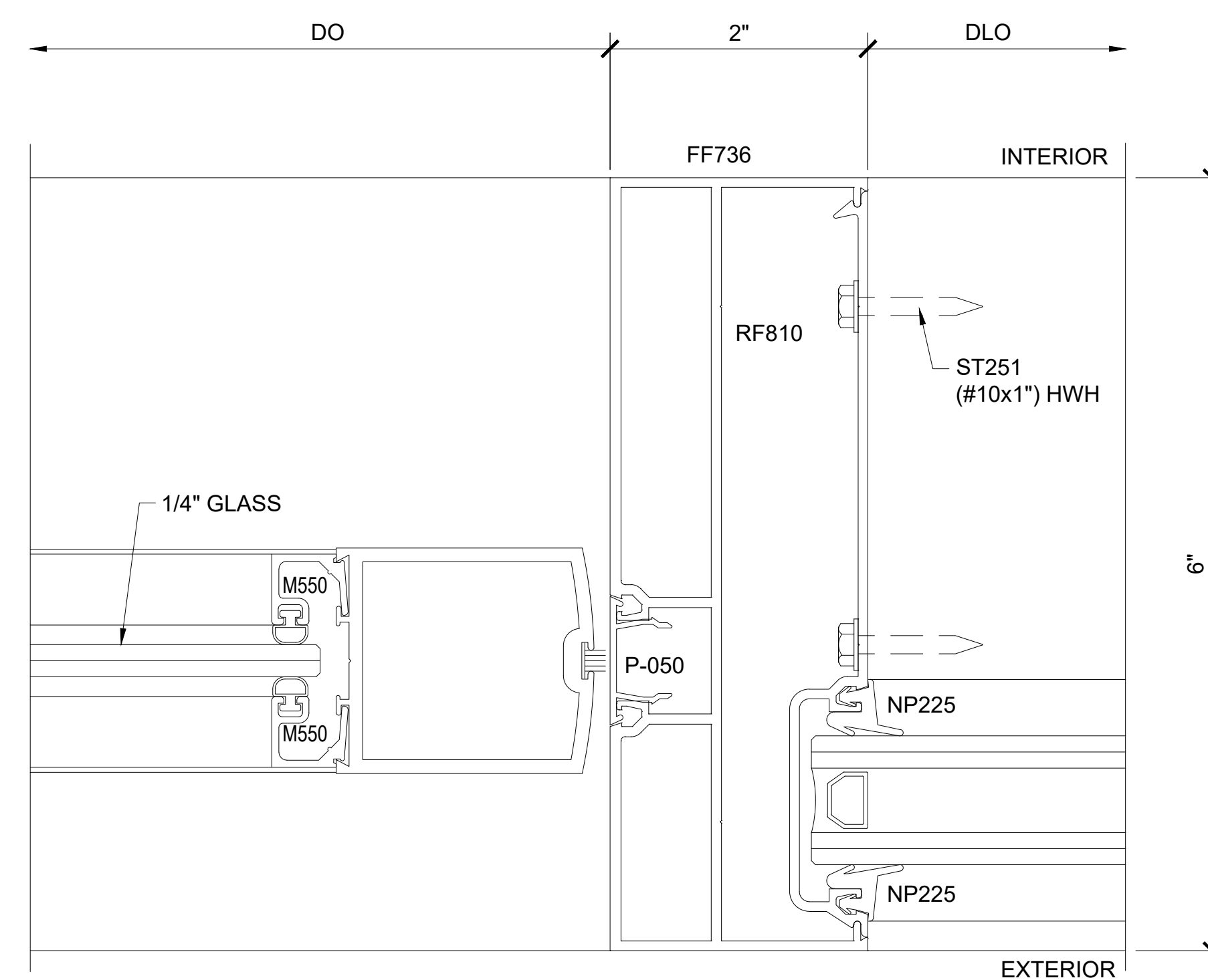
SECTION DETAIL AT DOOR INTERMEDIATE VERTICAL
