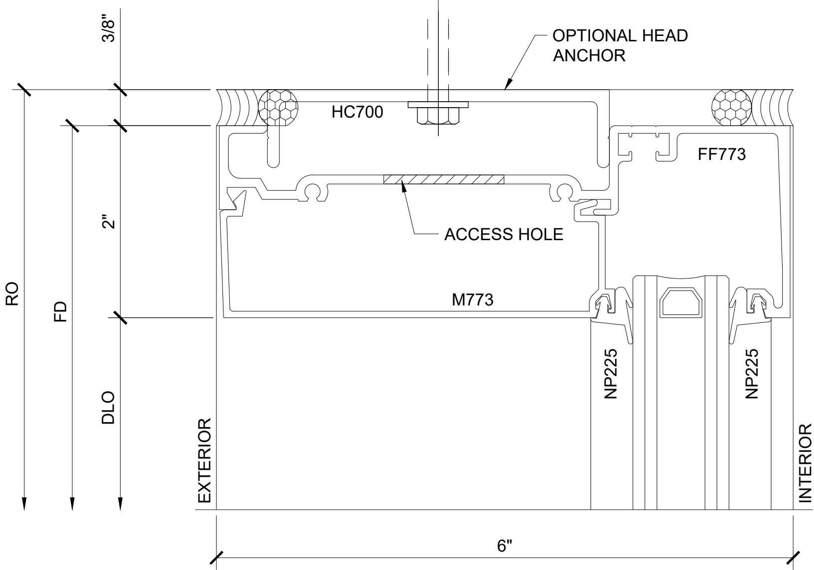
SECTION DETAIL AT HEAD W/ ANCHOR 11
