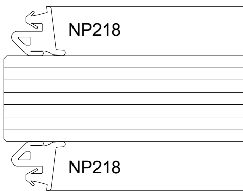
SECTION DETAIL AT FF601 - 7/8" GLASS 7
