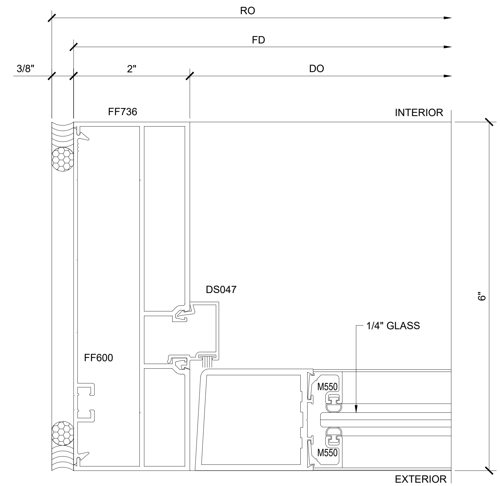
SECTION DETAIL AT DOOR JAMB ②
