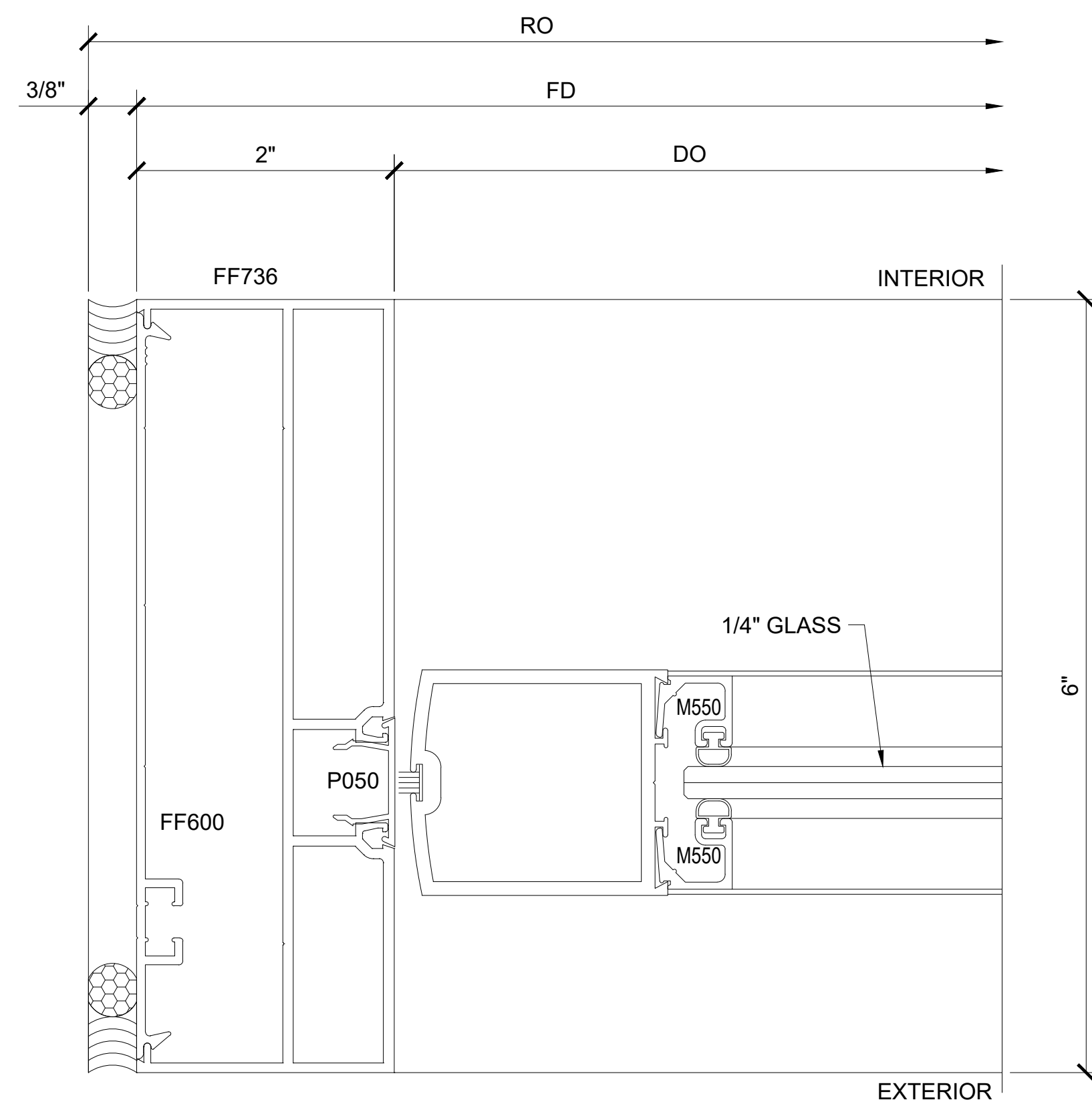
SECTION DETAIL AT DOOR JAMB
