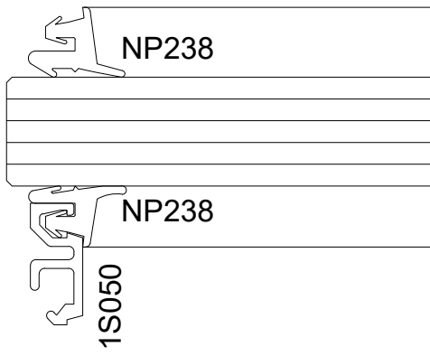
SECTION DETAIL AT FF601 - 5/8" GLASS 6
