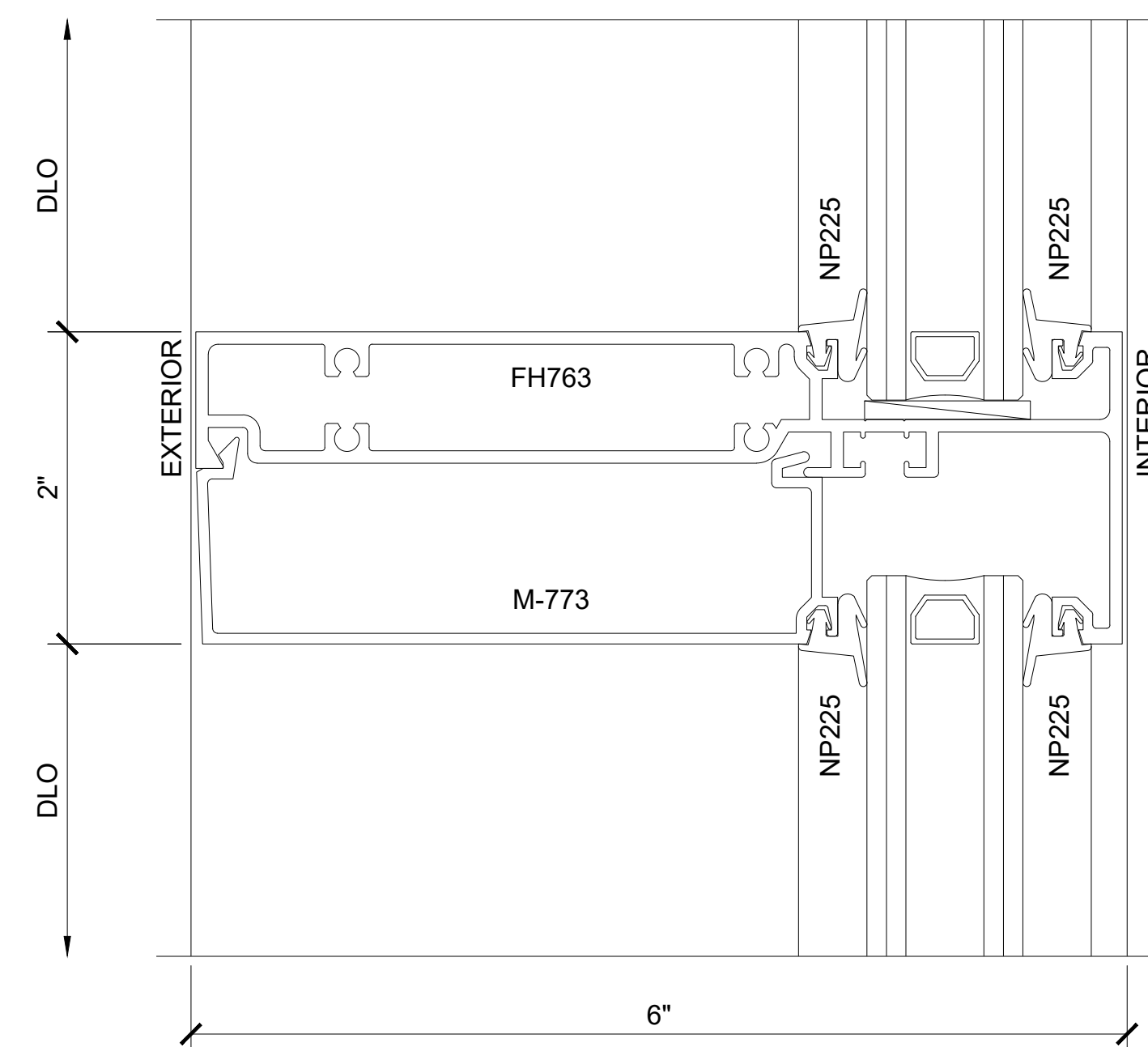
SECTION DETAIL AT INTERMEDIATE HORIZONTAL
