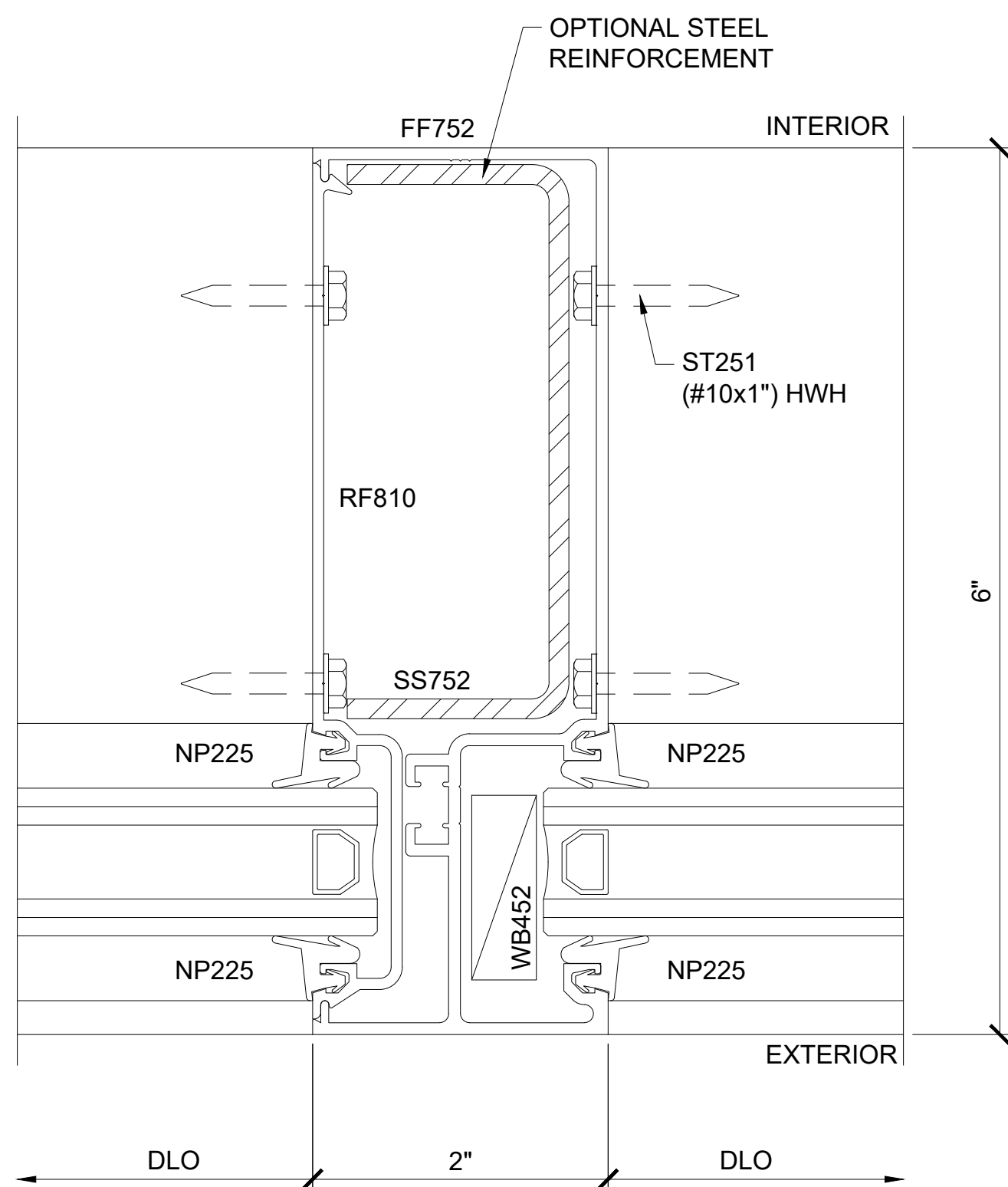
SECTION DETAIL AT INTERMEDIATE VERTICAL
