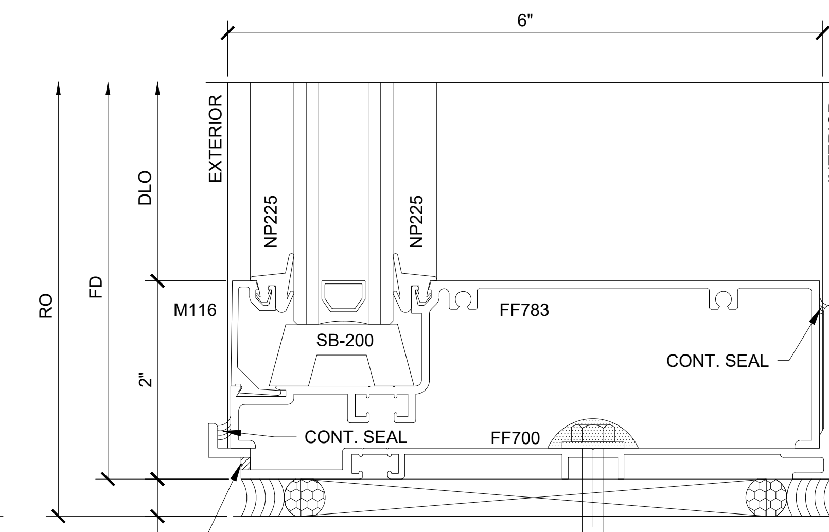
SECTION DETAIL AT SILL EXTERIOR GLAZING
