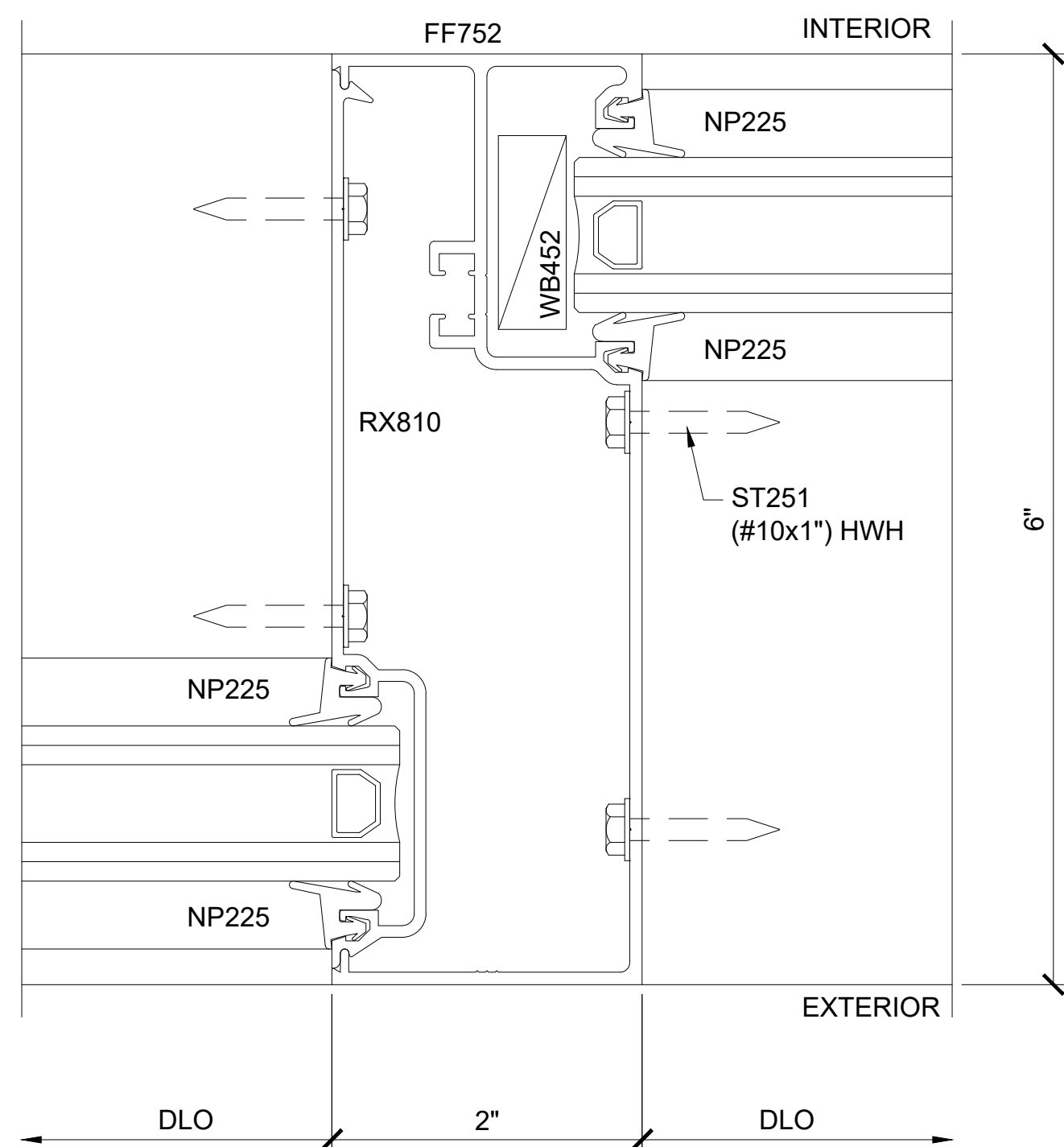
SECTION DETAIL AT INTERMEDIATE VERTICAL
