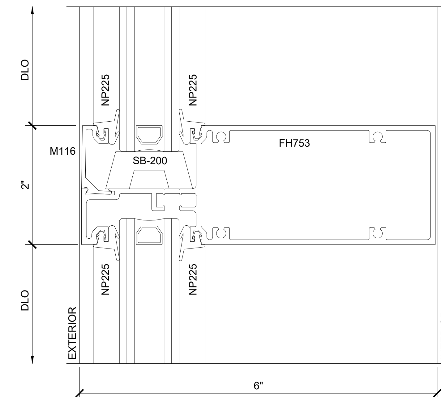
SECTION DETAIL AT INTERMEDIATE HORIZONTAL EXTERIOR GLAZING
