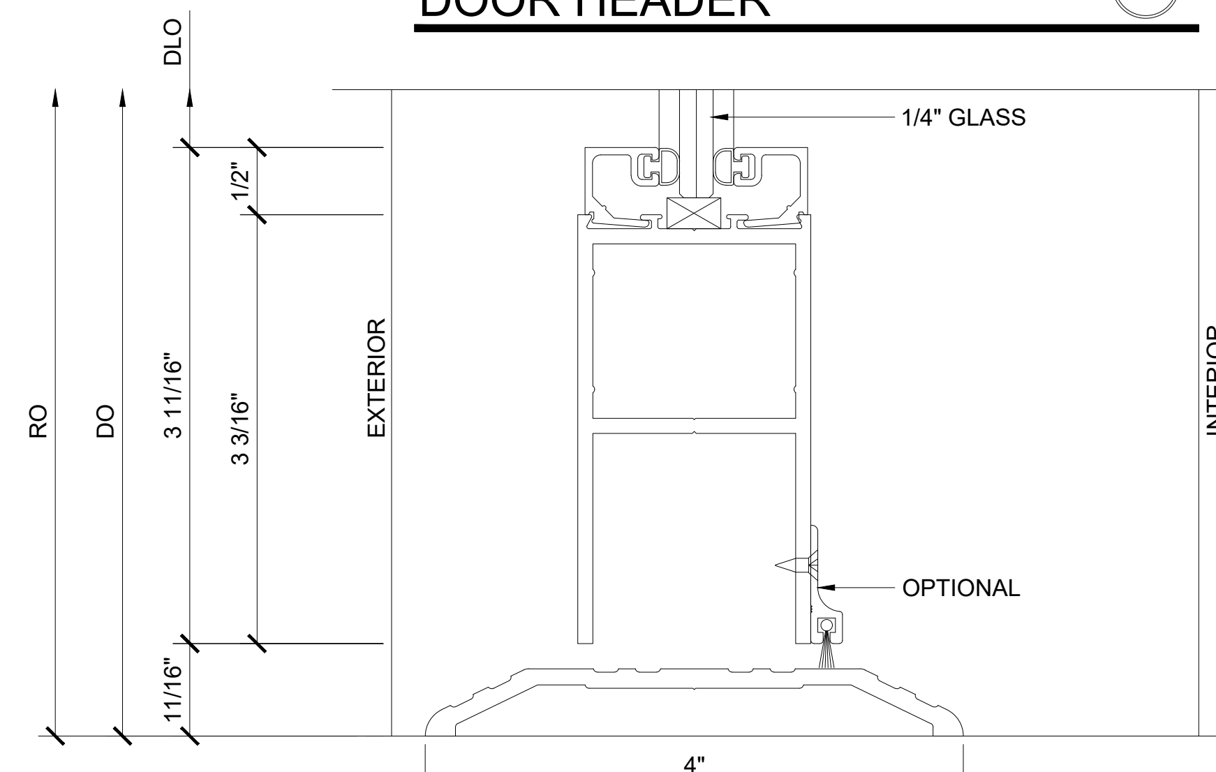
SECTION DETAIL AT BOTTOM RAIL
