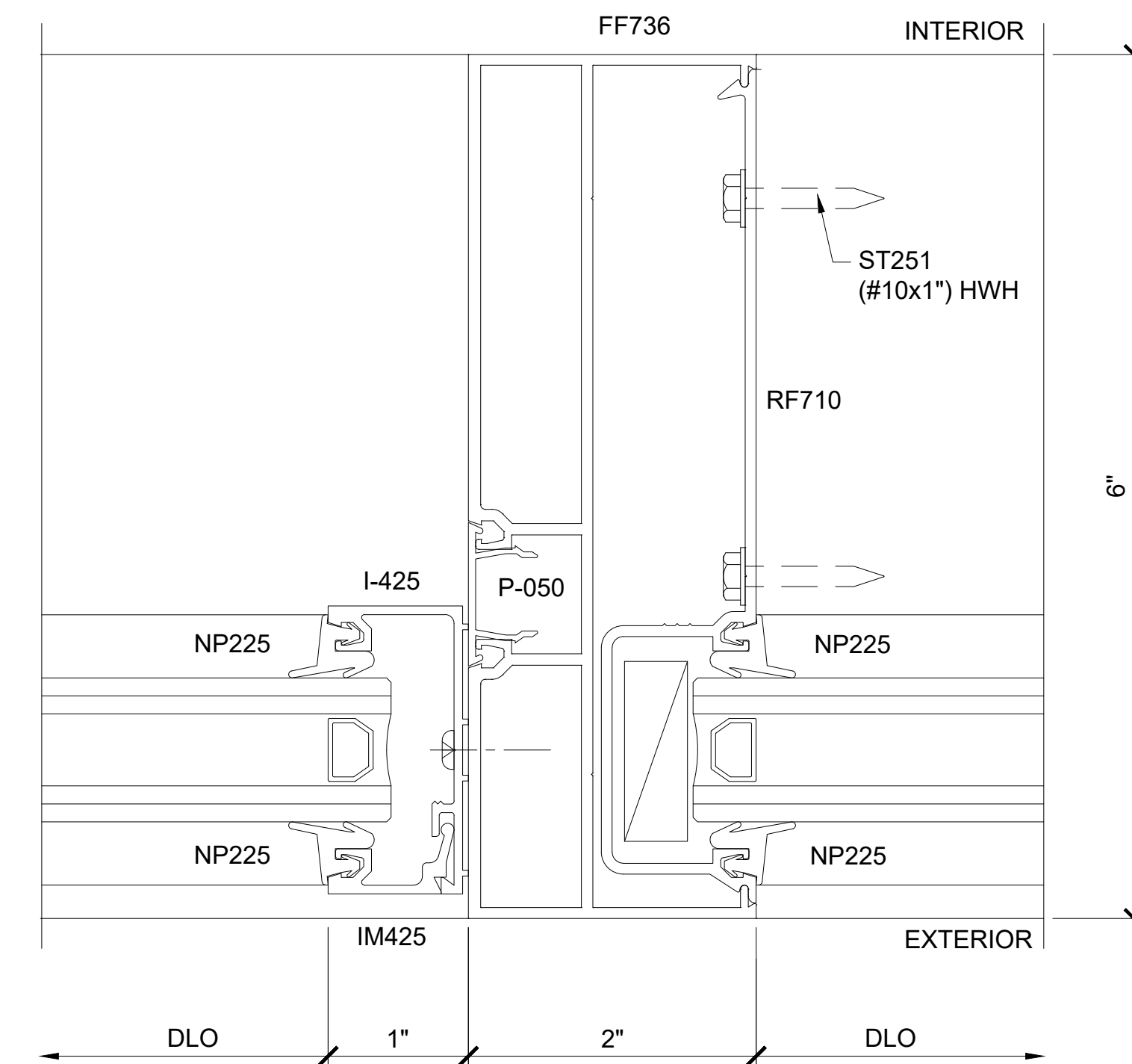
SECTION DETAIL AT INTERMEDIATE VERTICAL
