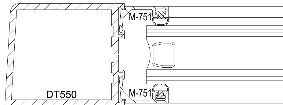
1" GLASS
