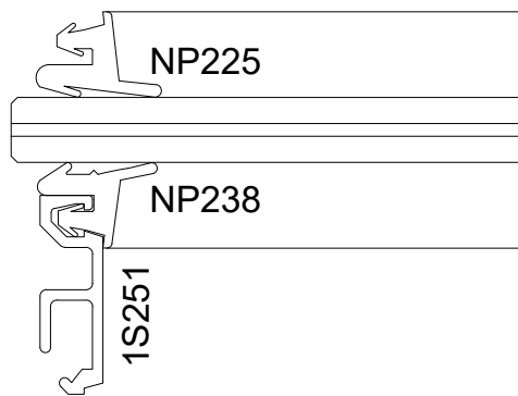
SECTION DETAIL AT FF601 - 5/16" GLASS 2
