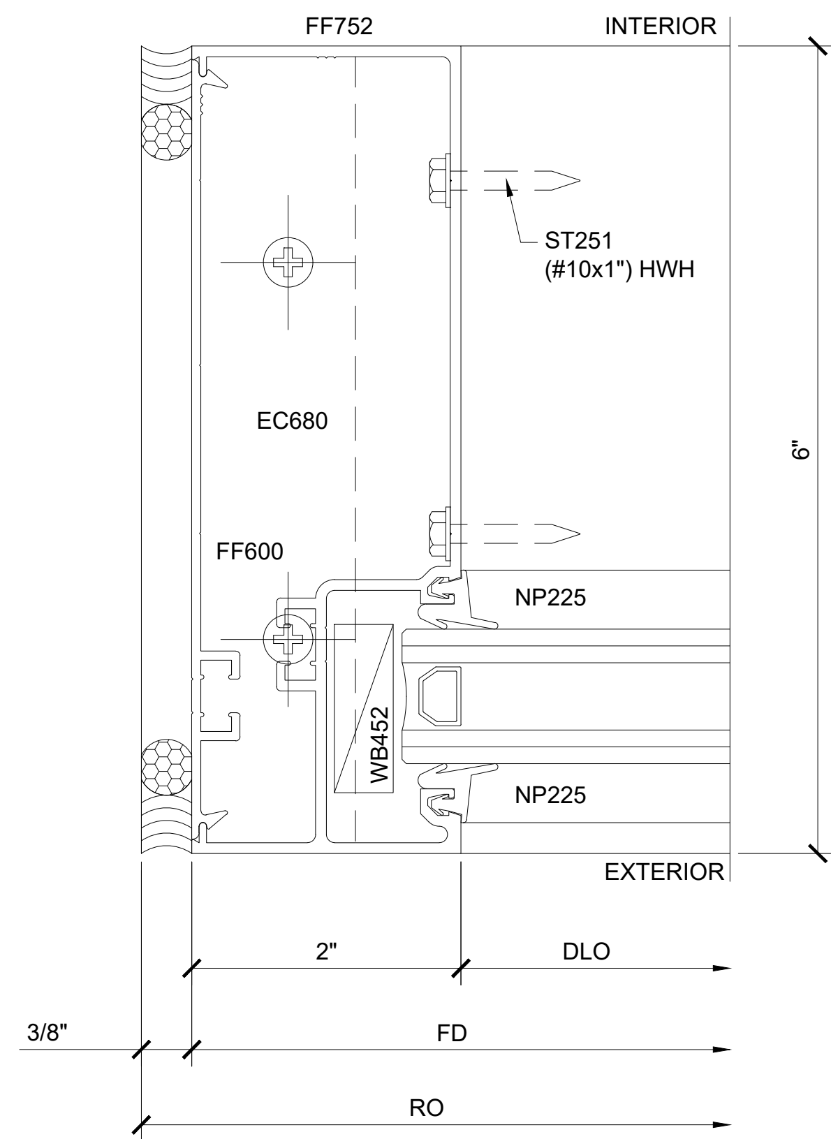
SECTION DETAIL AT JAMB
