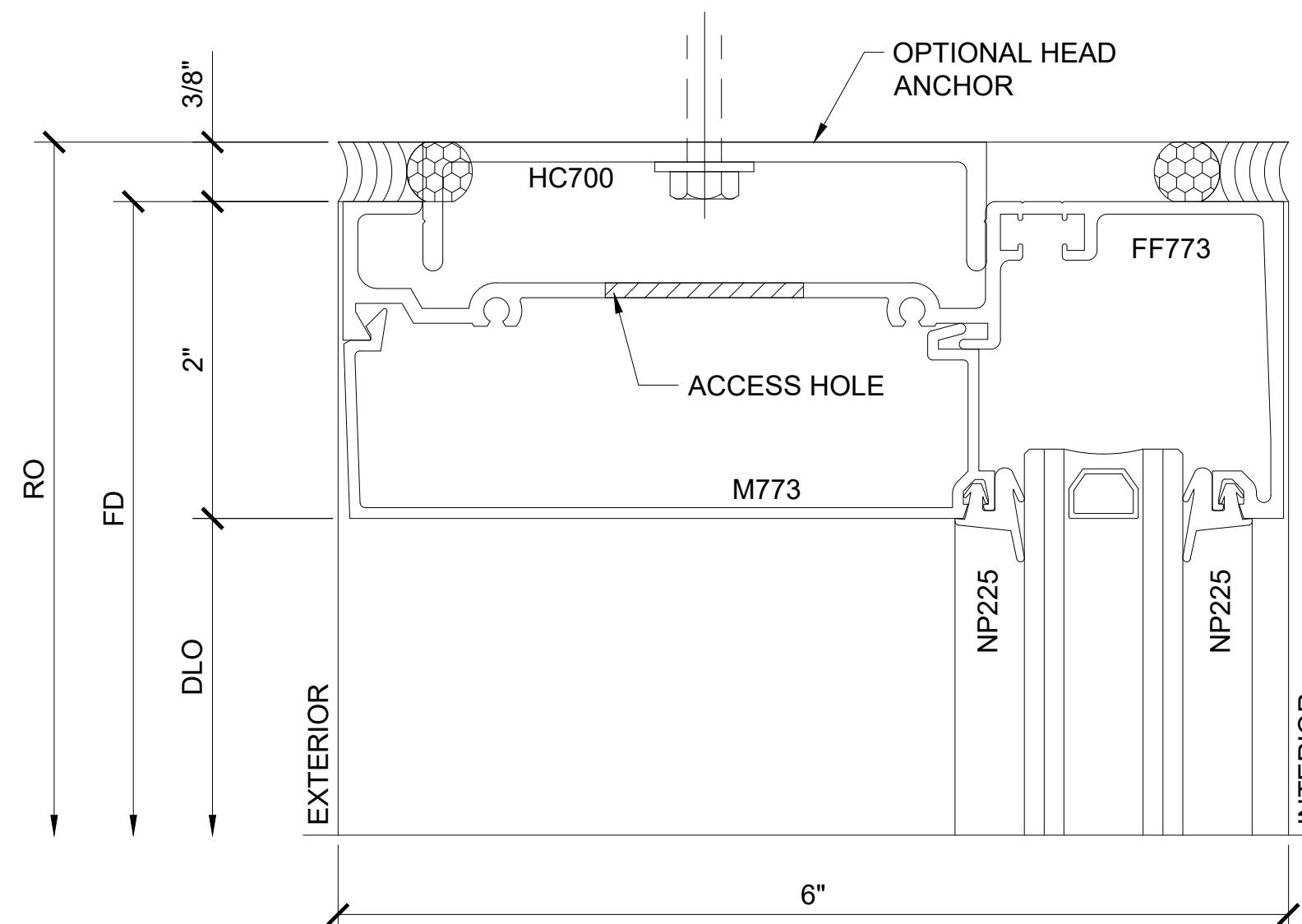
SECTION DETAIL AT HEAD W/ ANCHOR
