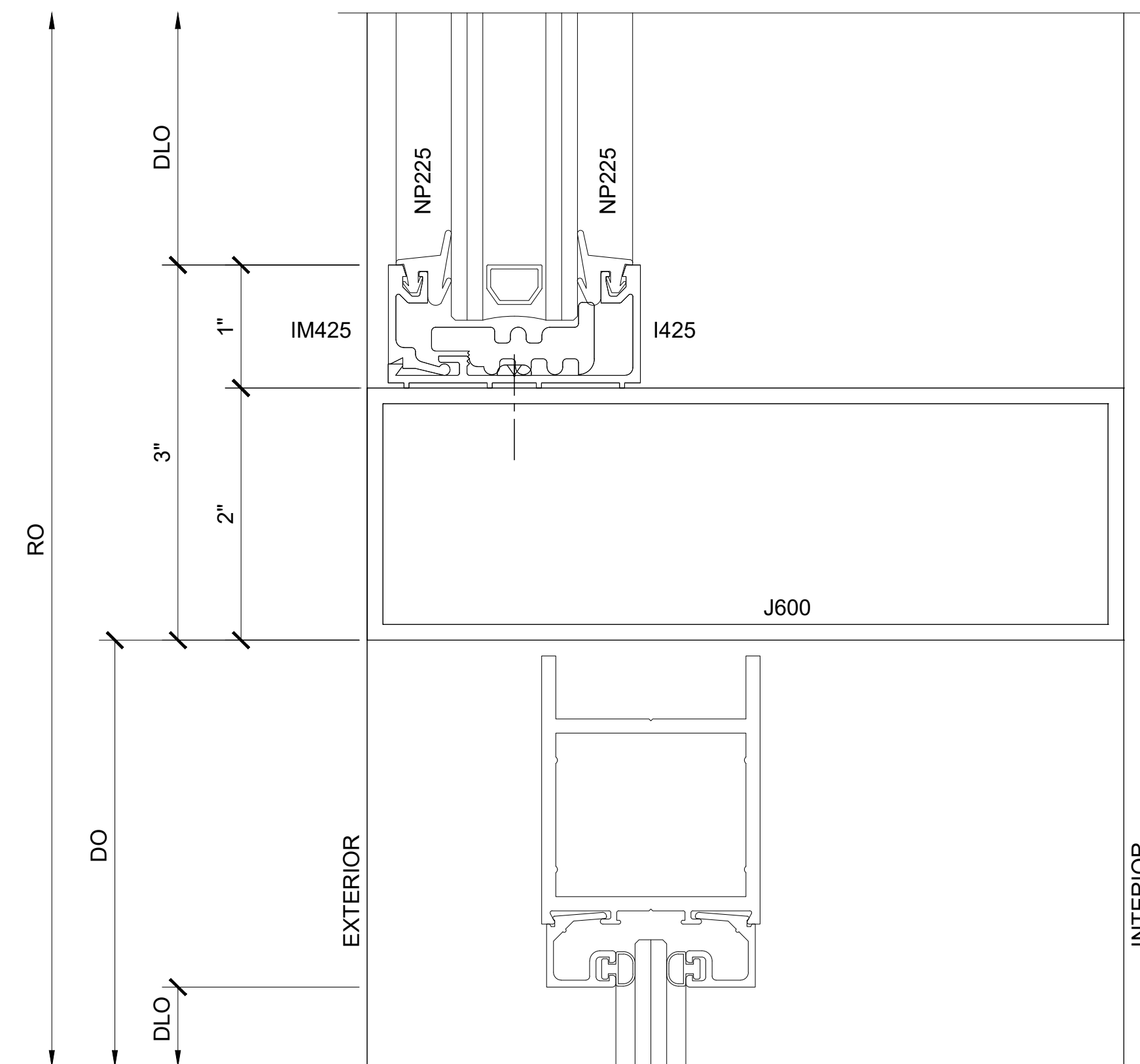
SECTION DETAIL AT DOOR HEADER
