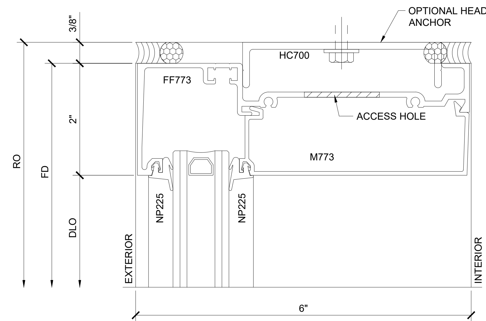
SECTION DETAIL AT HEAD WITH ANCHOR
