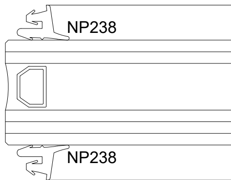
SECTION DETAIL AT FF601 - 1-1/8" GLASS 11
