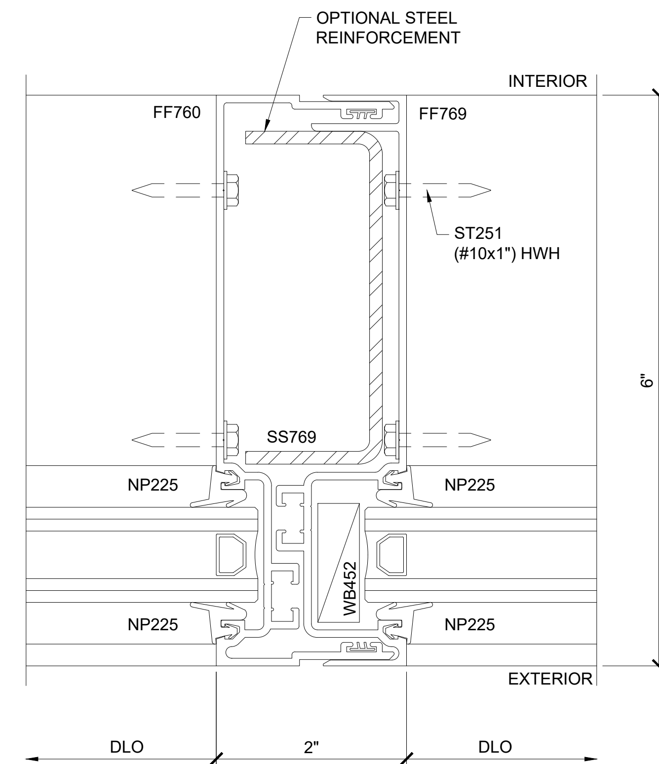
SECTION DETAIL EXPANSION INTERMEDIATE VERTICAL
