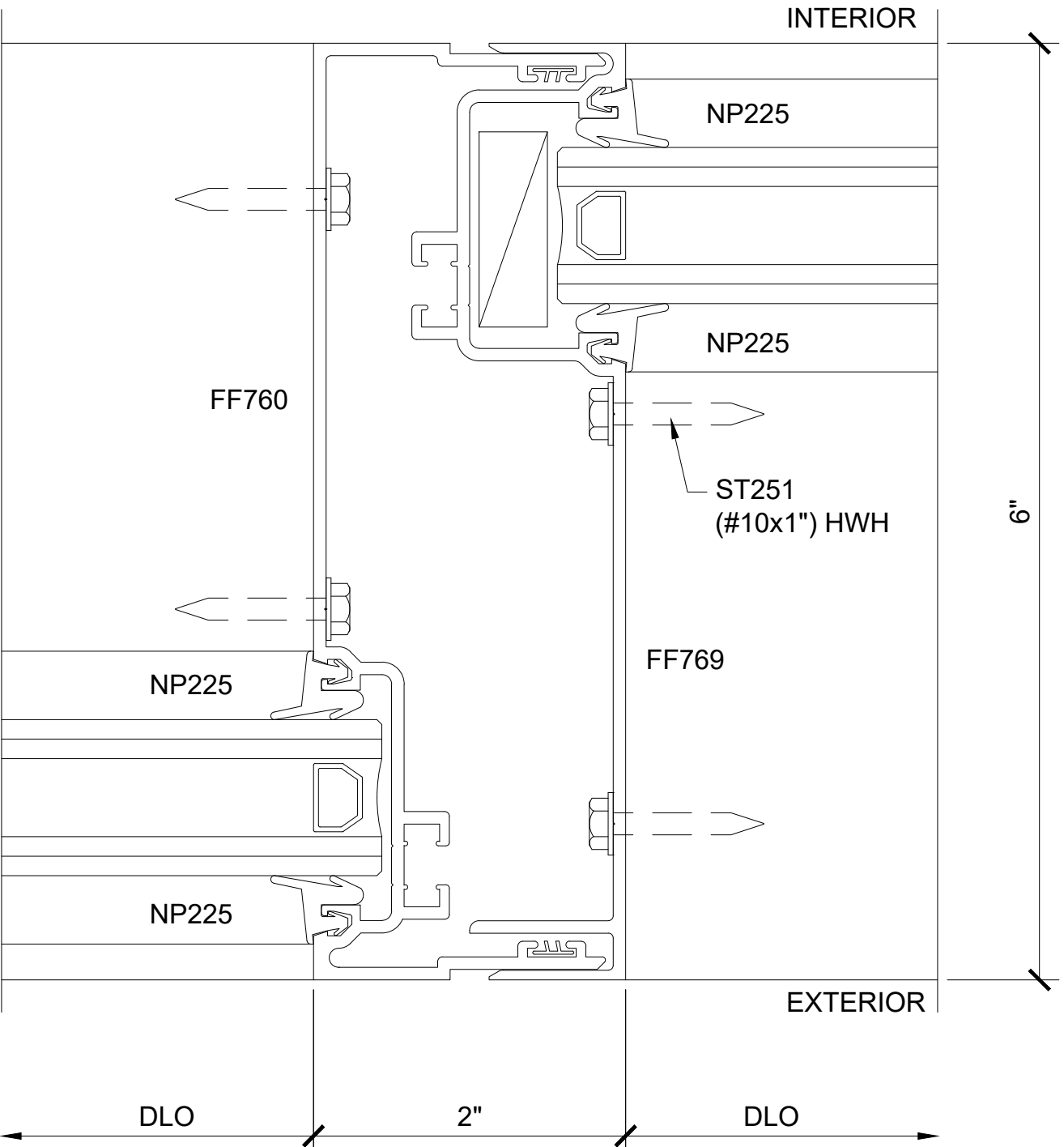
SECTION DETAIL EXPANSION INTERMEDIATE VERTICAL 10
