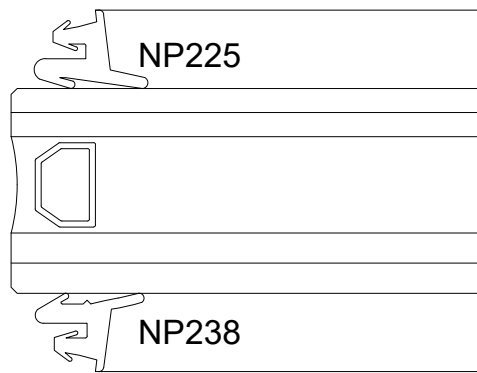
SECTION DETAIL AT FF601 - 1-1/16" GLASS 10
