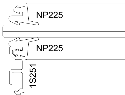
SECTION DETAIL AT FF601 - 1/4" GLASS 1
