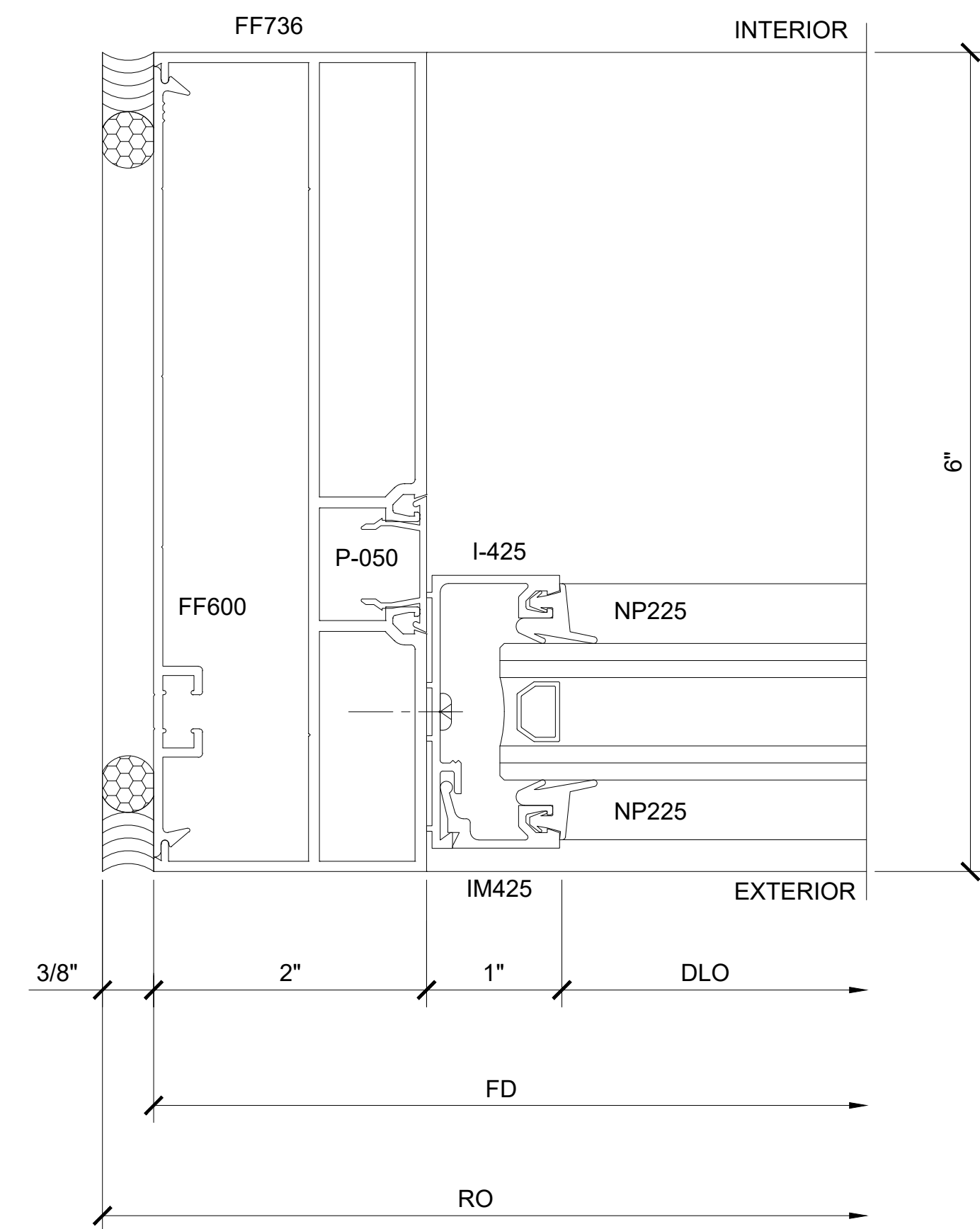
SECTION DETAIL AT JAMB ①
