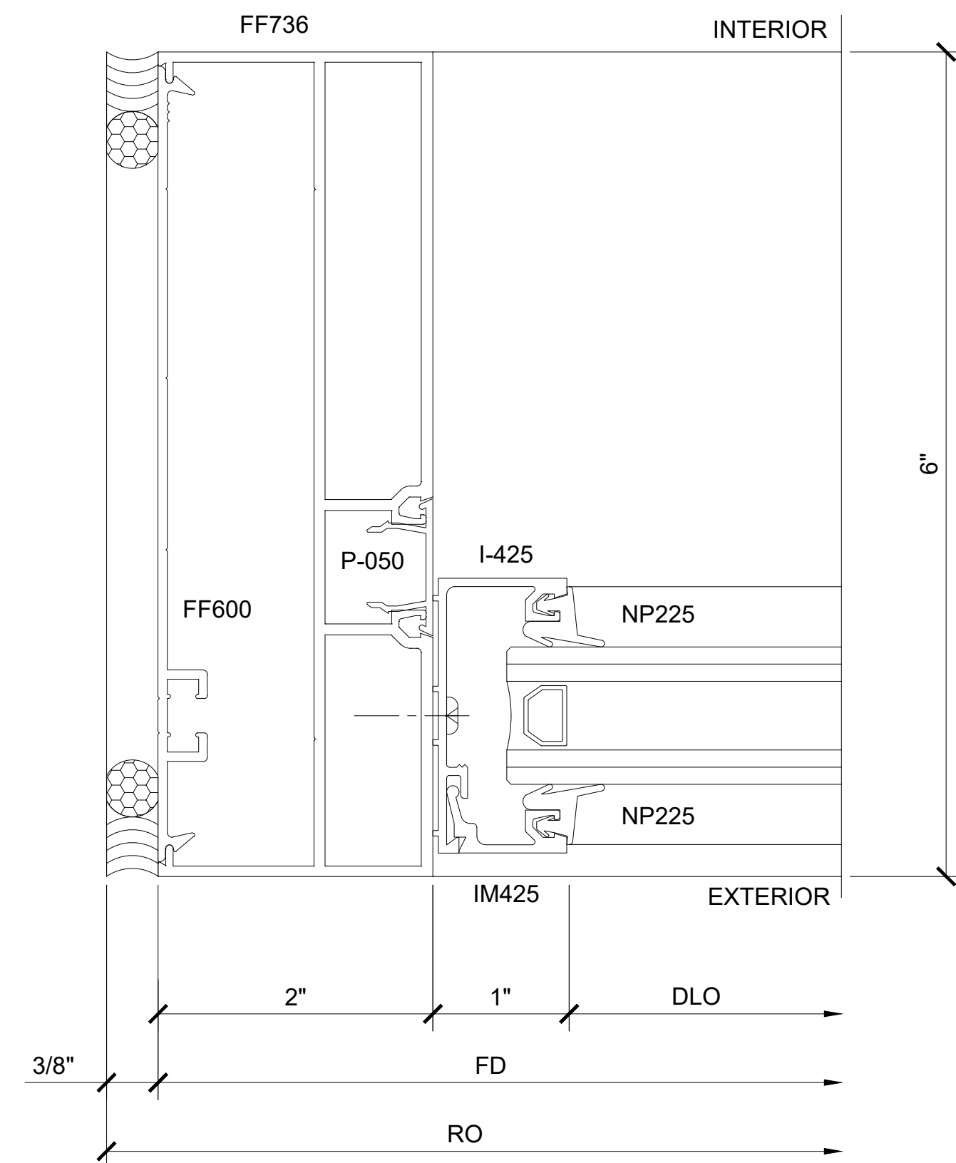
SECTION DETAIL AT JAMB
