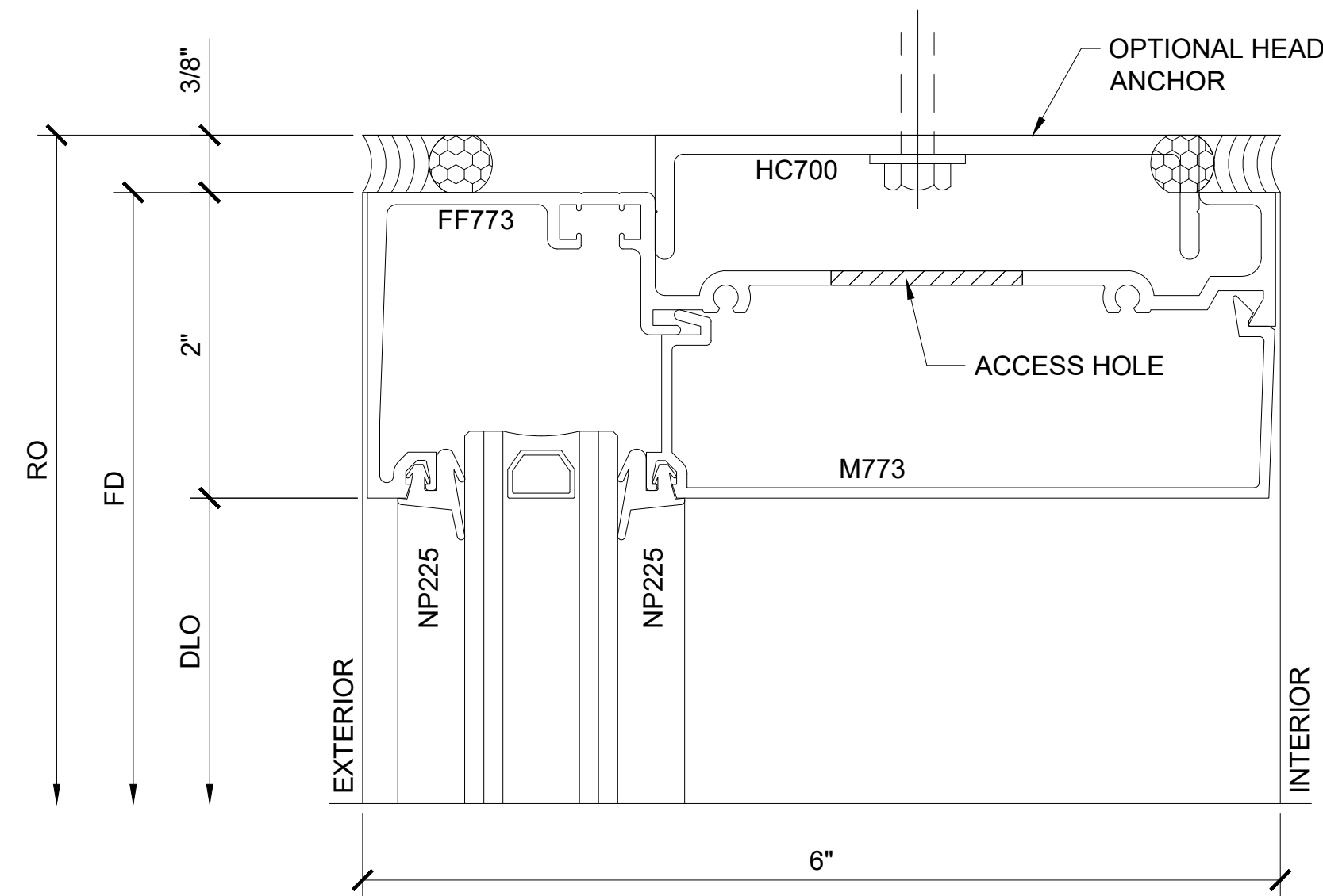
SECTION DETAIL AT HEAD W/ ANCHOR
