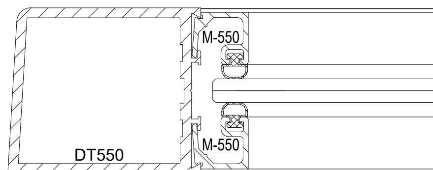
1/4" GLASS - SQUARE
