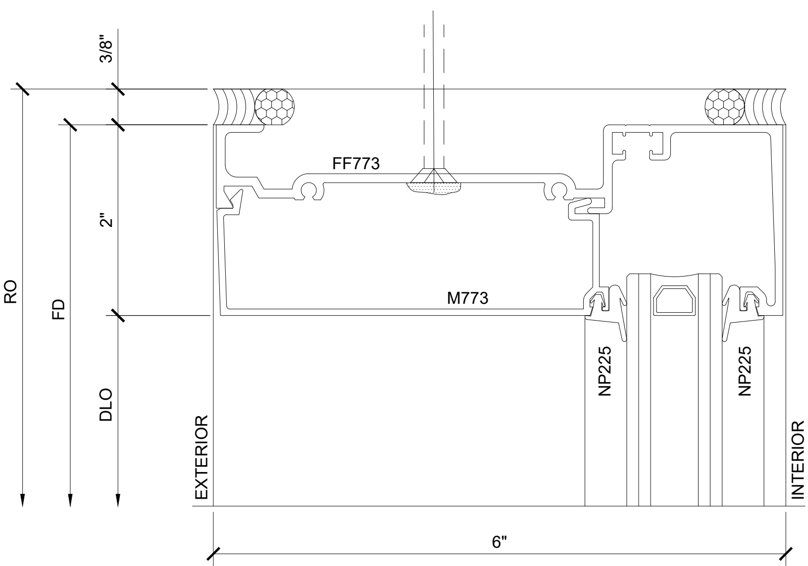
SECTION DETAIL AT HEAD 12
