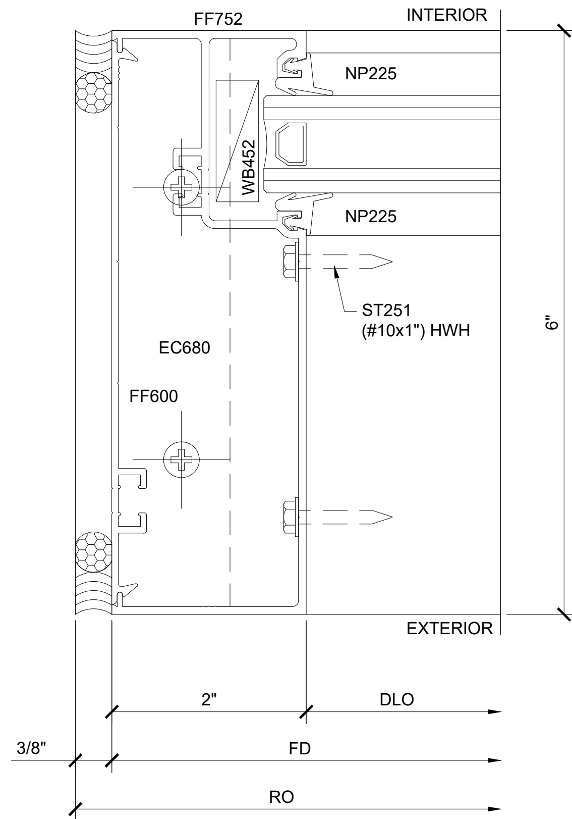
SECTION DETAIL AT JAMB
