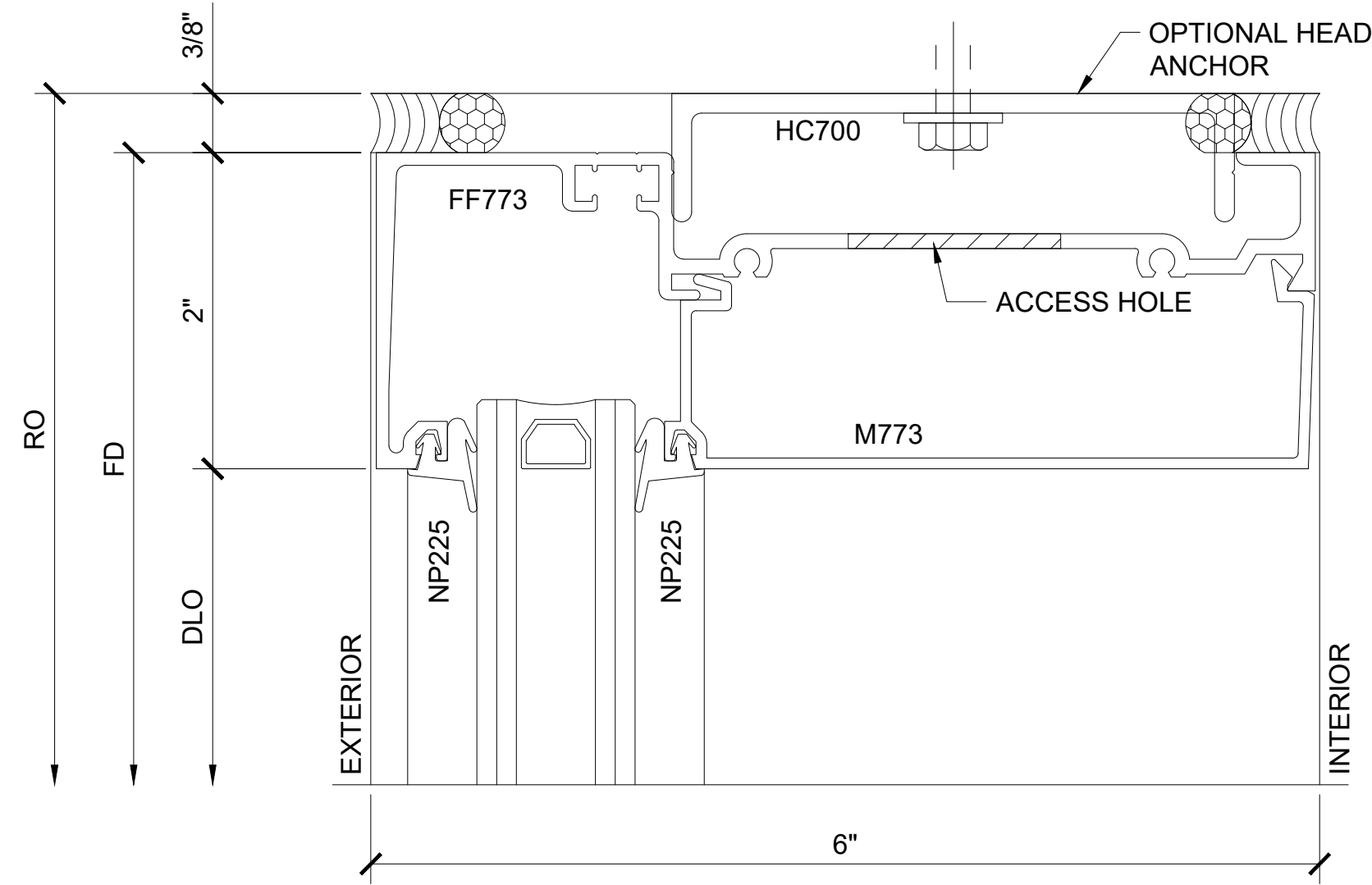
SECTION DETAIL AT HEAD WITH ANCHOR 7
