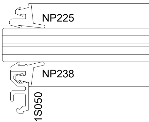
SECTION DETAIL AT FF601 - 9/16" GLASS 5
