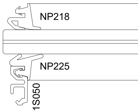
SECTION DETAIL AT FF601 - 7/16" GLASS 3
