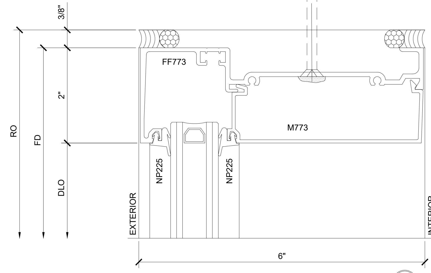
SECTION DETAIL AT HEAD
