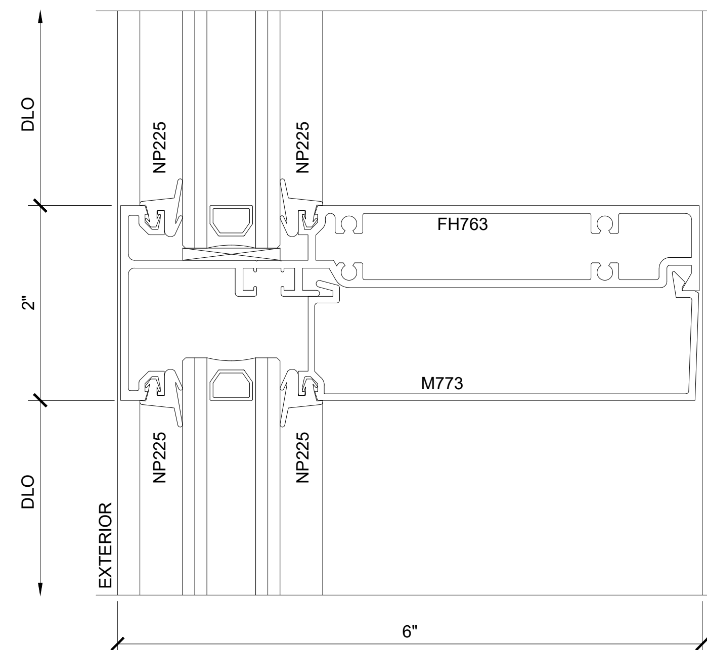
SECTION DETAIL AT INTERMEDIATE HORIZONTAL INTERIOR GLAZING
