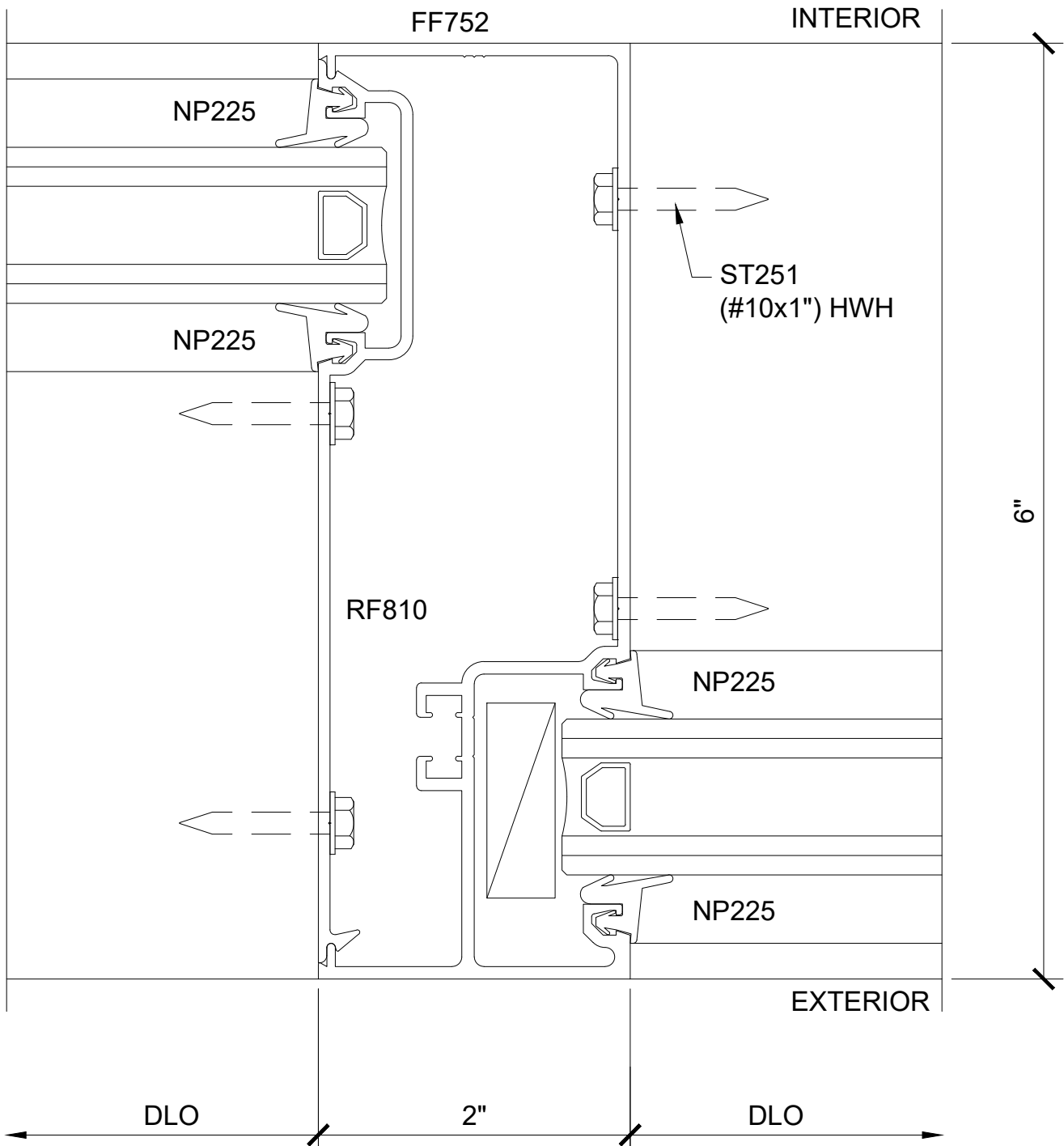
SECTION DETAIL AT INTERMEDIATE VERTICAL 9
