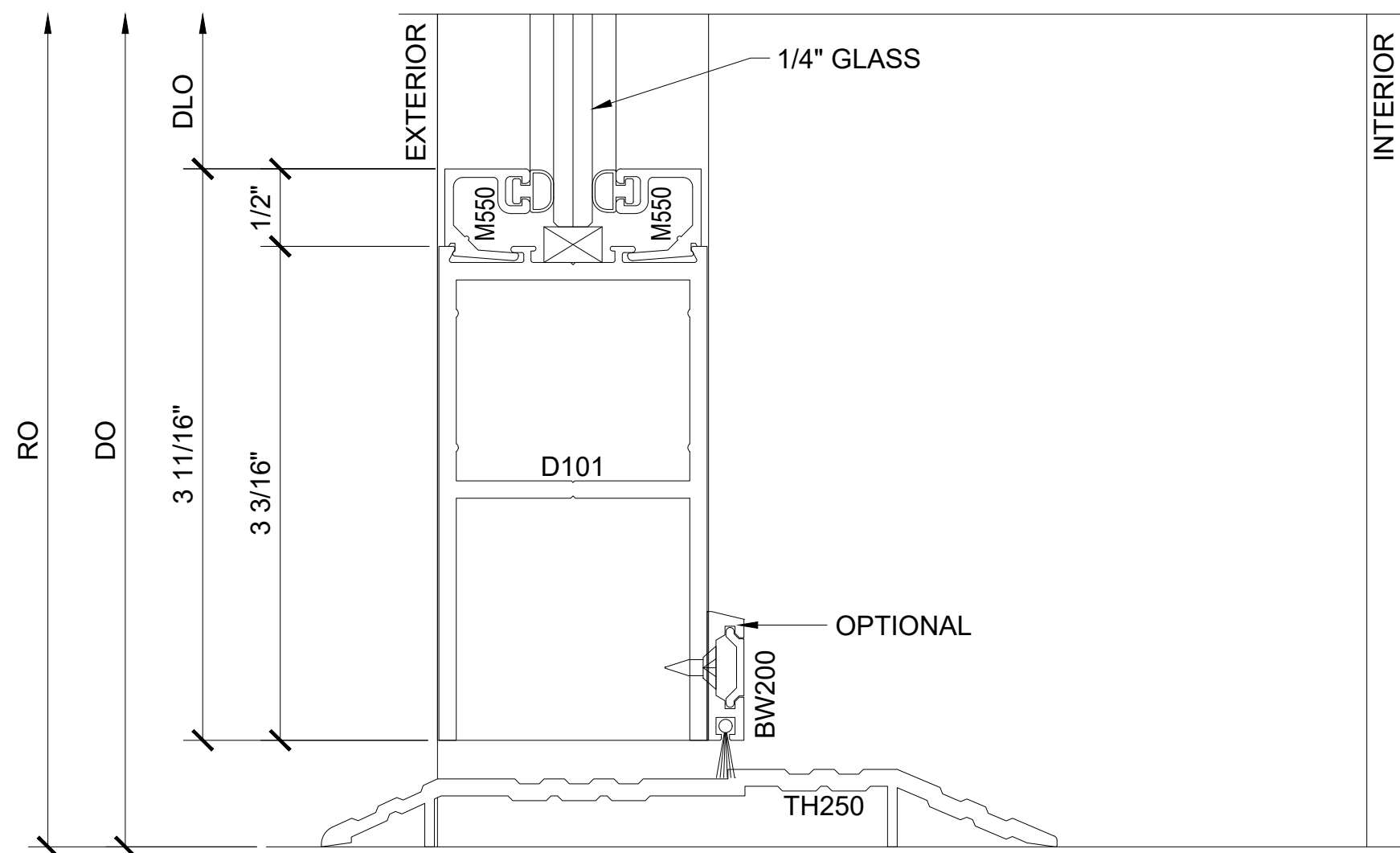
SECTION DETAIL @ BOTTOM RAIL 11
