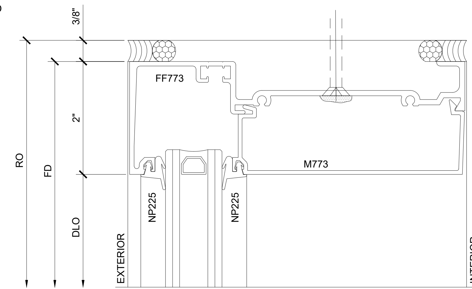
SECTION DETAIL AT HEAD
