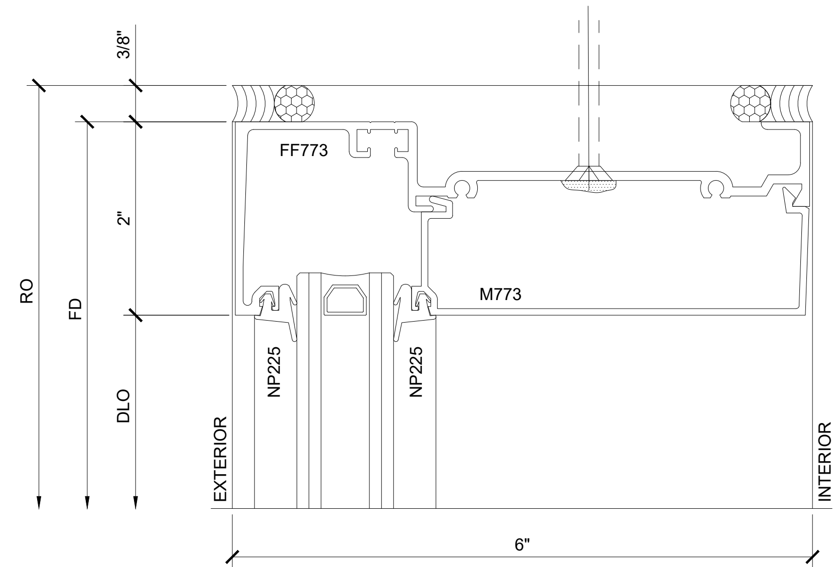
SECTION DETAIL AT HEAD
