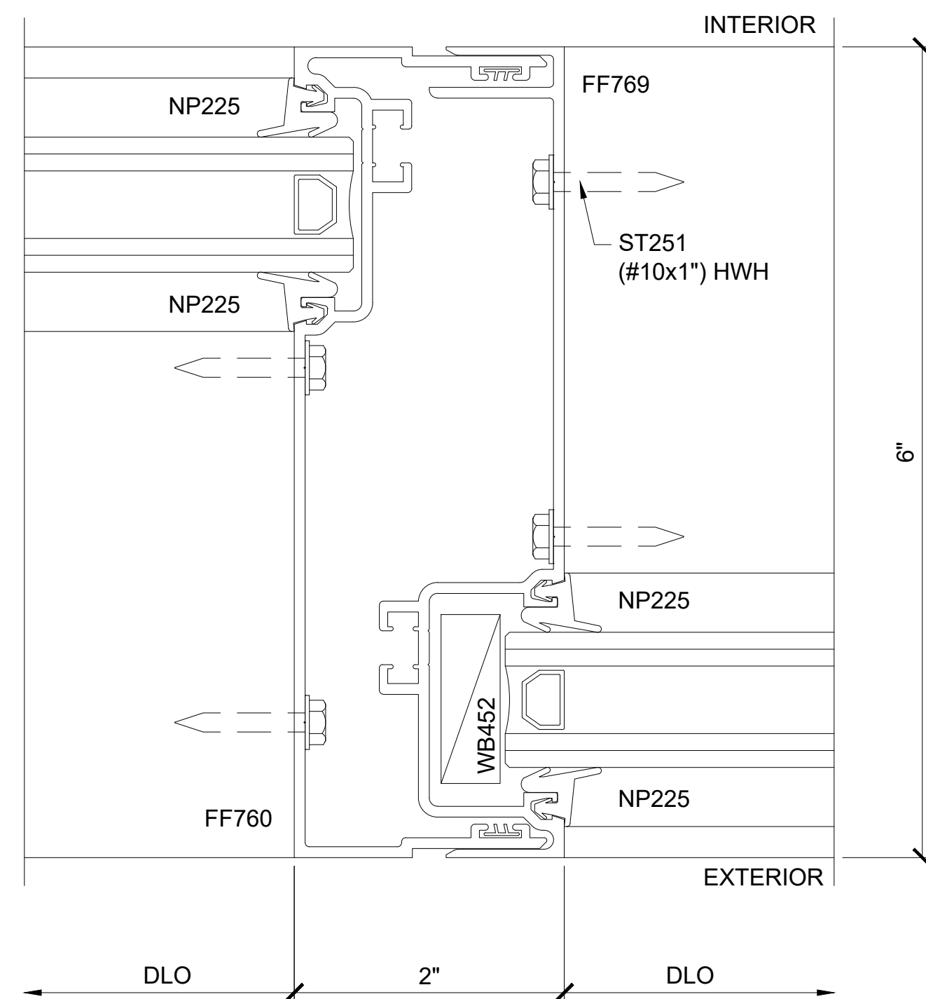
SECTION DETAIL EXPANSION INTERMEDIATE VERTICAL
