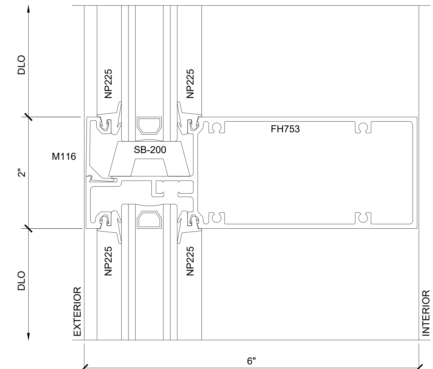
SECTION DETAIL AT INTERMEDIATE HORIZONTAL
