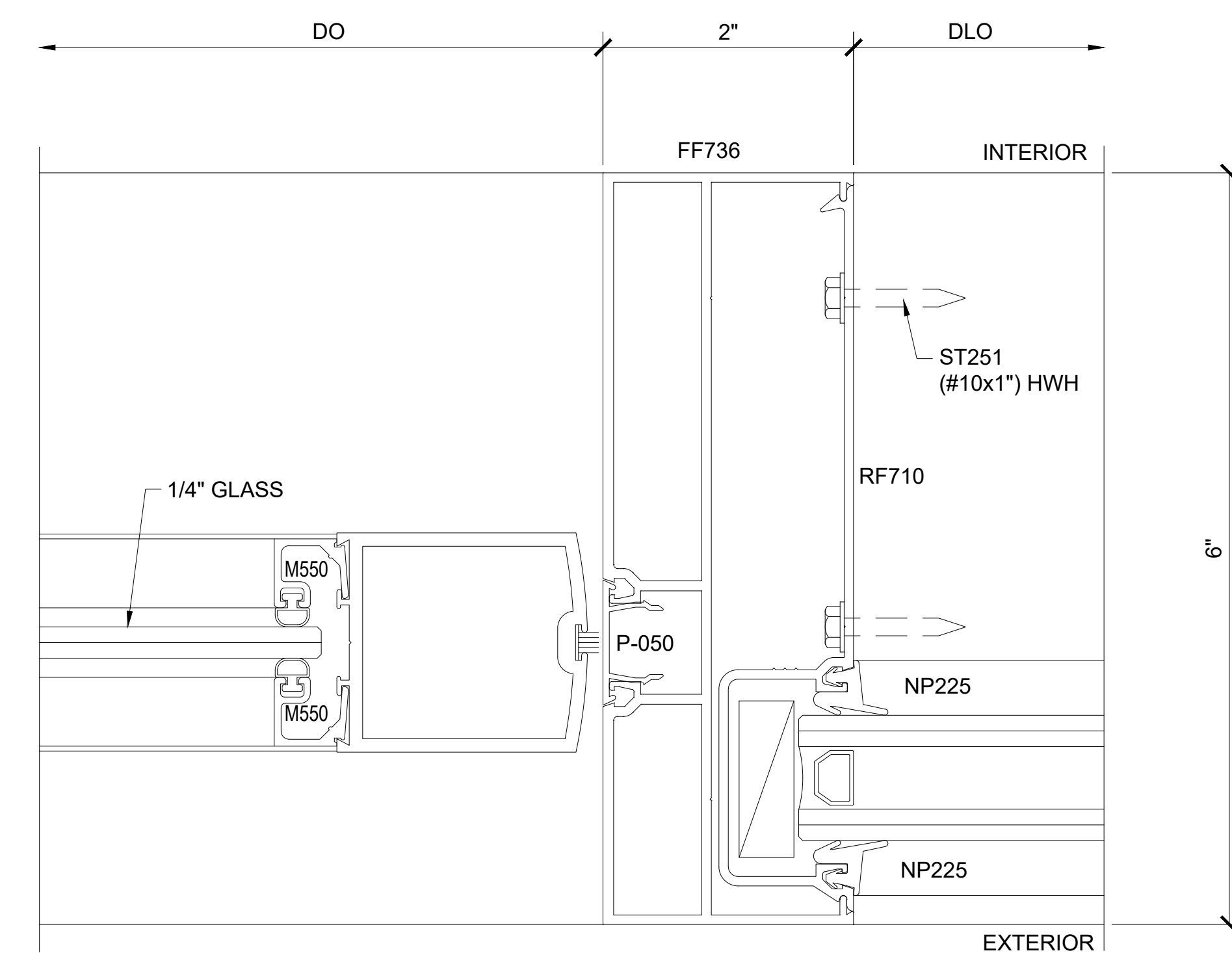
SECTION DETAIL AT DOOR INTERMEDIATE VERTICAL
