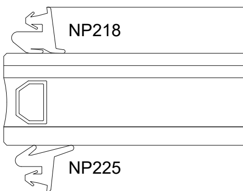
SECTION DETAIL AT FF601 - 15/16" GLASS 8
