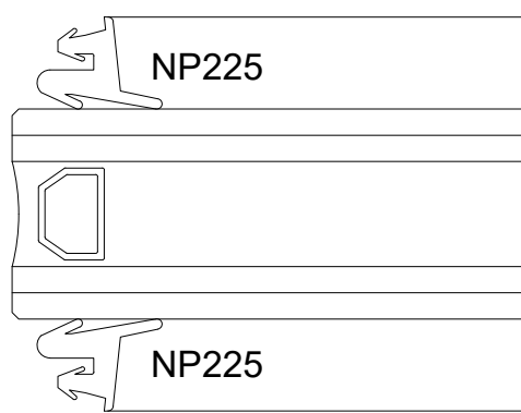
SECTION DETAIL AT FF601 - 1" GLASS 9
