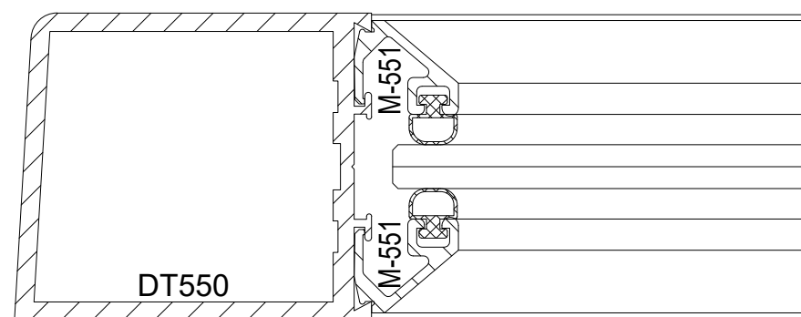
1/4" GLASS - TAPERED
