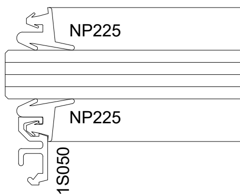
SECTION DETAIL AT FF601 - 1/2" GLASS 4
