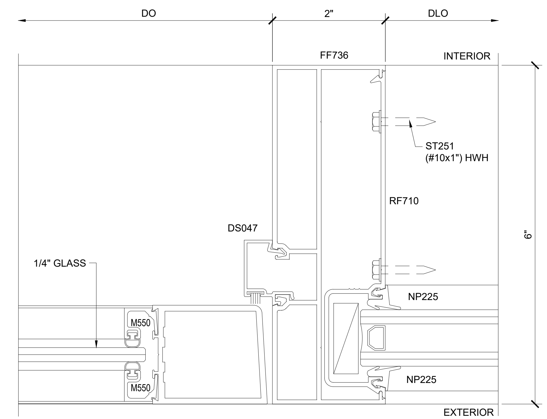
SECTION DETAIL AT DOOR INTERMEDIATE VERTICAL ⑥
