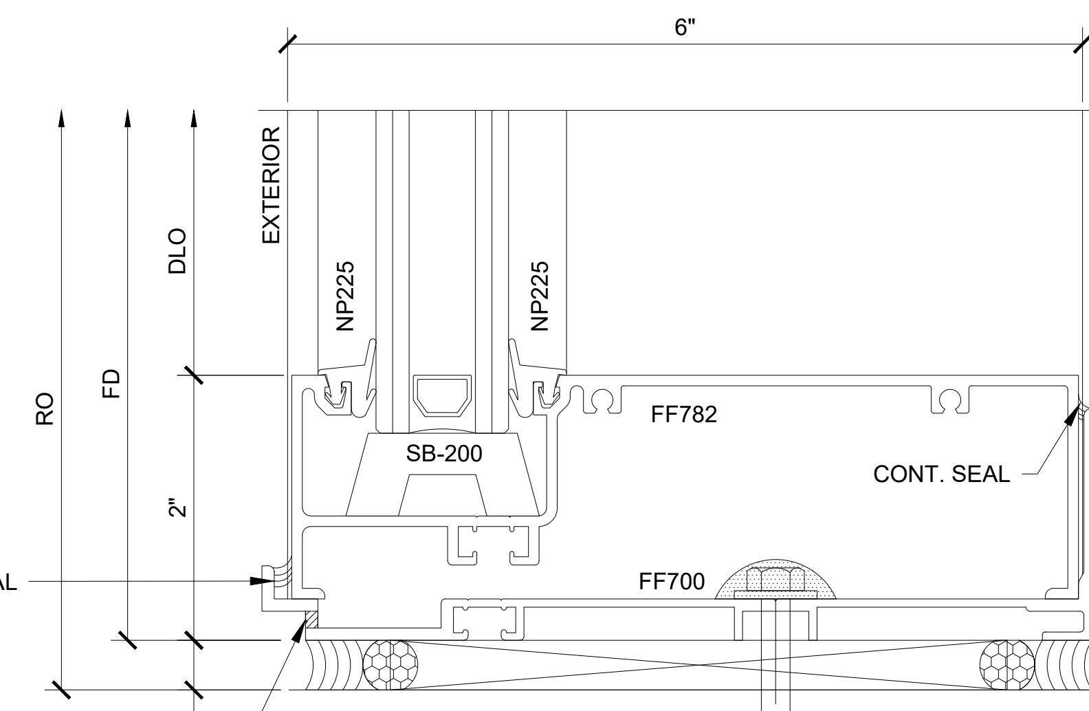
SECTION DETAIL AT SILL INTERIOR GLAZING
