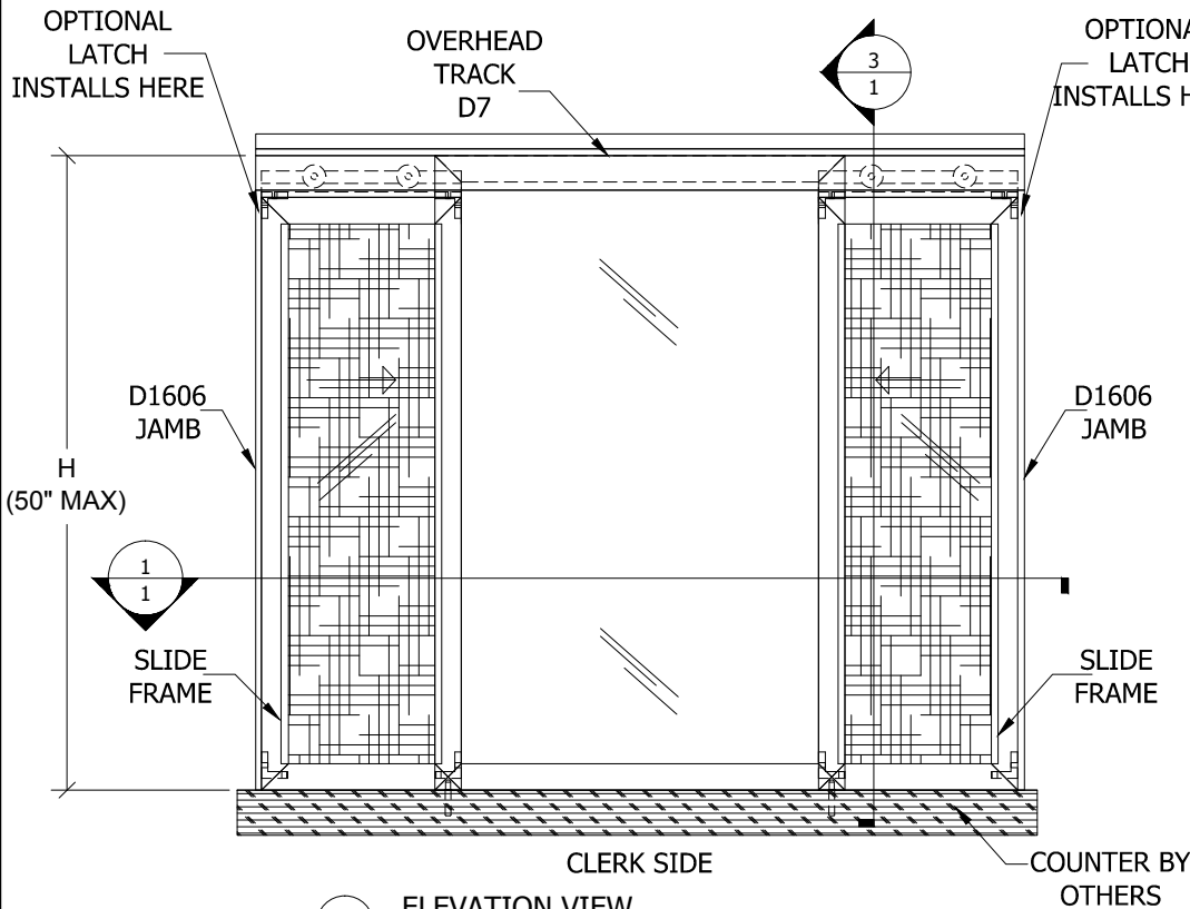
2 ELEVATION VIEW
