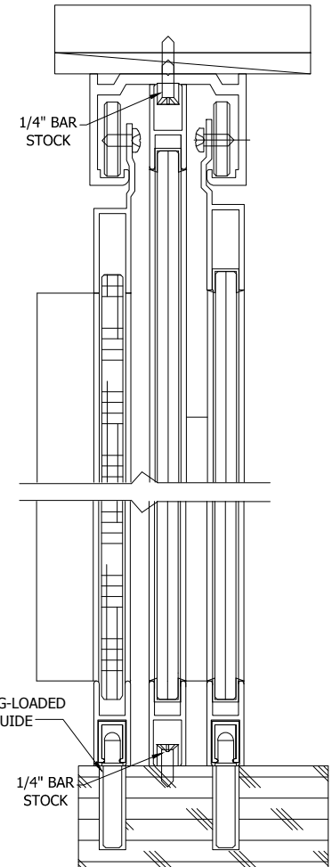
4 SECTION VIEW
