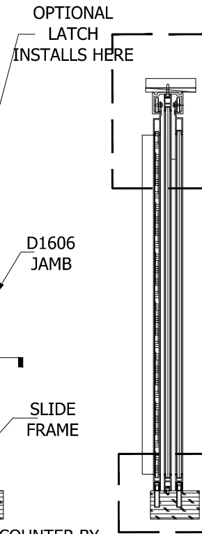
3 SECTION VIEW
