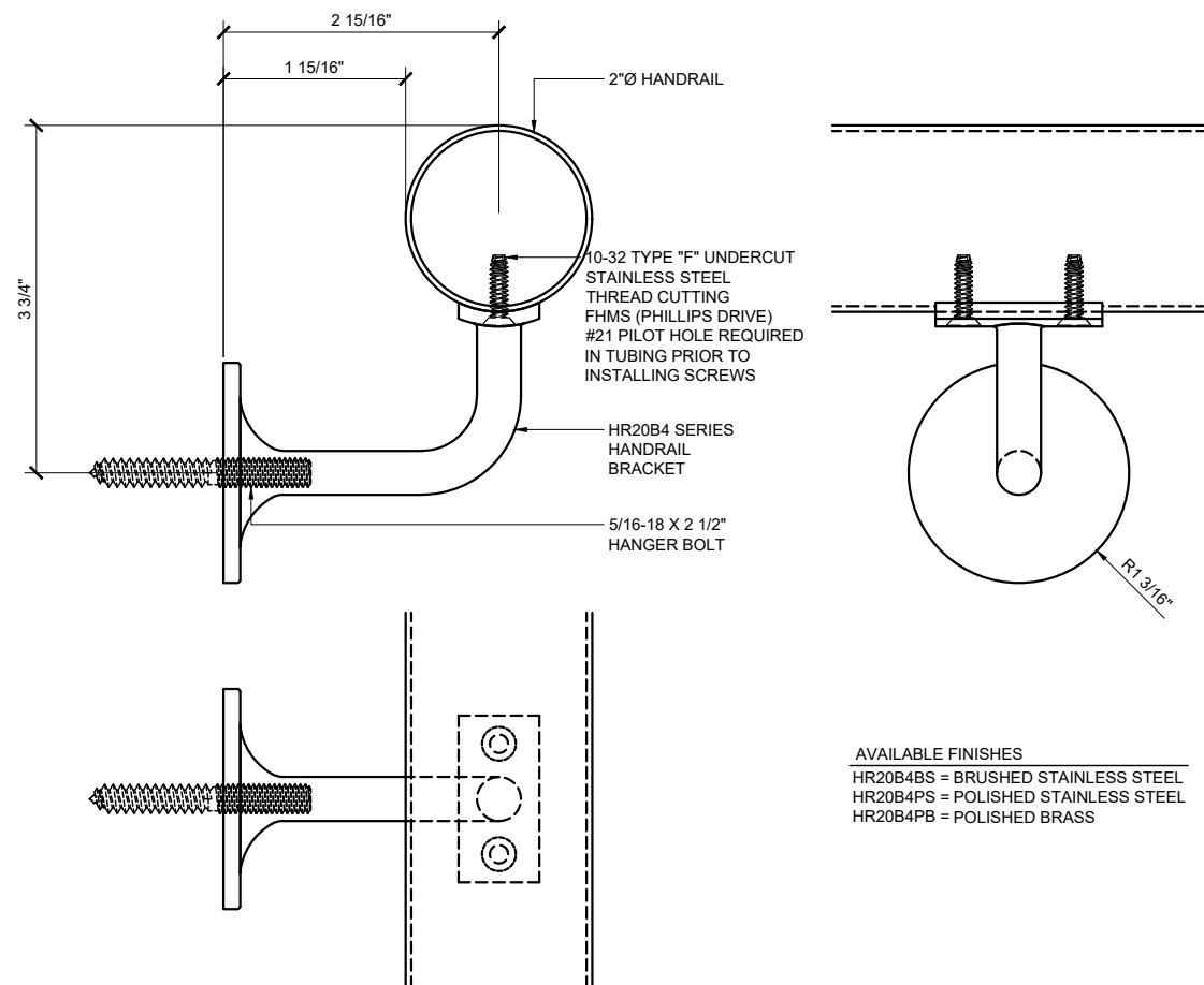
WALL MOUNT HANDRAIL BRACKET HR20B4 SERIES
