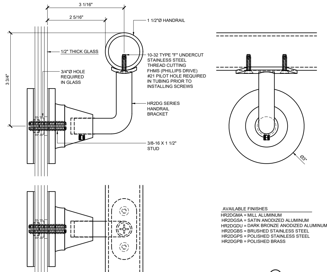
GLASS MOUNT HANDRAIL BRACKET HR2DG SERIES
