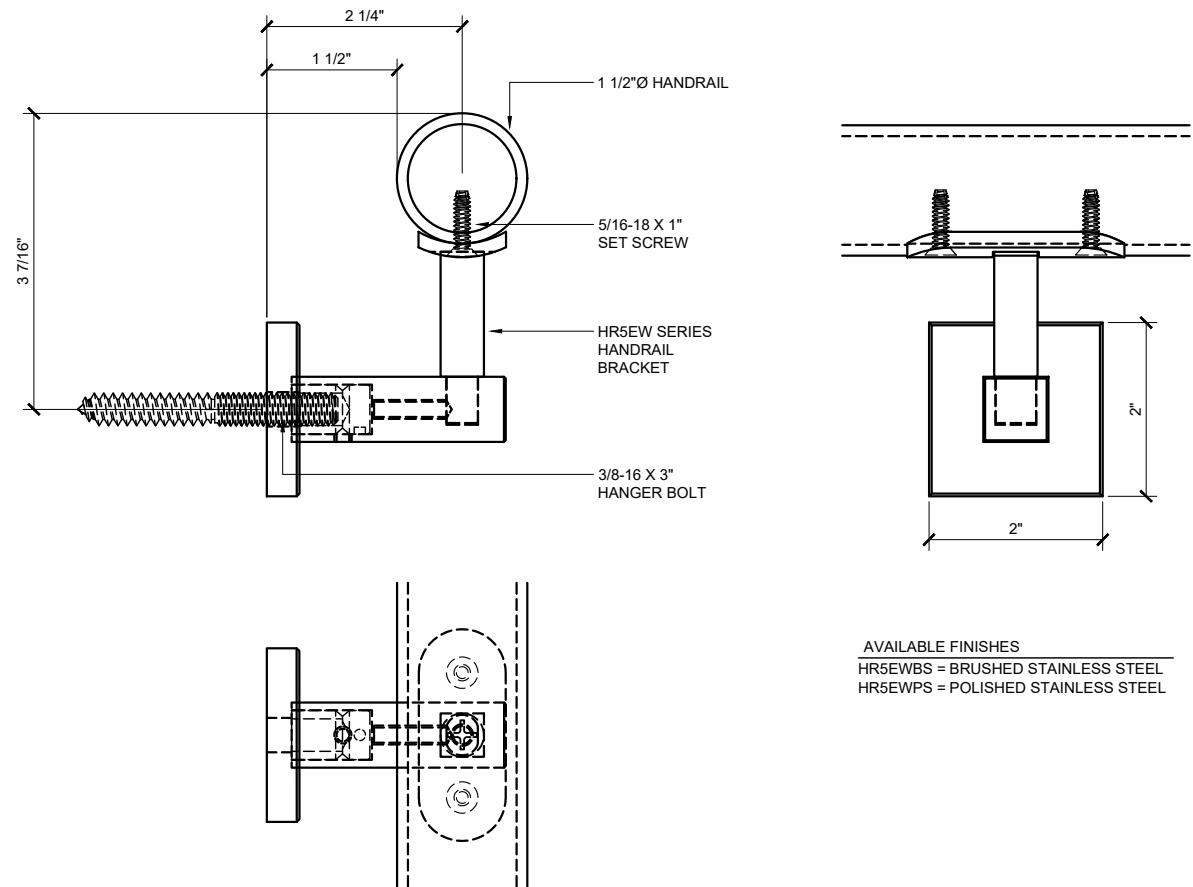
WALL MOUNT HANDRAIL BRACKET HR5EW SERIES ③
