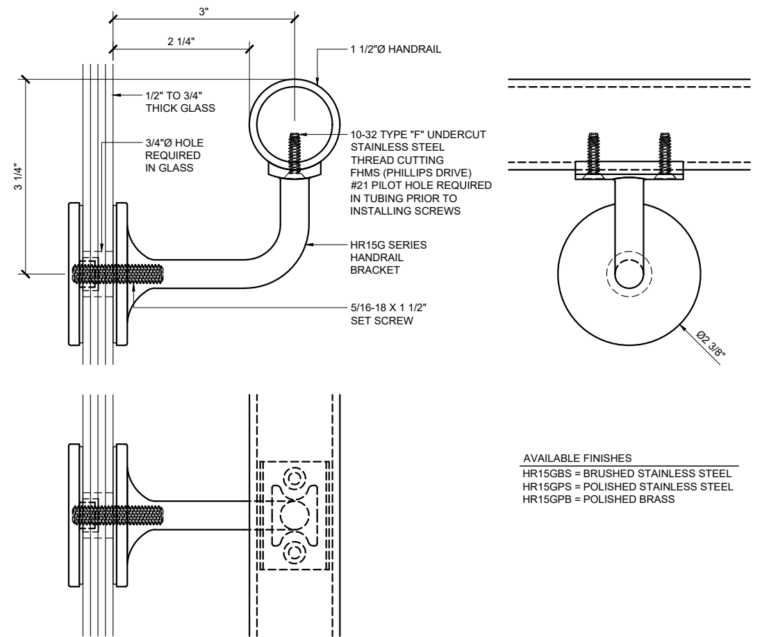
GLASS MOUNT HANDRAIL BRACKET HR15G SERIES
