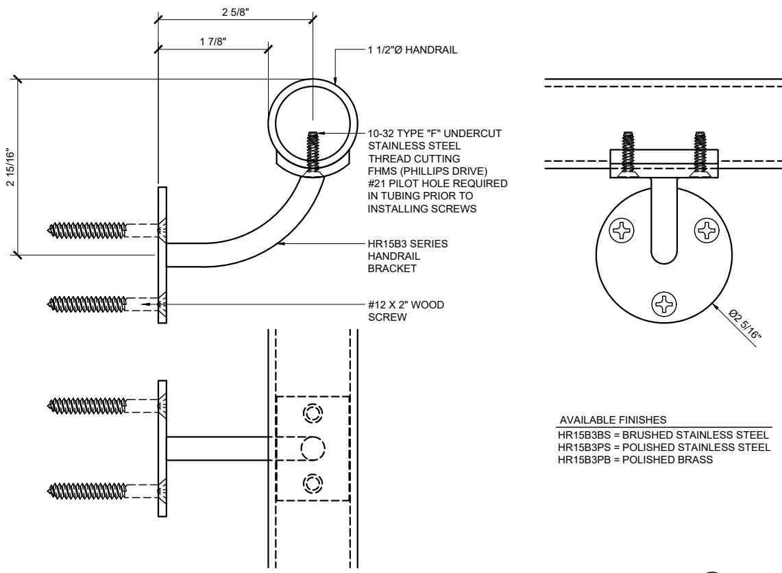
WALL MOUNT HANDRAIL BRACKET HR15B3 SERIES
