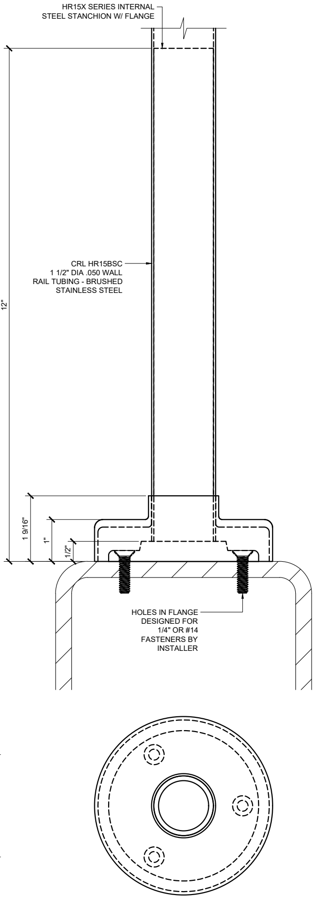
STEEL MOUNT
