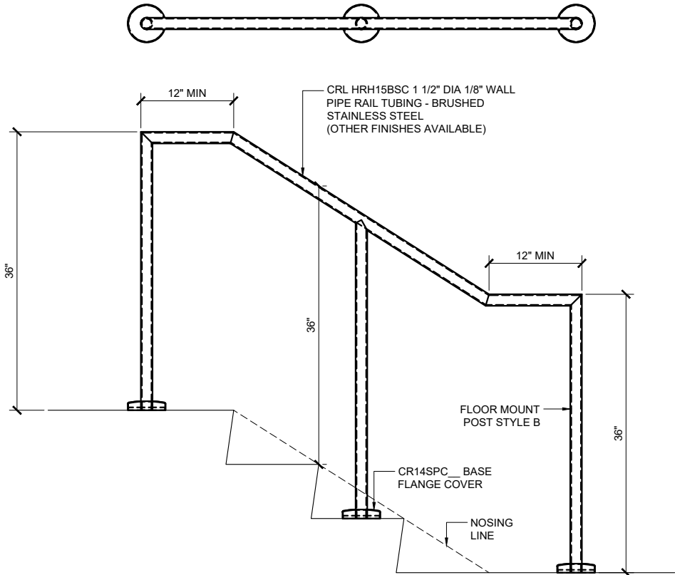
TYPICAL FREE STANDING HANDRAIL WITH MITERED CORNERS
