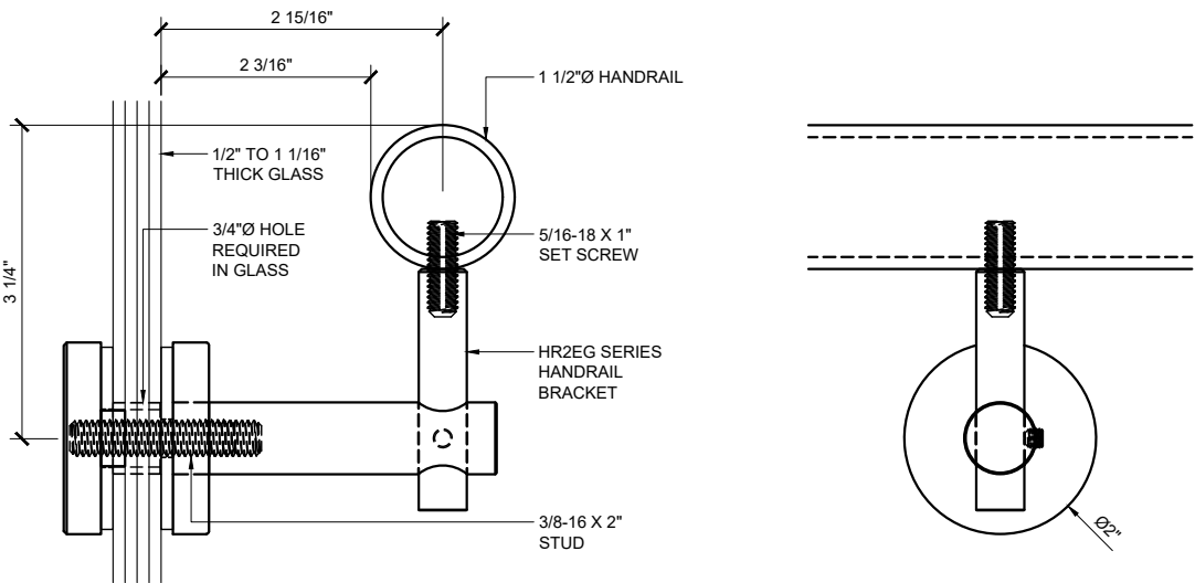
GLASS MOUNT HANDRAIL BRACKET HR2EG SERIES
