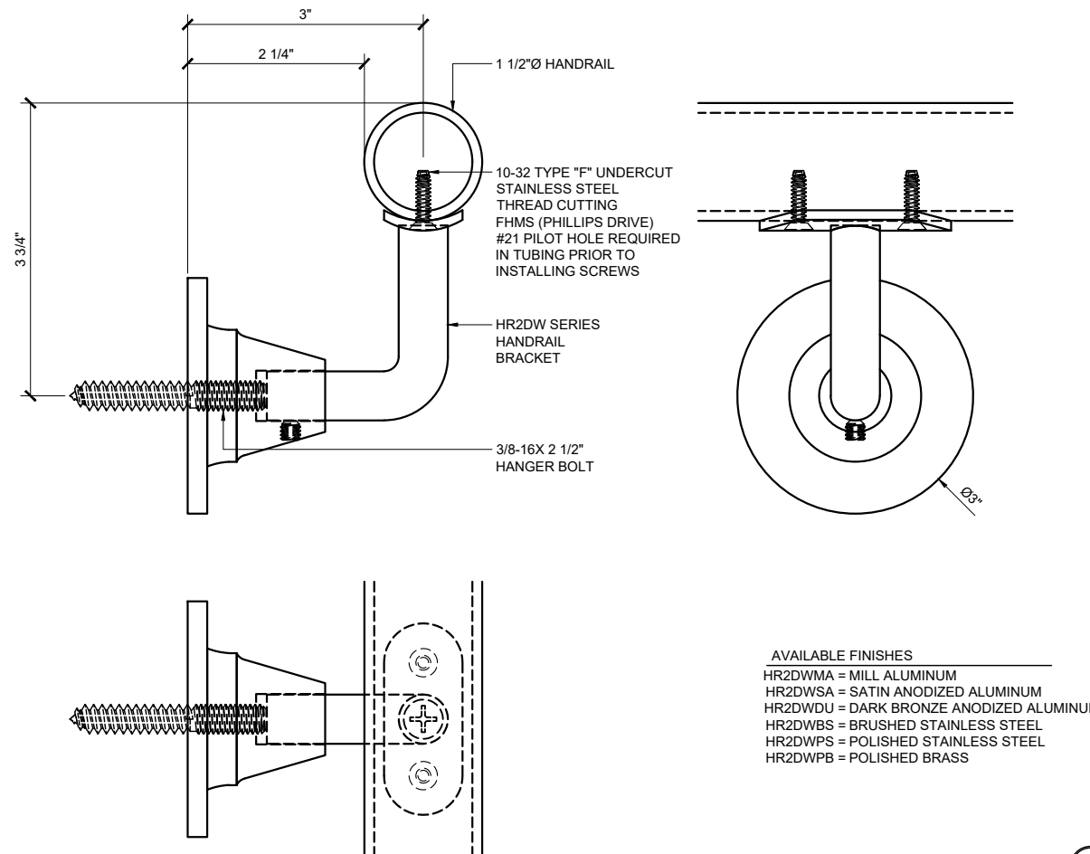
WALL MOUNT HANDRAIL BRACKET HR2DW SERIES
