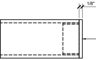
CRL HRH15EC FLAT END CAP FOR 1 1/2" O.D. TUBING
