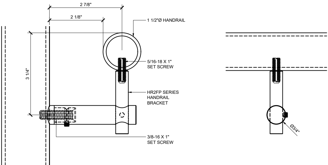
POST MOUNT HANDRAIL BRACKET HR2EP SERIES
