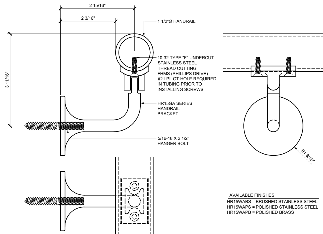
WALL MOUNT HANDRAIL BRACKET HR15WA SERIES
