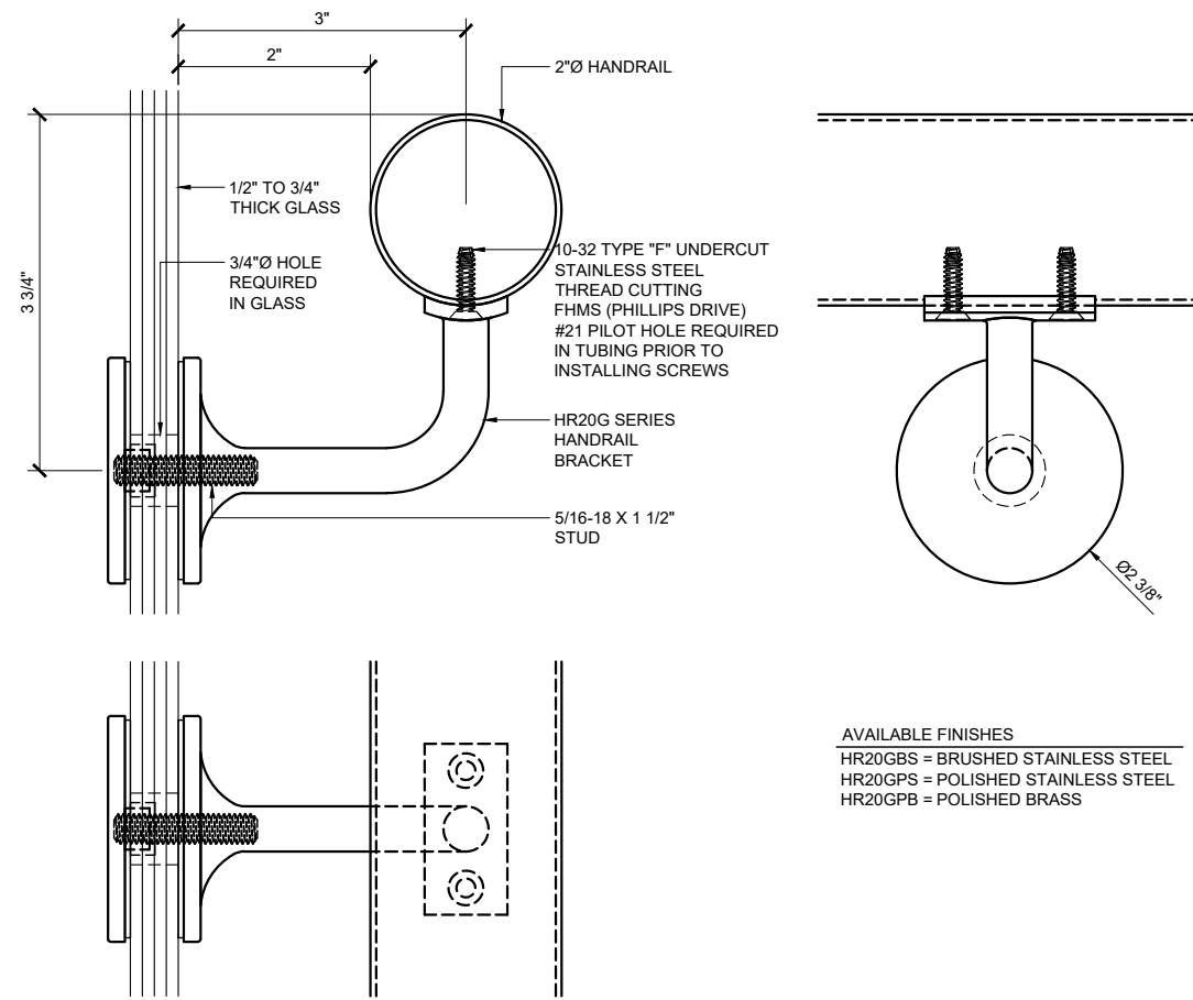
GLASS MOUNT HANDRAIL BRACKET HR20G SERIES
