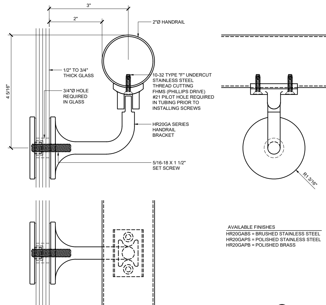
GLASS MOUNT HANDRAIL BRACKET HR20GA SERIES
