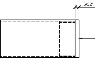
CRL HR15F FLAT END CAP FOR 1 1/2" O.D. HAND RAIL TUBING
