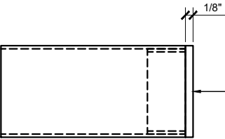
CRL SA10 FLAT END CAP FOR 1 1/2" SQUARE HAND RAIL TUBING
