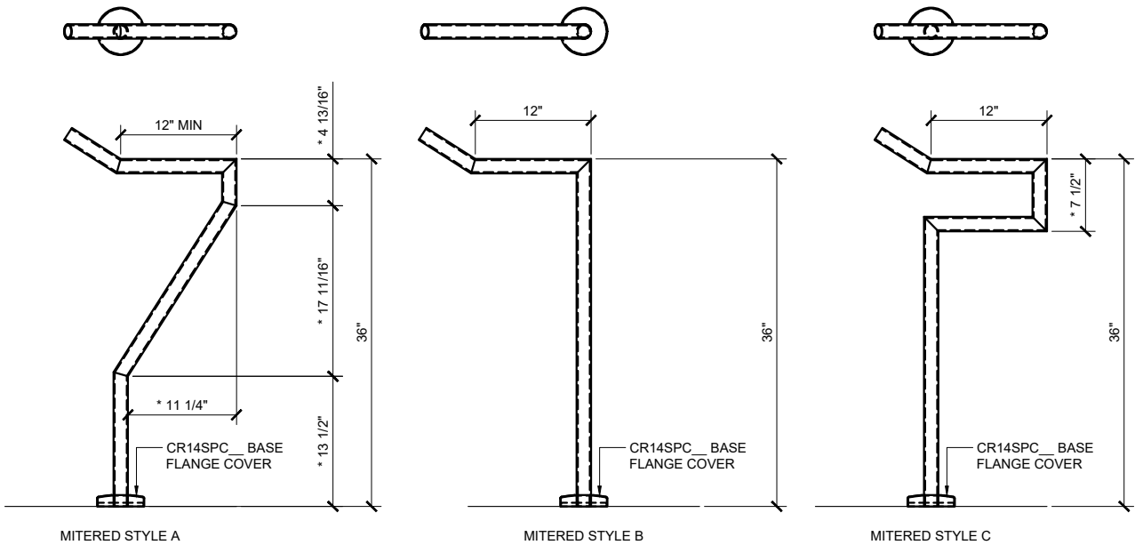
STANDARD FLOOR MOUNT CONFIGURATIONS WITH MITERED CORNERS
