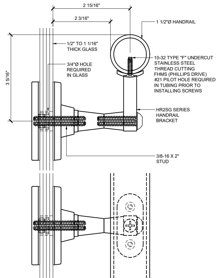
GLASS MOUNT HANDRAIL BRACKET HR2SG SERIES
