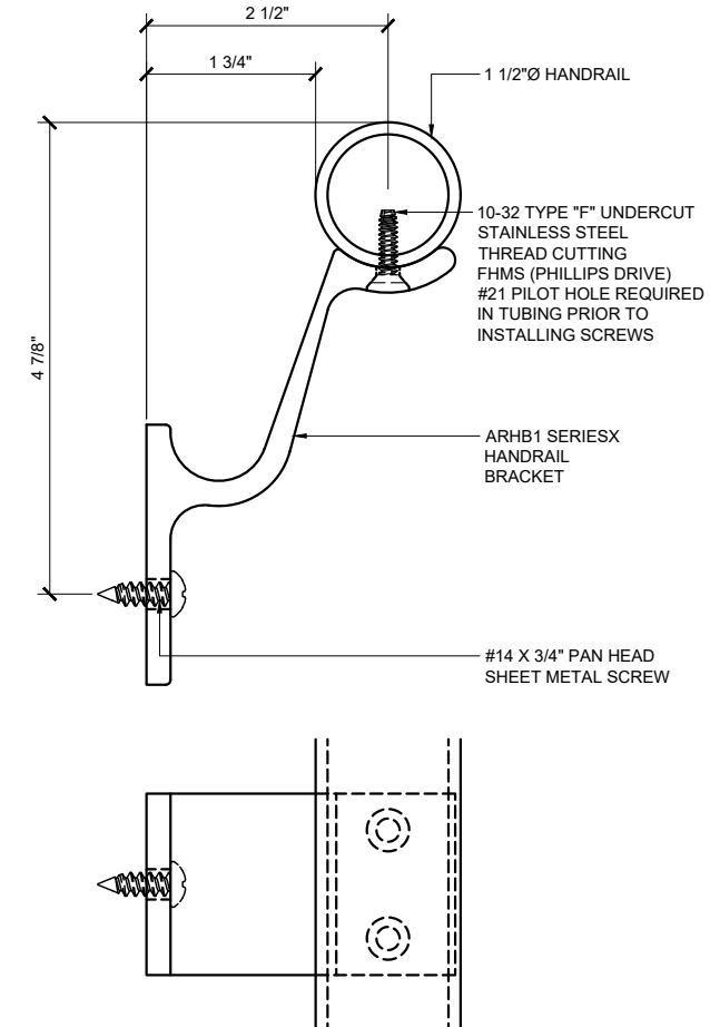
WALL MOUNT HANDRAIL BRACKET ARHB1 SERIES
