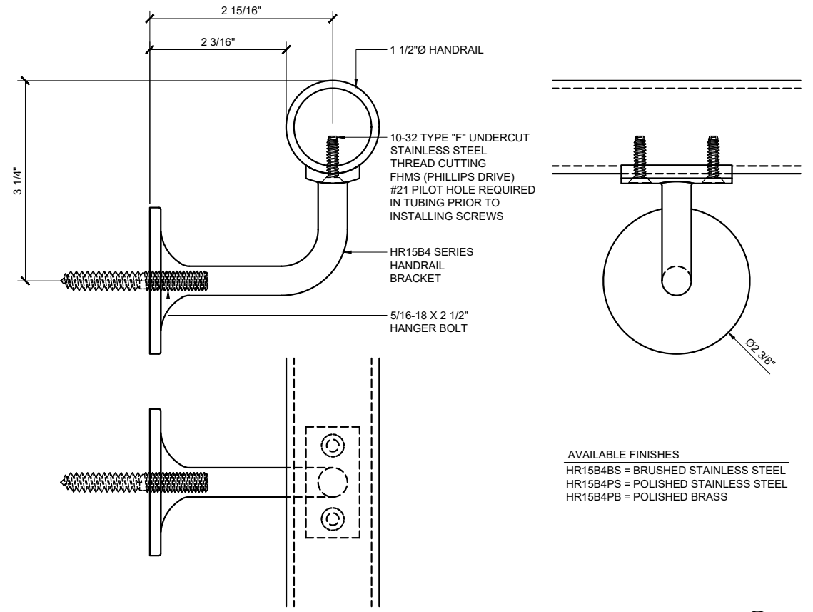
WALL MOUNT HANDRAIL BRACKET HR15B4 SERIES
