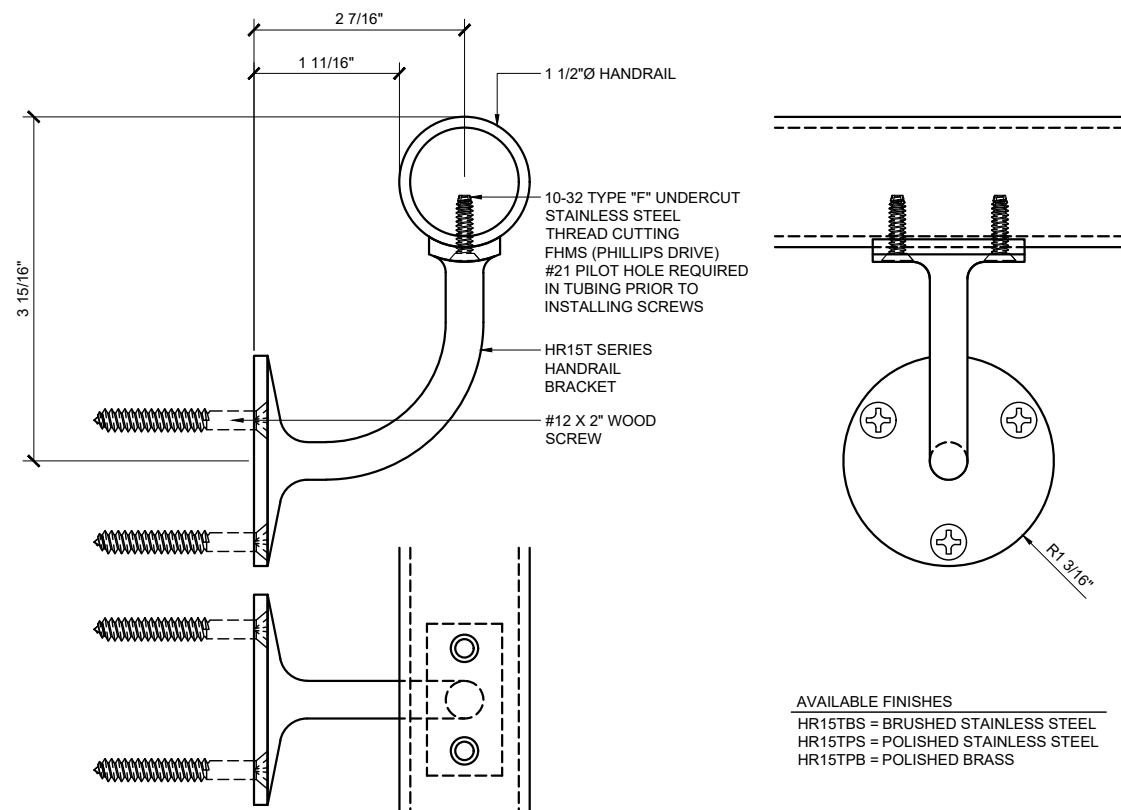
WALL MOUNT HANDRAIL BRACKET HR15T SERIES
