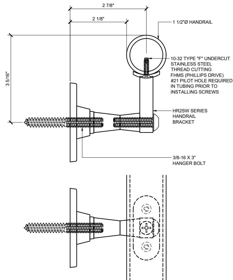
WALL MOUNT HANDRAIL BRACKET HR2SW SERIES
