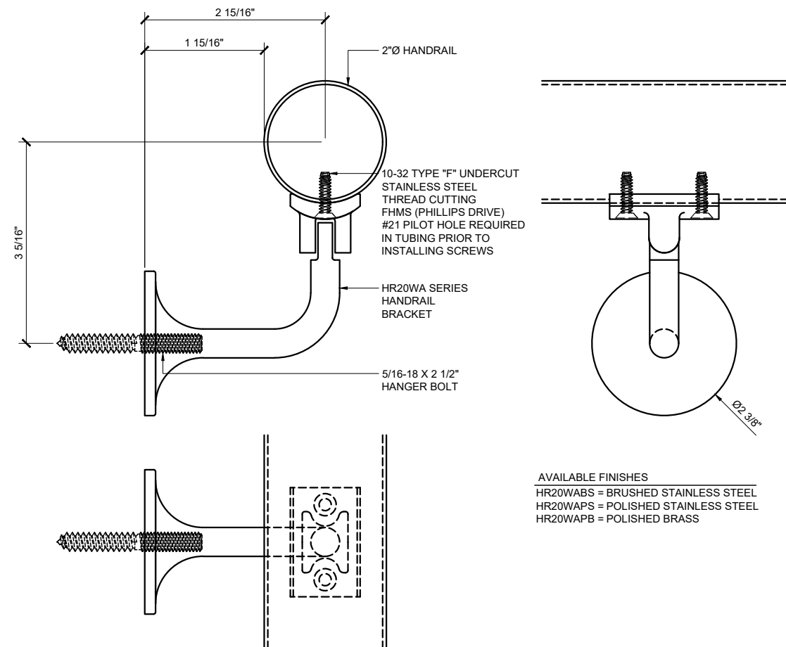
WALL MOUNT HANDRAIL BRACKET HR20WA SERIES
