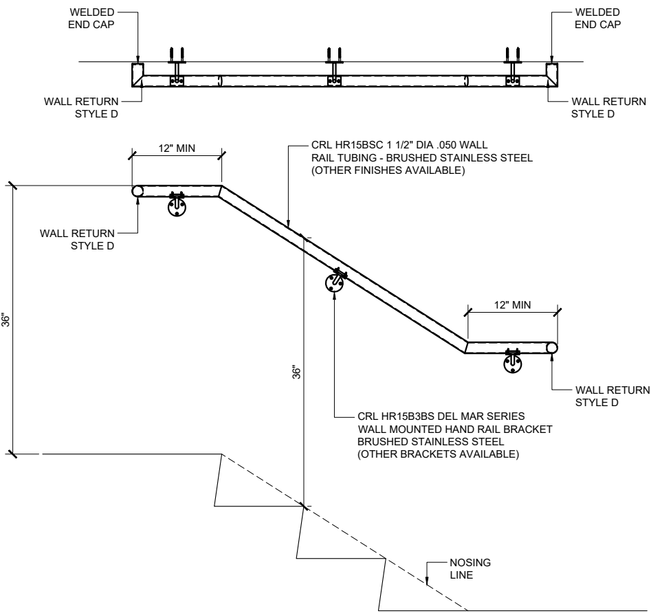
TYPICAL WALL-MOUNTED HANDRAIL WITH MITERED CORNERS
