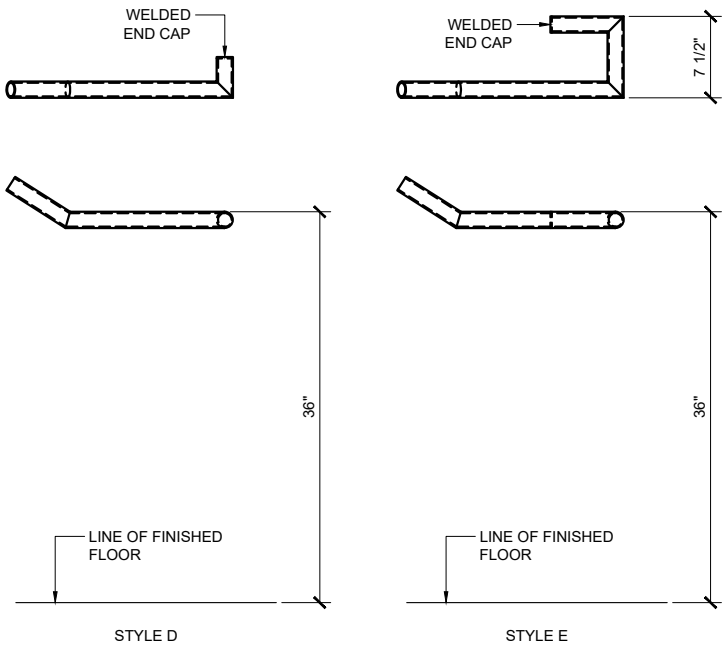
STANDARD WALL RETURN CONFIGURATIONS WITH MITERED CORNERS
