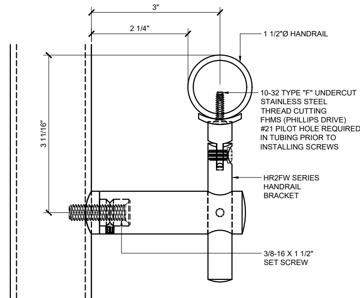
WALL MOUNT HANDRAIL BRACKET HR2FW SERIES
