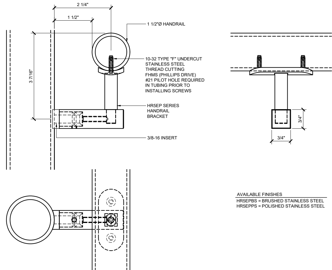
POST MOUNT HANDRAIL BRACKET HR5EP SERIES ②
