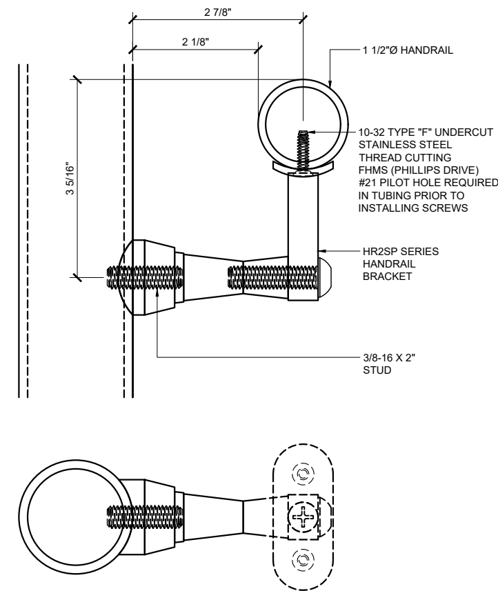
POST MOUNT HANDRAIL BRACKET HR2SP SERIES
