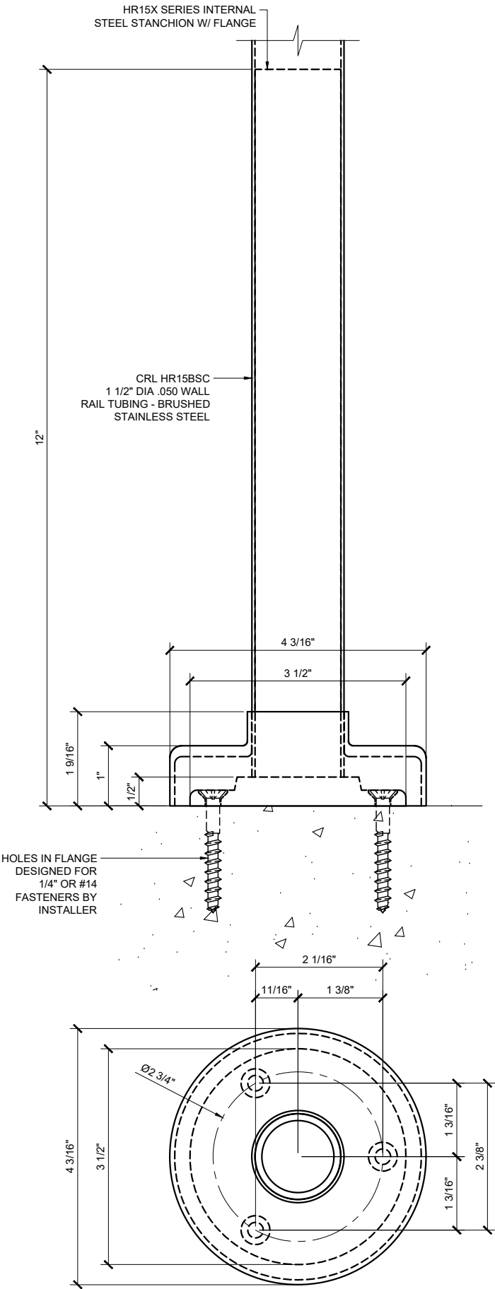
CONCRETE MOUNT
