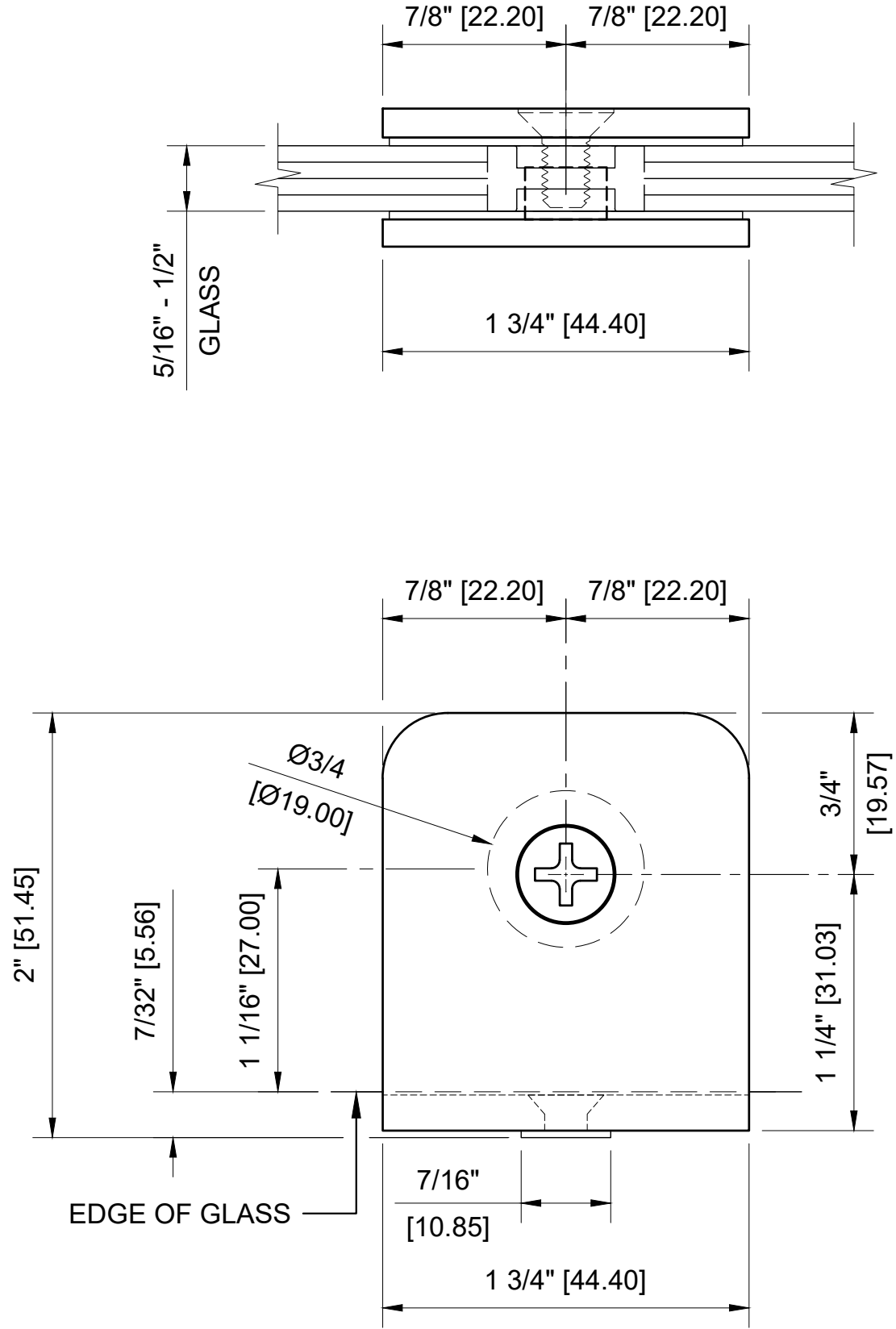
CRL - GCB186 TRADITIONAL MOVABLE WALL MOUNT TRANSOM CLAMP FOR 5/16" - 1/2" GLASS
