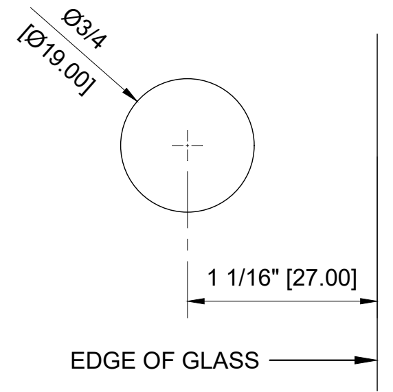
GLASS FABRICATION TEMPLATE
