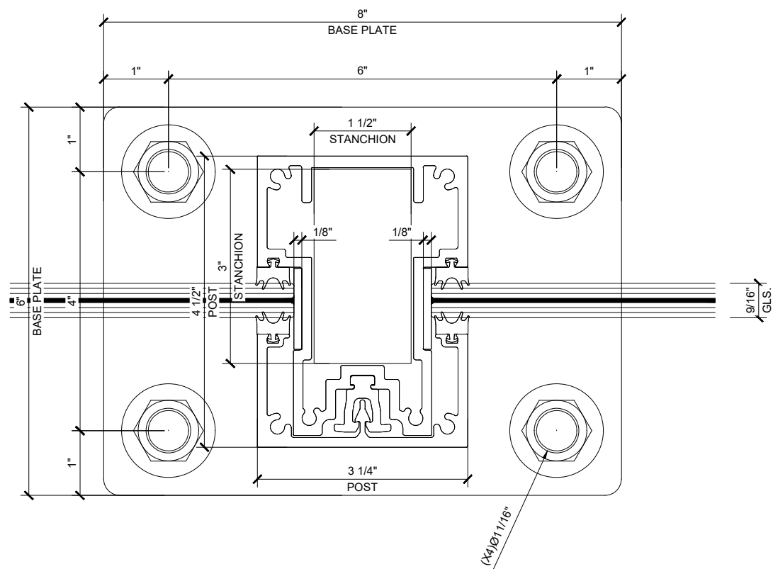
2 WINDSCREEN CENTER POST DETAIL ARCH REF: _____ SCALE: 1'-0"=1'-0"
