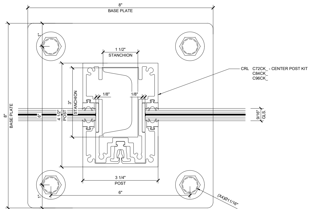
2 WINDSCREEN CENTER POST DETAIL
