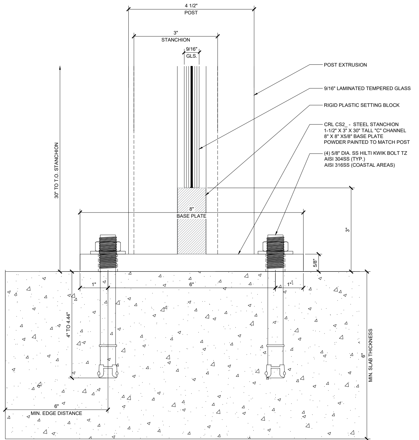
3 WINDSCREEN ANCHOR DETAIL
