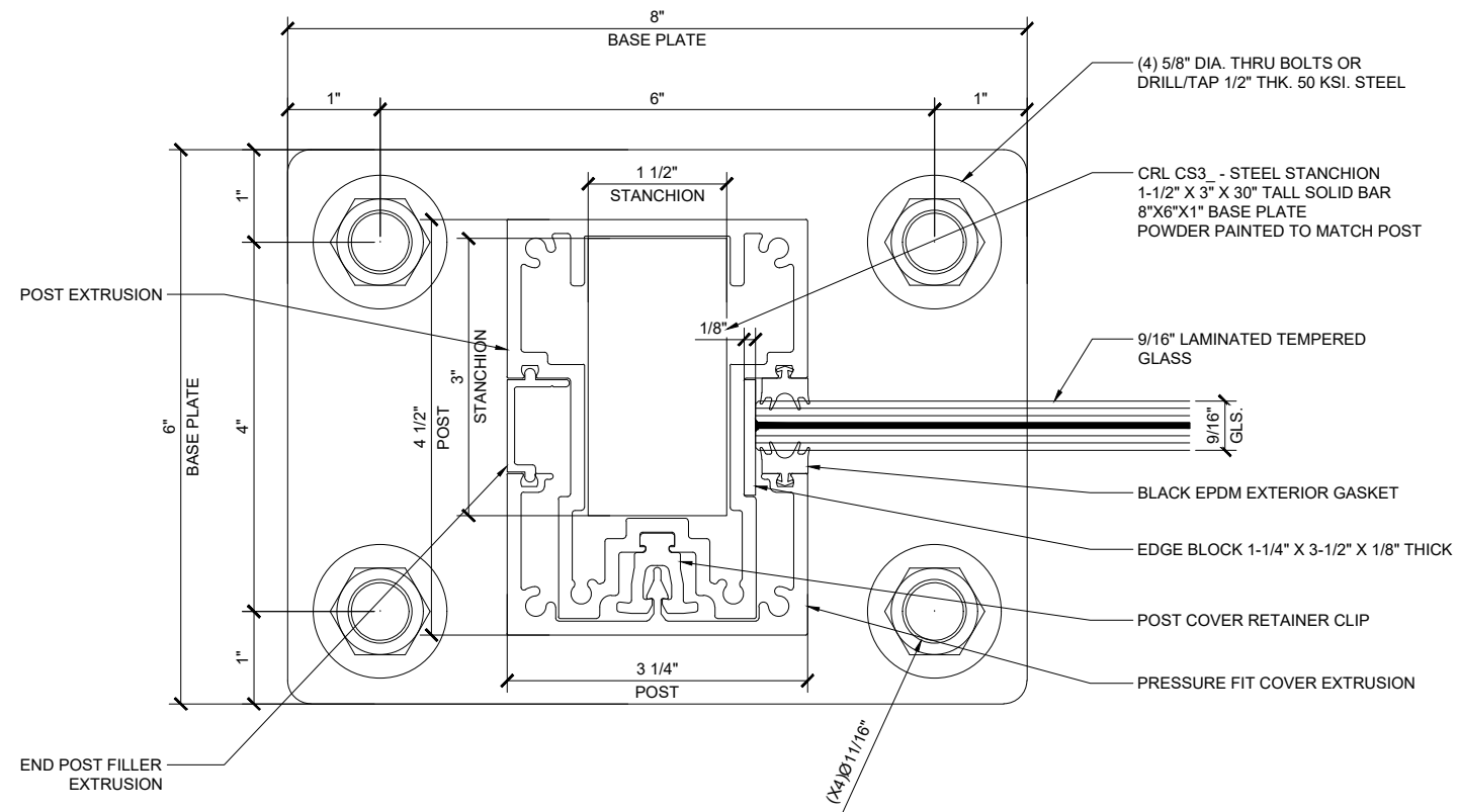
1 WINDSCREEN END POST DETAIL ARCH REF: _____ SCALE: 1'-0"=1'-0"
