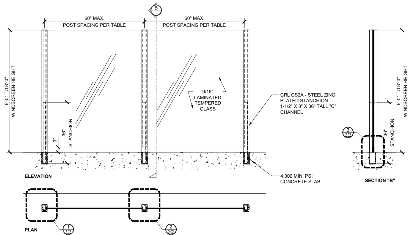
② TYP. WINDSCREEN (CORE MOUNT_CONCRETE)
