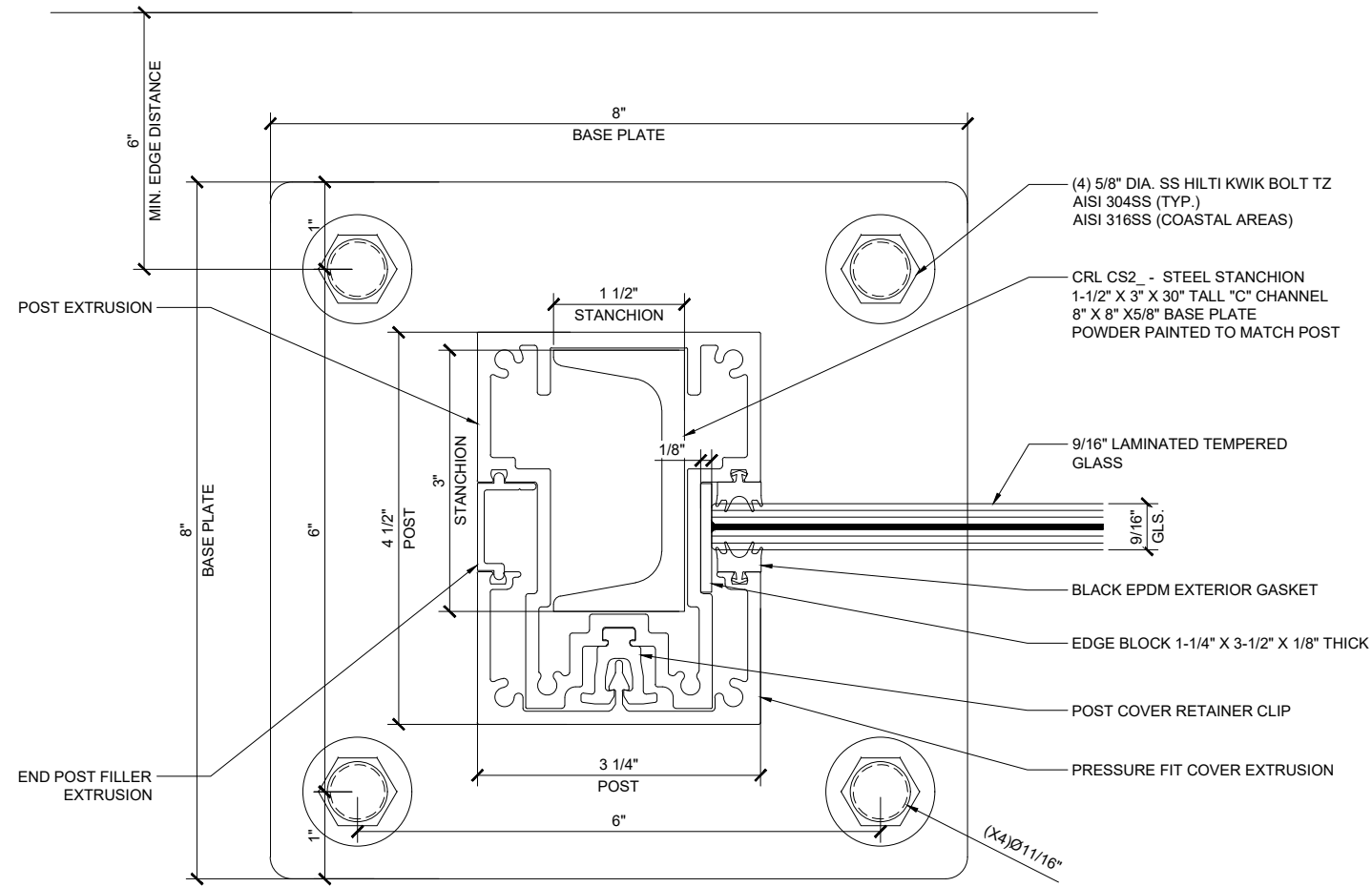
1 WINDSCREEN END POST DETAIL
