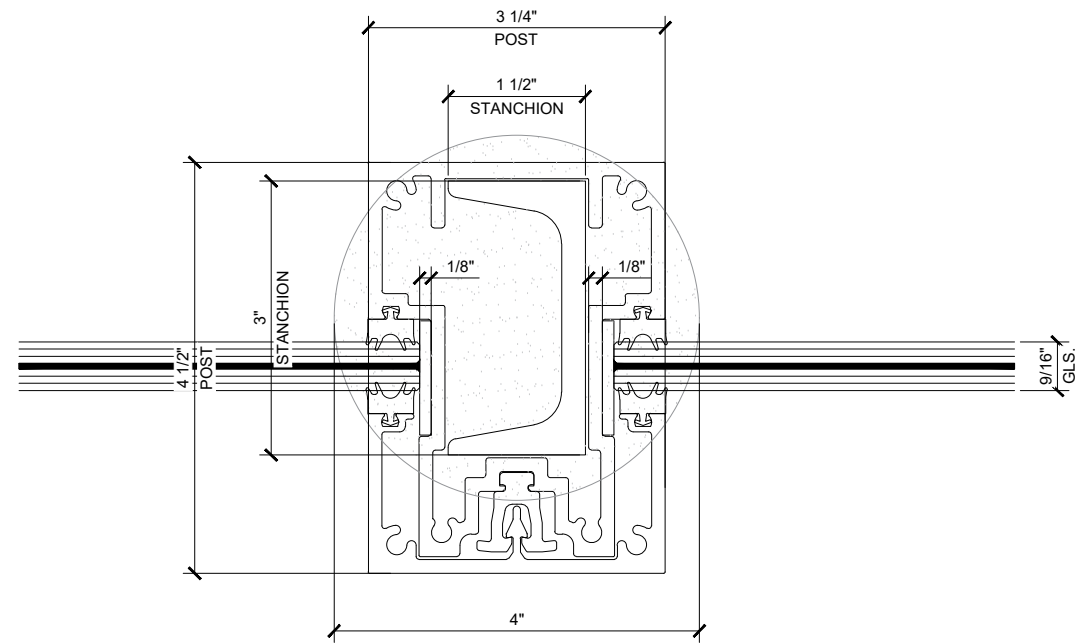
2 WINDSCREEN CENTER POST DETAIL ARCH REF: _____ SCALE: 1'-0"=1'-0"
