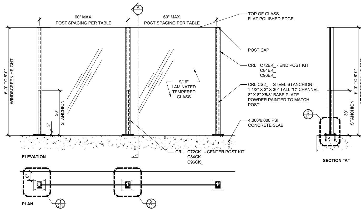
① TYP. WINDSCREEN (SURFACE MOUNT_CONCRETE)
