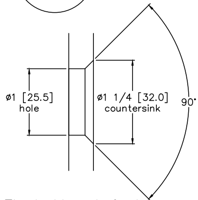
Flush Mount fastener fabrication
