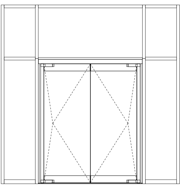
1 Balancer Double Elevation Exposed 3/4" = 1'-0"
