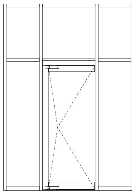
2 Balancer Single Elevation Exposed 3/4" = 1'-0"
