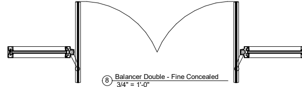
8 Balancer Double - Fine Concealed 3/4" = 1'-0"
