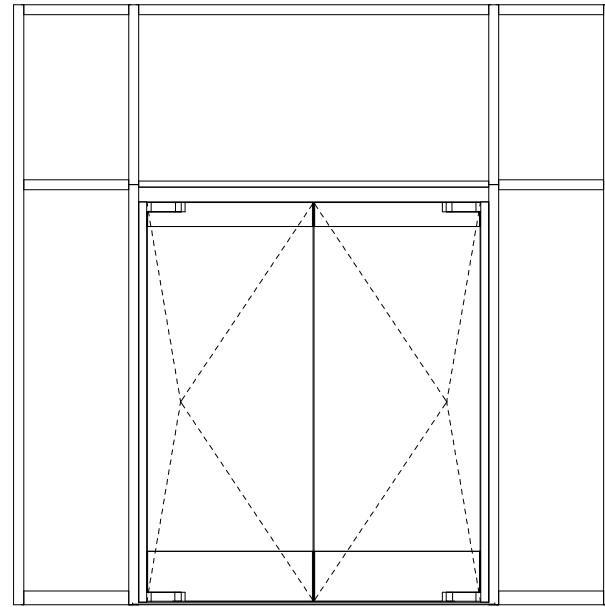
2 Balancer Double Elevation Concealed 3/4" = 1'-0"
