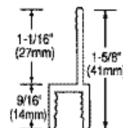
Top Rail for 3/8" (10mm) Glass
