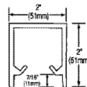
Header for 1/4" (6mm) Glass
