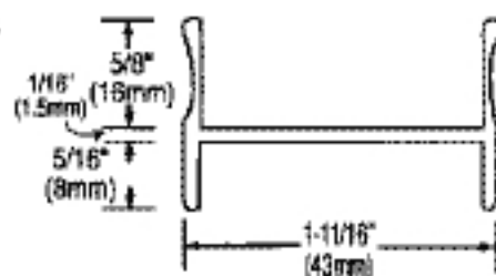
Side Jamb for 3/8" (10mm) or 1/4" (6mm) Glass
