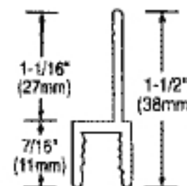
Top Rail for 1/4" (6mm) Glass
