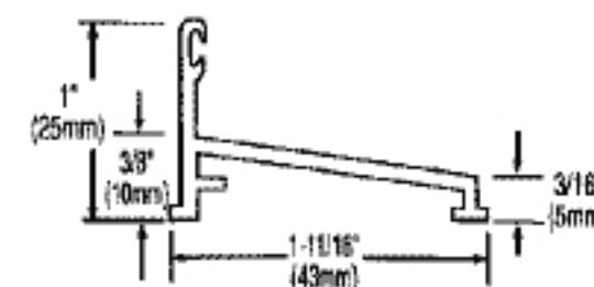
Bottom Track for 3/8" (10mm) or 1/4" (6mm) Glass
