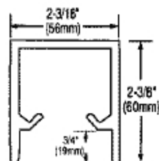
Header for 3/8" (10mm) Glass
