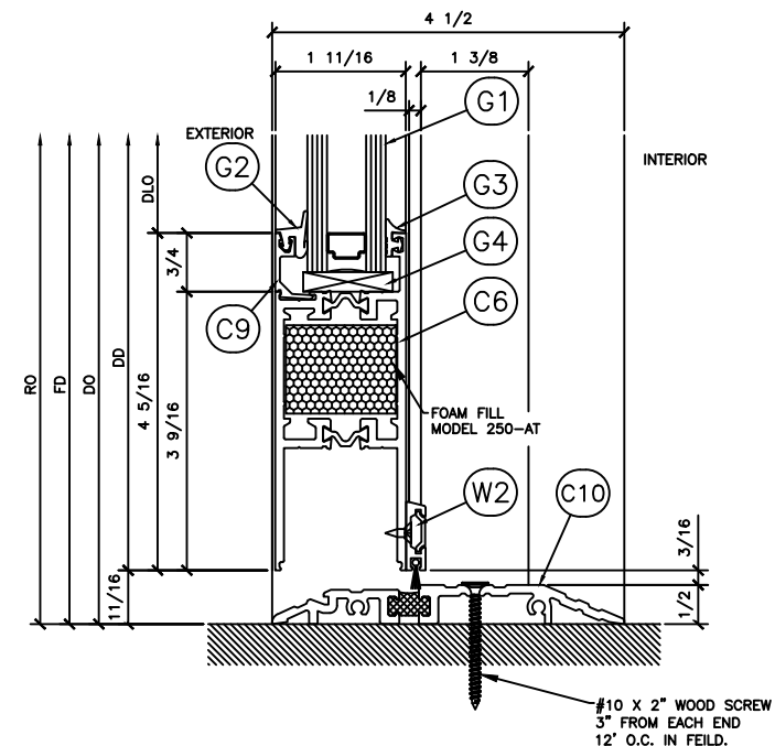
④ SECTION DETAIL @ 4 5/16" DOOR SILL SCALE: FULL SIZE
