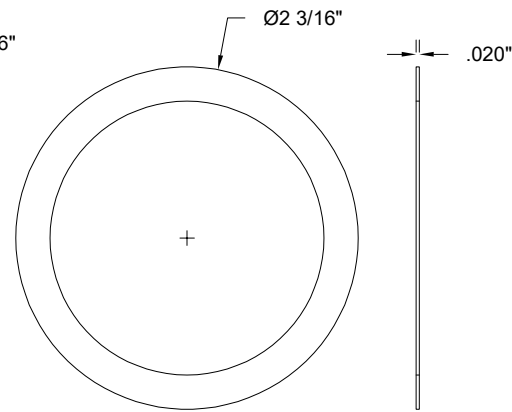
GASKET X2
