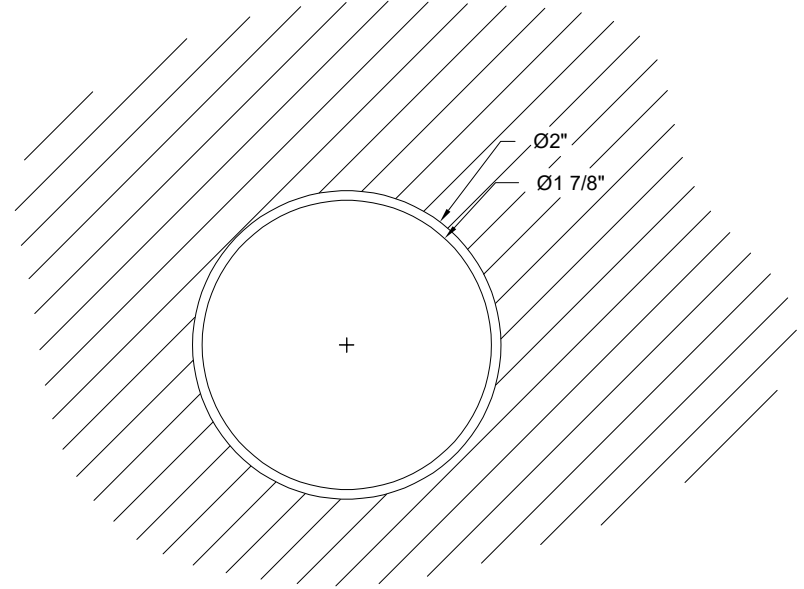
GLASS CUTOUT
