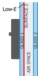
Double Pane Window
