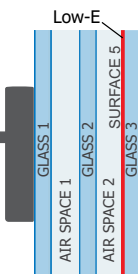
Triple Pane Window
