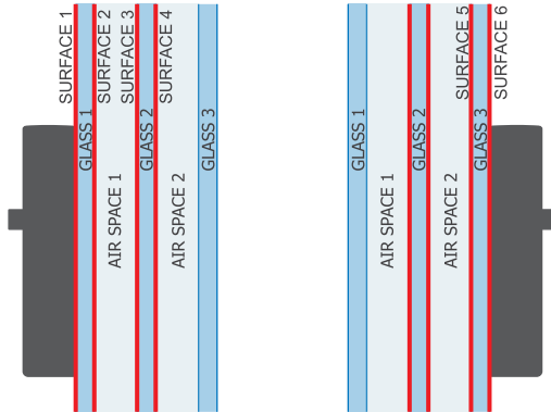
Triple Pane Window
