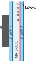
Double Pane Window
