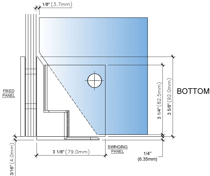
2B FRONT VIEW DETAIL - 4MM FIXED PANEL GAP ARCH REF: SCALE: 1'-0\"/>
