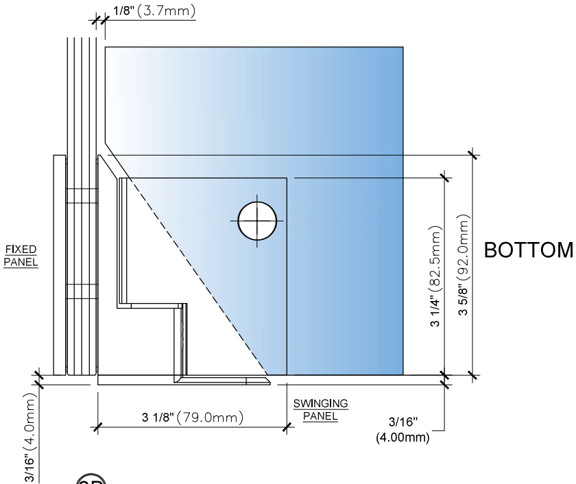
2B FRONT VIEW DETAIL - 4MM FIXED PANEL GAP
