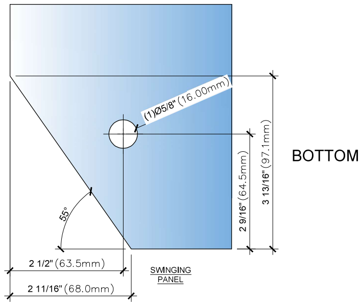
3B GLASS CUT OUT DETAIL - 4MM FIXED PANEL GAP
