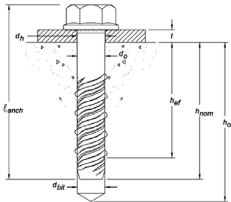
FIGURE 1—WEDGE-BOLT+ ANCHOR DETAIL
