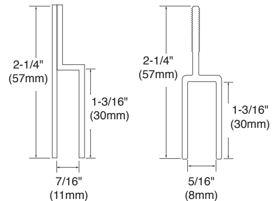
Top Hanger for 3/8" (10mm) Glass
