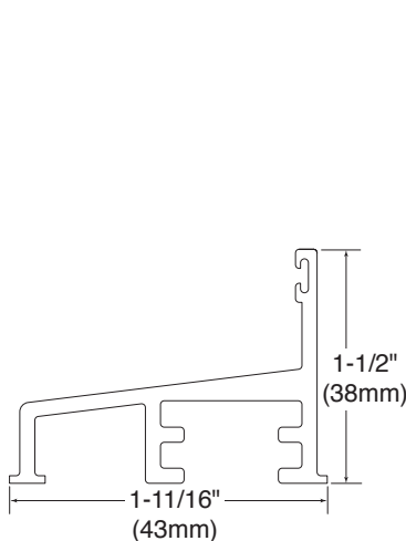
Bottom Track for 3/8" (10mm) or 1/4" (6mm) Glass
