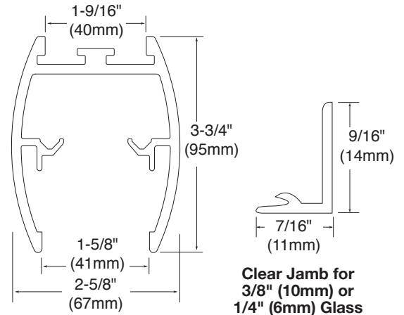
Header for 3/8" (10mm) Glass or 1/4" (6mm) Glass
