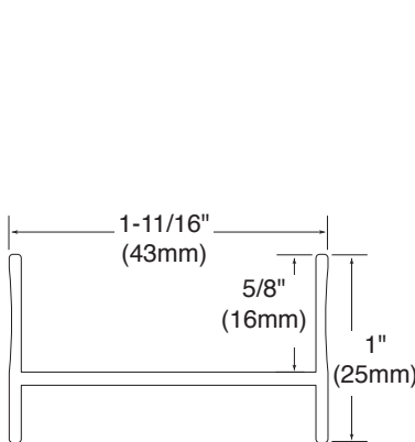
Side Jamb for 3/8" (10mm) or 1/4" (6mm) Glass
