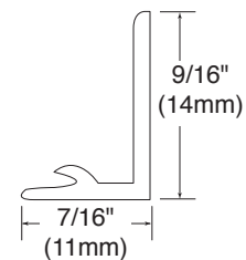
Clear Jamb for 3/8" (10mm) or 1/4" (6mm) Glass
