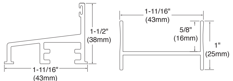
Bottom Track for 3/8" (10mm) or 1/4" (6mm) Glass
