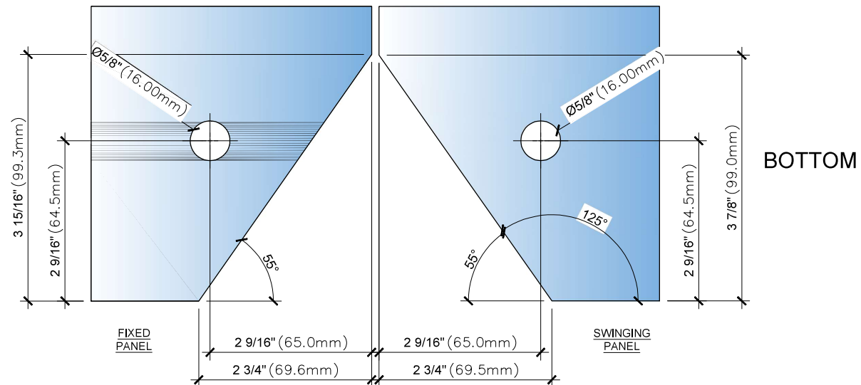
3B GLASS CUT OUT DETAIL - 4MM FIXED PANEL GAP ARCH REF: SCALE: 1'-0"=1'-0"
