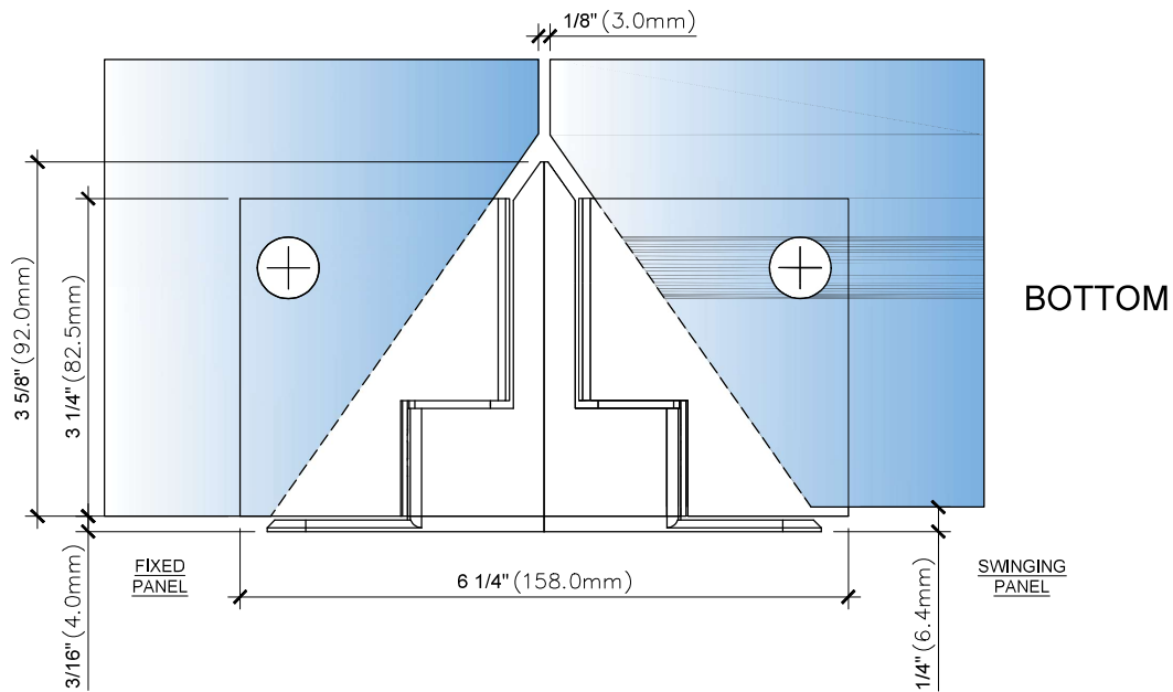
2B FRONT VIEW DETAIL - 4MM FIXED PANEL GAP
