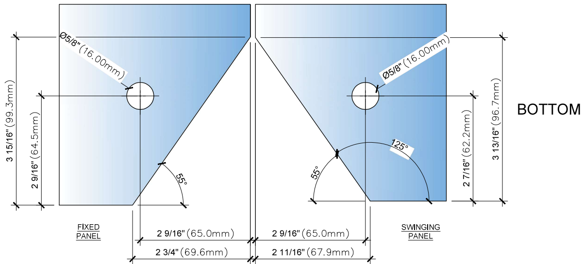
3B GLASS CUT OUT DETAIL - 4MM FIXED PANEL GAP
