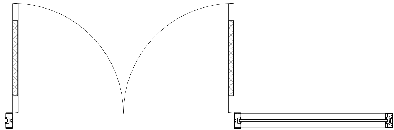
1 FINE - DOUBLE 3/4" = 1'-0"
