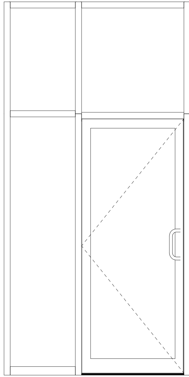
12 NORTH 3/4" = 1'-0"
