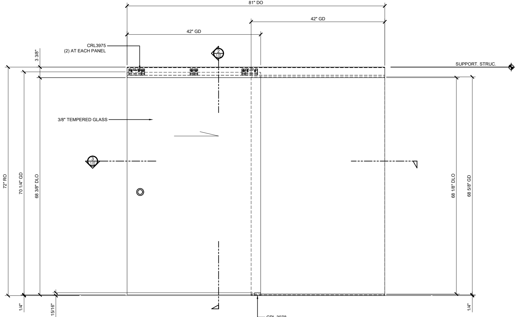
① CRL2812F AND CRL 28512F - ELEVATION
