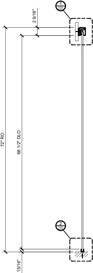
② SLIDER SECTION
