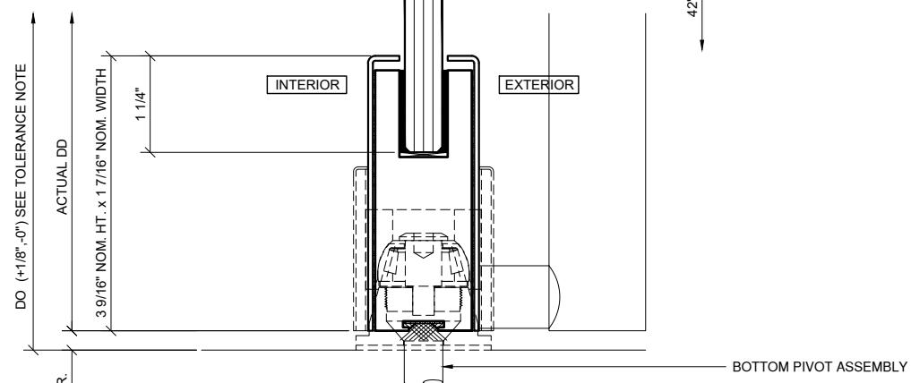
3 SECTION AT DOOR SILL
