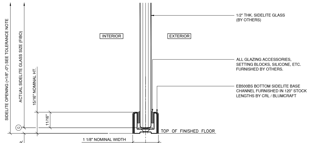
5 SECTION AT SIDELITE SILL
