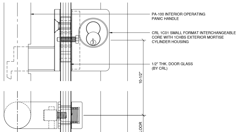
2 SECTION AT DOOR PULL
