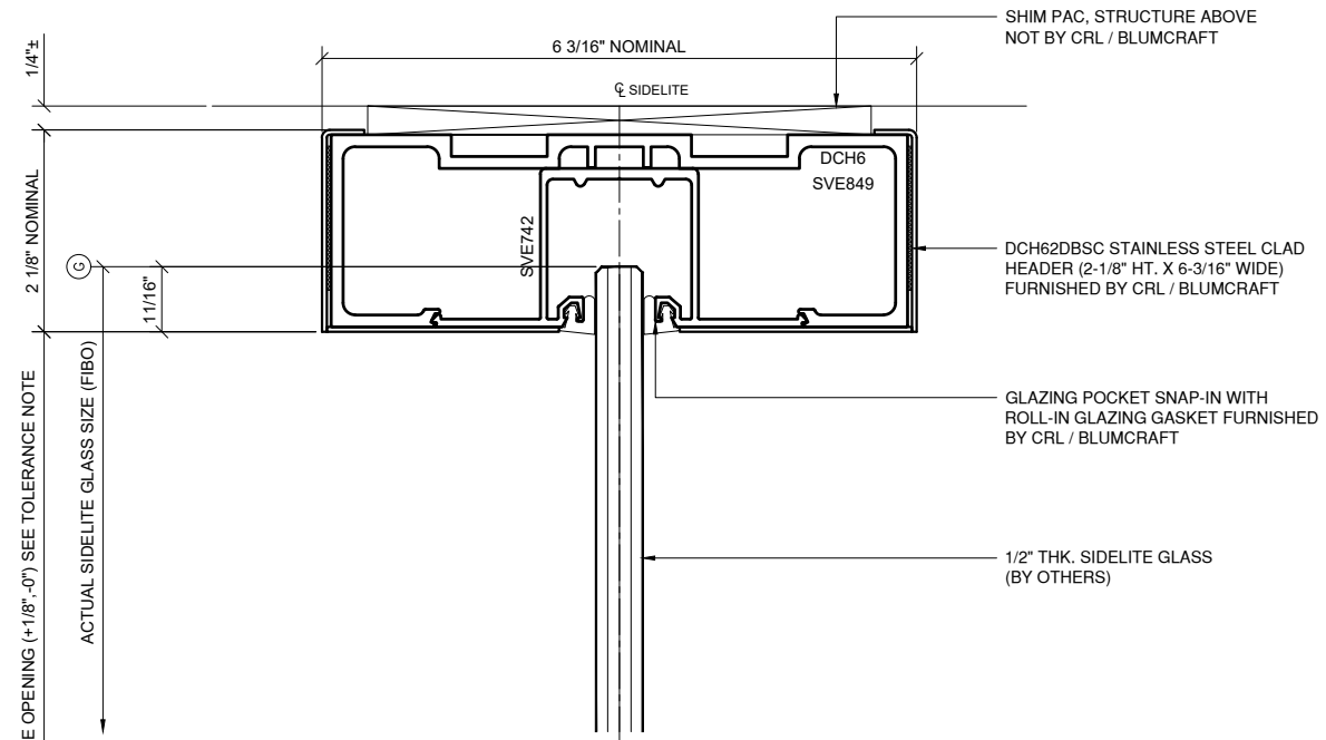
4 SECTION AT SIDELITE HEAD
