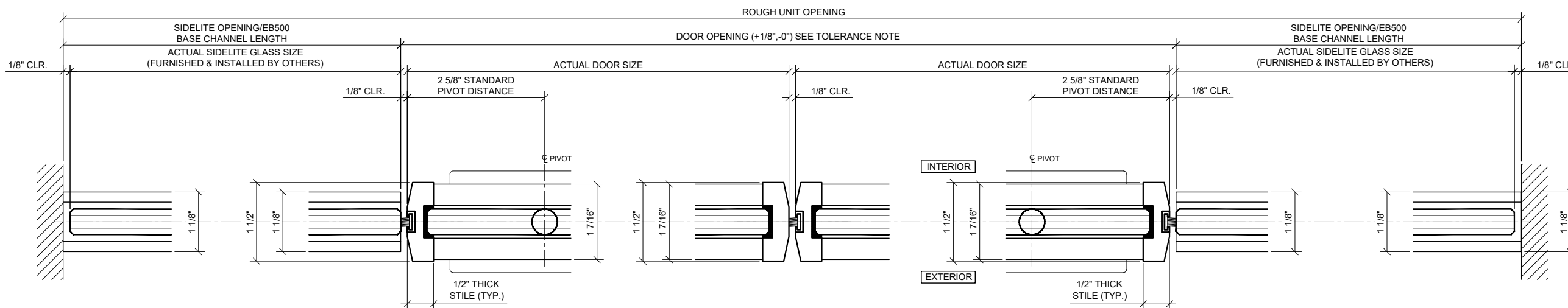
1A PLAN: WALL TO SIDE LITE
