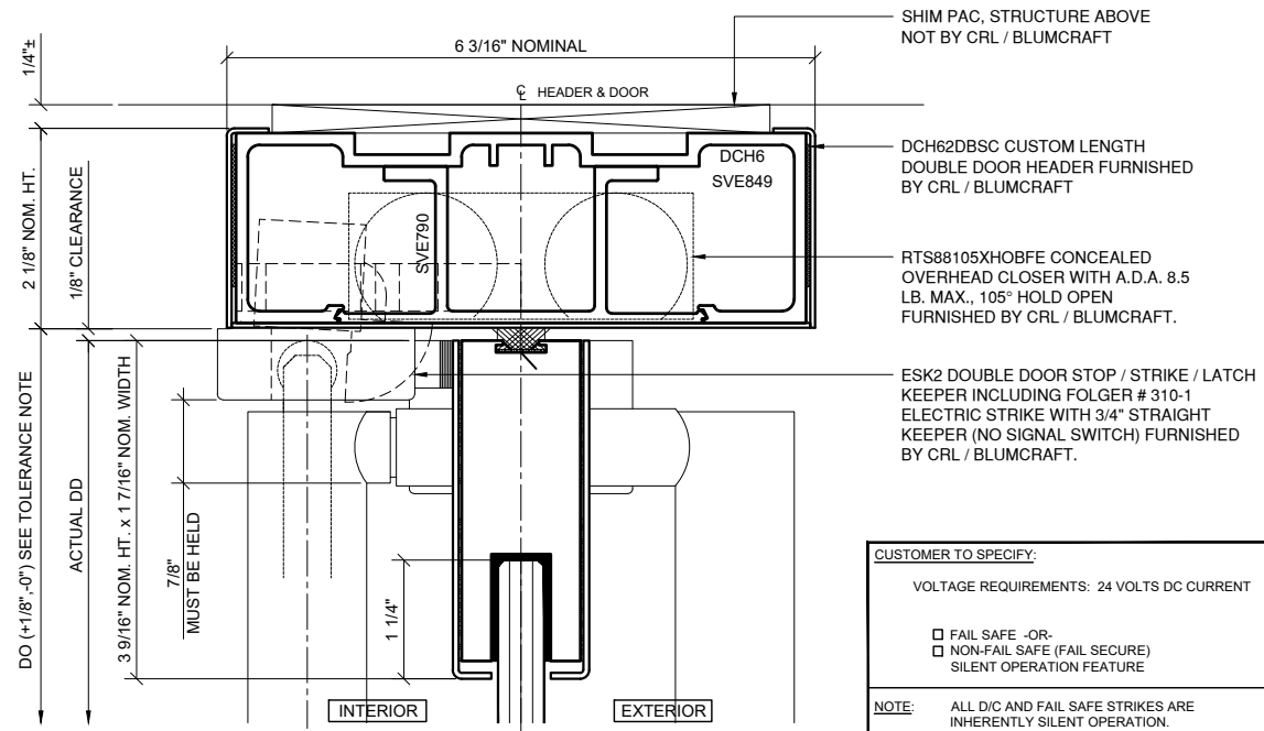
1 SECTION AT DOOR HEAD
