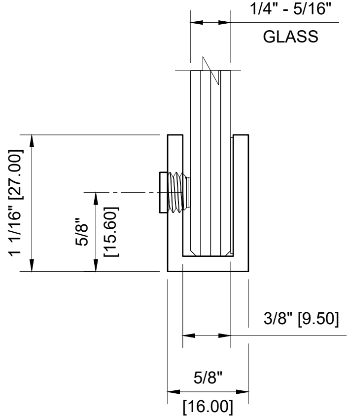
CRL EH36 - BRASS FINISH DOUBLE SET SCREW GLASS CLAMP
