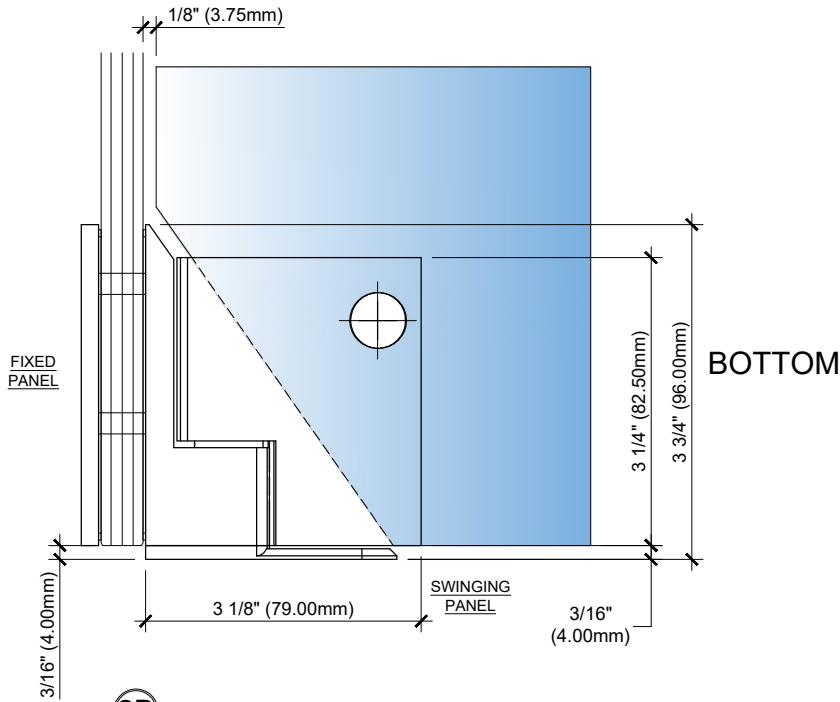
2B FRONT VIEW DETAIL - 4MM FIXED PANEL GAP
