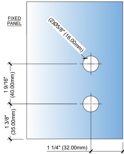
3B GLASS CUT OUT DETAIL - 4MM FIXED PANEL GAP
