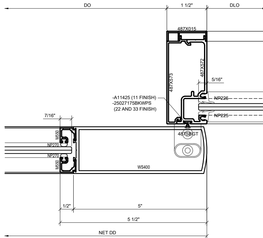
② SERIES 487 OPS INTEGRATED SLIDER INTERMEDIATE JAMB DETAIL (CLOSED) 1'-0"=1'-0" ARCH REF: N/A
