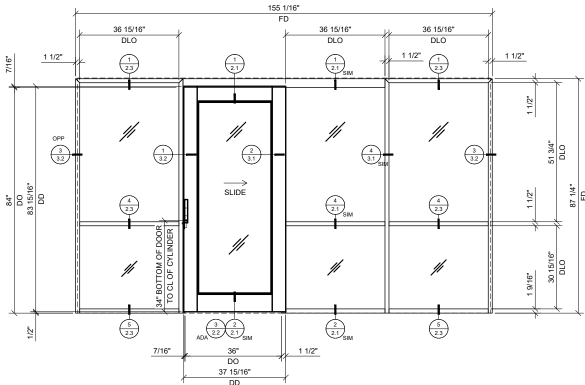
3 SINGLE SLIDER WITH BAY & SIDELITE AT BOTH ENDS 3/4"=1'-0"
