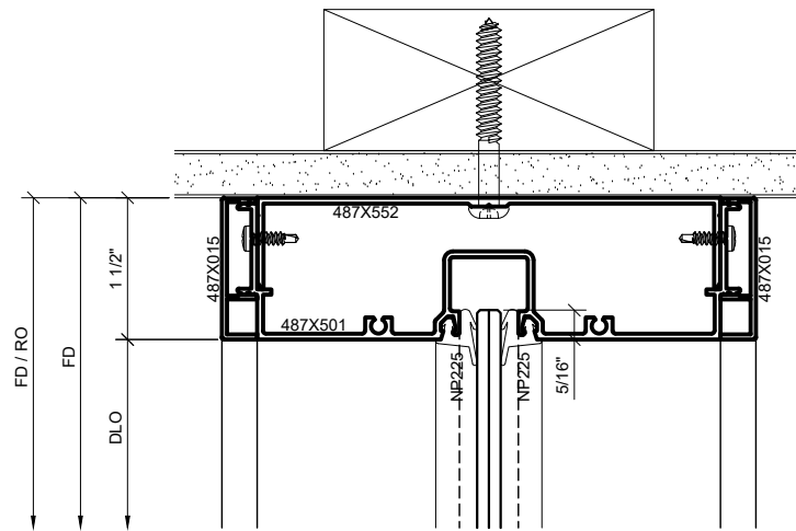
② SERIES 487 OPS SURFACE MOUNT HEAD DETAIL AT SIDELITE (NO SHIM) 1'-0\"/>
