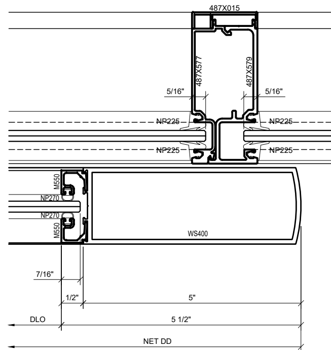
⑤ SERIES 487 OPS INTEGRATED SLIDER SHALLOW VERTICAL DETAIL (OPEN) 1'-0"=1'-0" ARCH REF: N/A
