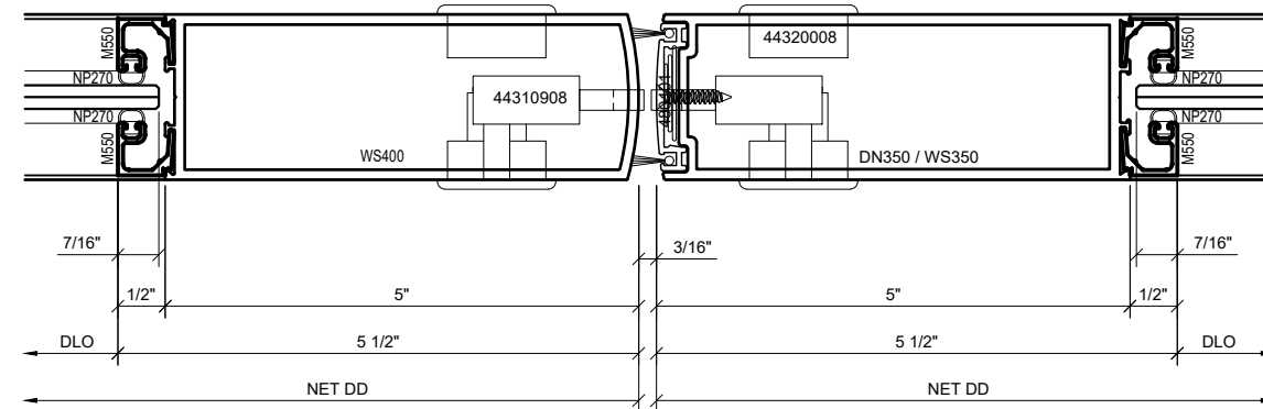
⑥ SERIES 487 OPS INTEGRATED SLIDER MEETING STILES AT DOOR PAIR DETAIL 1'-0"=1'-0" ARCH REF: N/A
