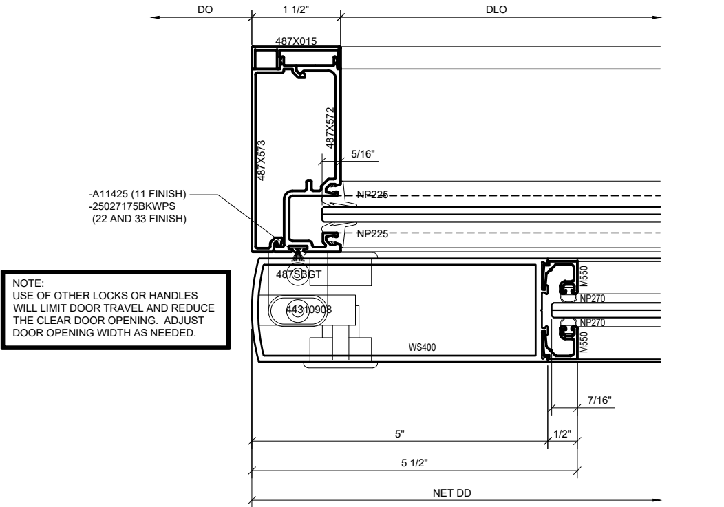
② SERIES 487 OPS INTEGRATED SLIDER TRANSITION VERTICAL-STANDARD TO INTERMEDIATE JAMB DETAIL (OPEN) 1'-0"=1'-0" ARCH REF: N/A
