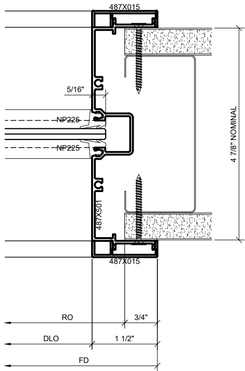
③ SERIES 487 OPS STANDARD JAMB DETAIL 1'-0"=1'-0" ARCH REF: N/A
