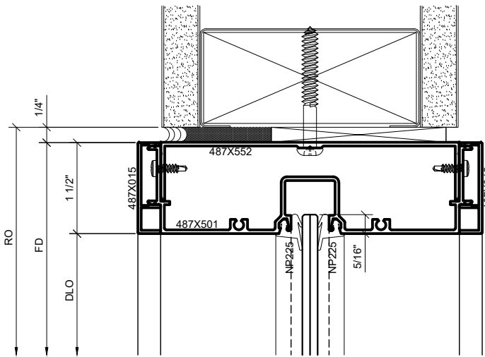
① SERIES 487 OPS SURFACE MOUNT HEAD DETAIL AT SIDELITE (w/ SHIM) 1'-0\"/>
