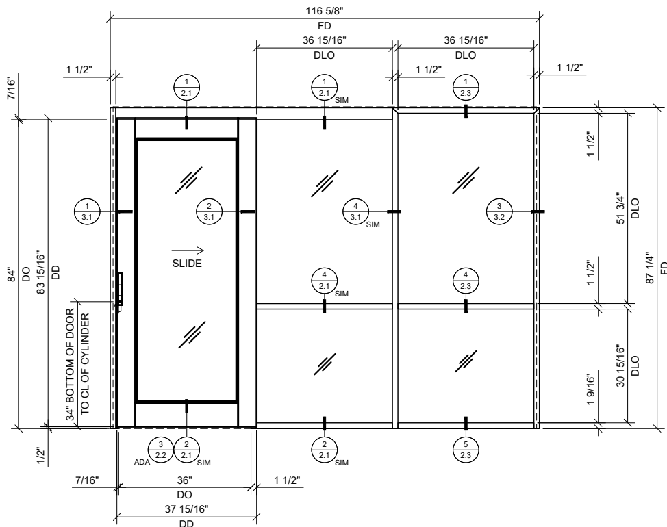
1 SINGLE SLIDER WITH BAY & SIDELITE 3/4"=1'-0"
