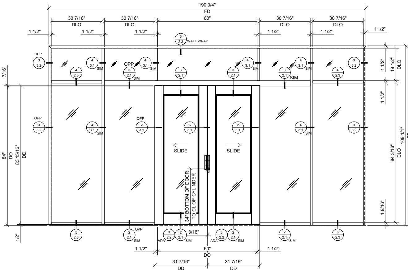
4 BI-PART SLIDER WITH BAY, TRANSOM & SIDELITES AT EACH END 3/4"=1'-0" ARCH REF: N/A
