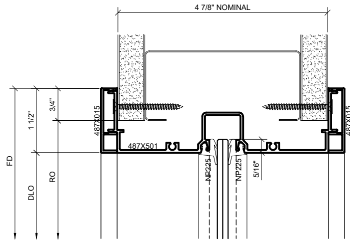
③ SERIES 487 OPS WALL-WRAPPED TRANSOM HEAD DETAIL AT INT. VERTICAL 1'-0\"/>
