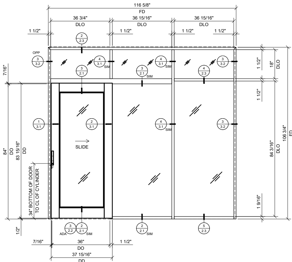
2 SINGLE SLIDER WITH BAY, TRANSOM & SIDELITE 3/4"=1'-0"
