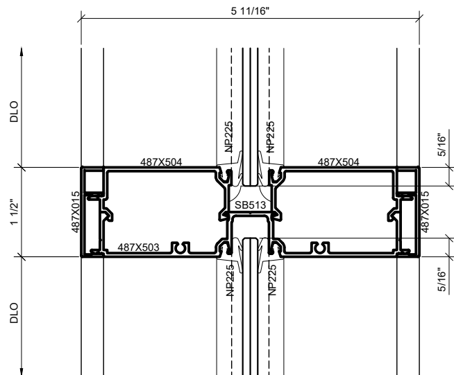
④ SERIES 487 OPS TYP HORIZONTAL DETAIL 1'-0\"/>
