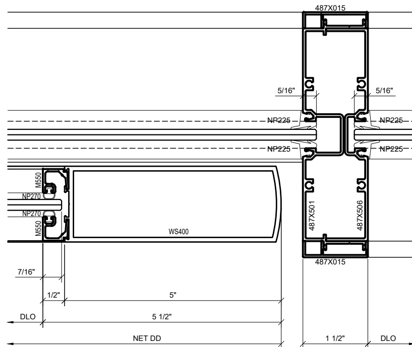
④ SERIES 487 OPS INTEGRATED SLIDER TRANSITION VERTICAL-SLIDER TO STANDARD (OPEN) 1'-0"=1'-0" ARCH REF: N/A
