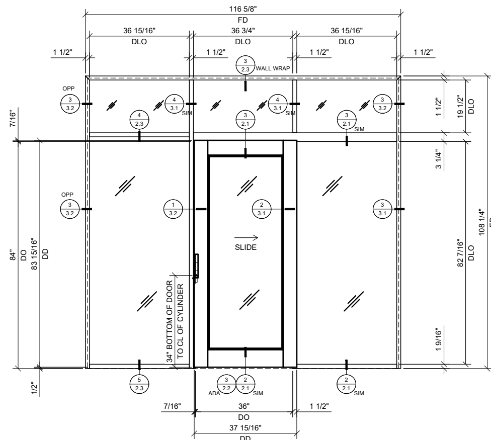
4 SINGLE SLIDER WITH BAY, TRANSOM & SIDELITE 3/4"=1'-0" ARCH REF: N
