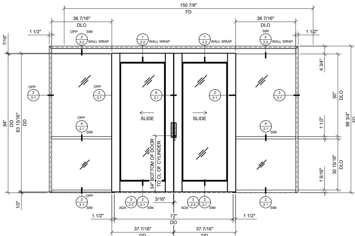
1 BI-PART SLIDER WITH BAYS 3/4"=1'-0" ARCH REF: N/A
