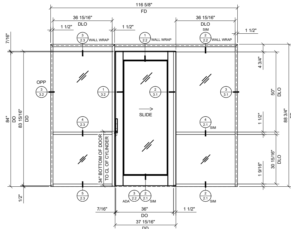
3 SINGLE SLIDER WITH BAY & SIDELITE 3/4"=1'-0" ARCH REF: N
