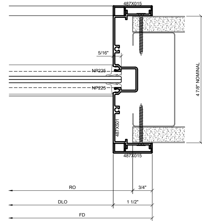
③ SERIES 487 OPS INTEGRATED SLIDER WALL JAMB DETAIL 1'-0"=1'-0" ARCH REF: N/A
