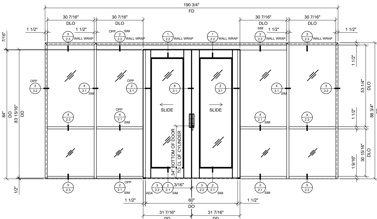
3 BI-PART SLIDER WITH BAY & SIDELITES AT EACH END 3/4"=1'-0" ARCH REF: N/A
