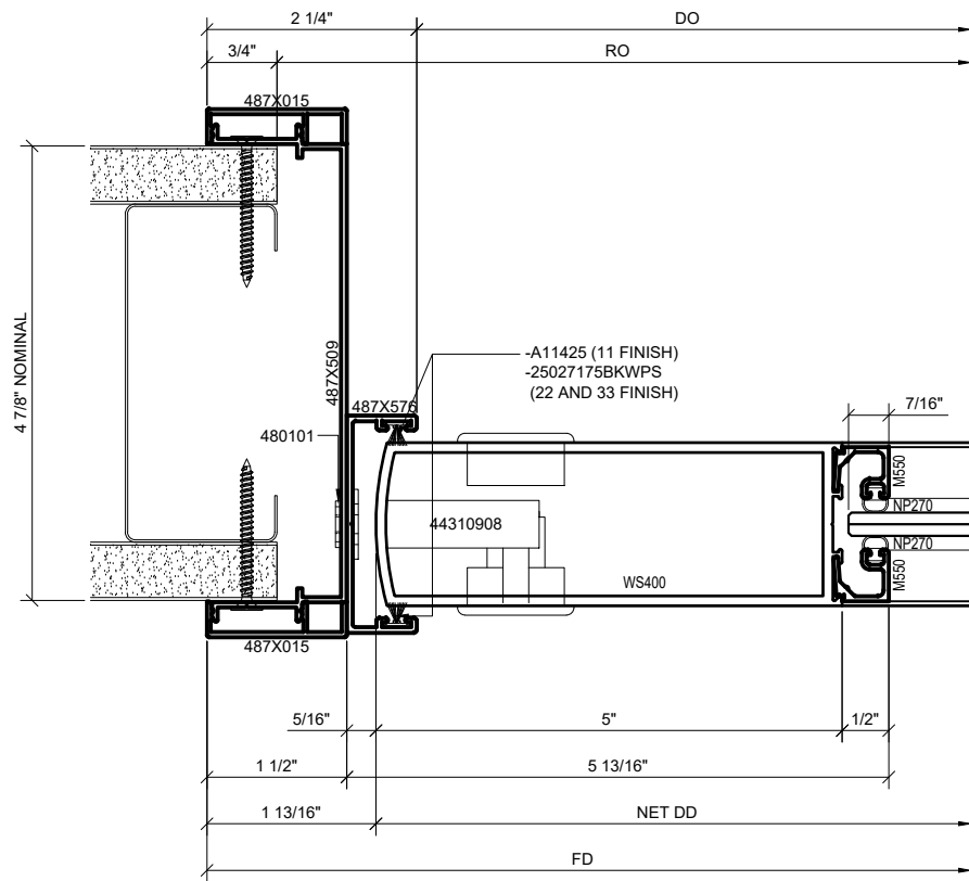
① SERIES 487 OPS INTEGRATED SLIDER STRIKE JAMB DETAIL (CLOSED) 1'-0"=1'-0" ARCH REF: N/A
