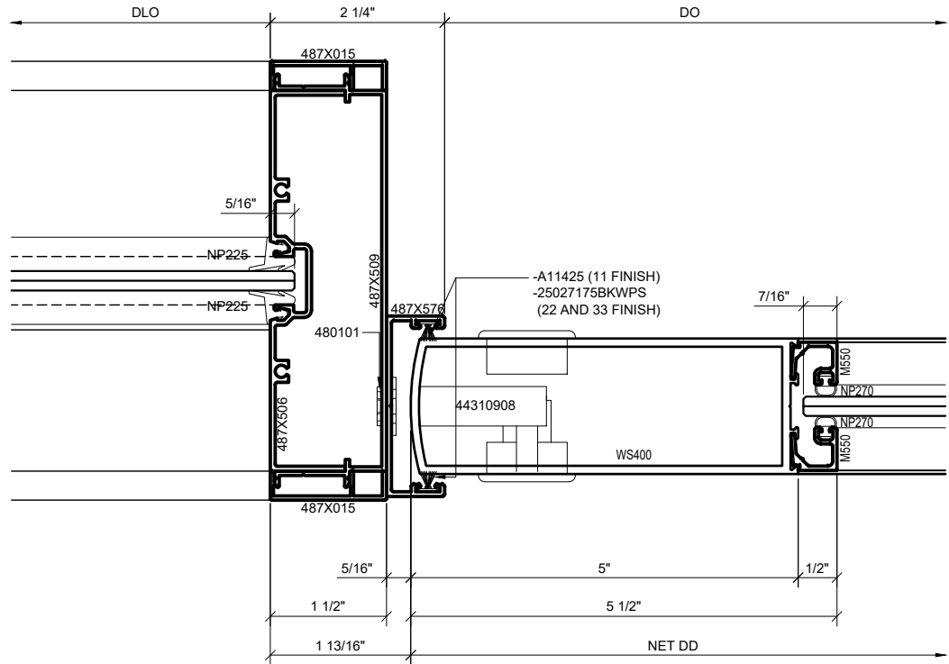
① SERIES 487 OPS INTEGRATED SLIDER TRANSITION VERTICAL-STANDARD TO STRIKE JAMB (CLOSED) 1'-0"=1'-0" ARCH REF: N/A
