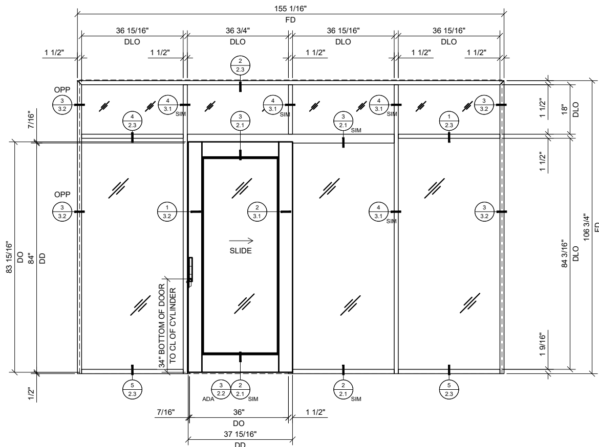
4 SINGLE SLIDER WITH BAY, TRANSOM & SIDELITE AT EACH END 3/4"=1'-0"
