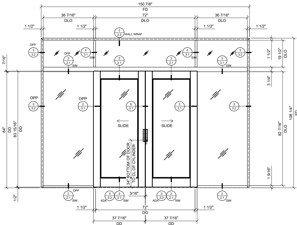
2 BI-PART SLIDER WITH BAYS & TRANSOM 3/4"=1'-0" ARCH REF: N/A
