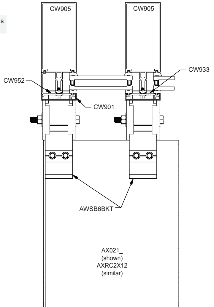
PLAN VIEW
