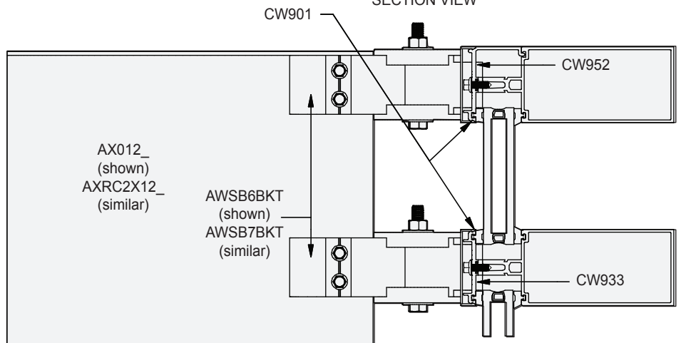
SECTION VIEW
