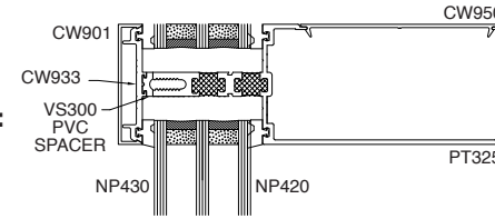
TYPICAL DETAILS:
