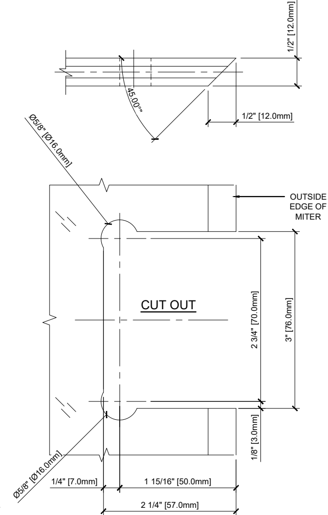
1/2" GLASS FABRICATION TEMPLATE FIXED PANEL
