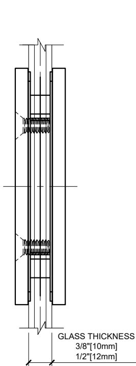
1/2" GLASS FABRICATION TEMPLATE FIXED PANEL
