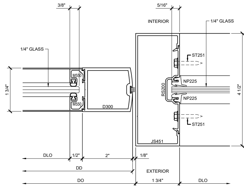
SECTION DETAIL @ DOOR JAMB
