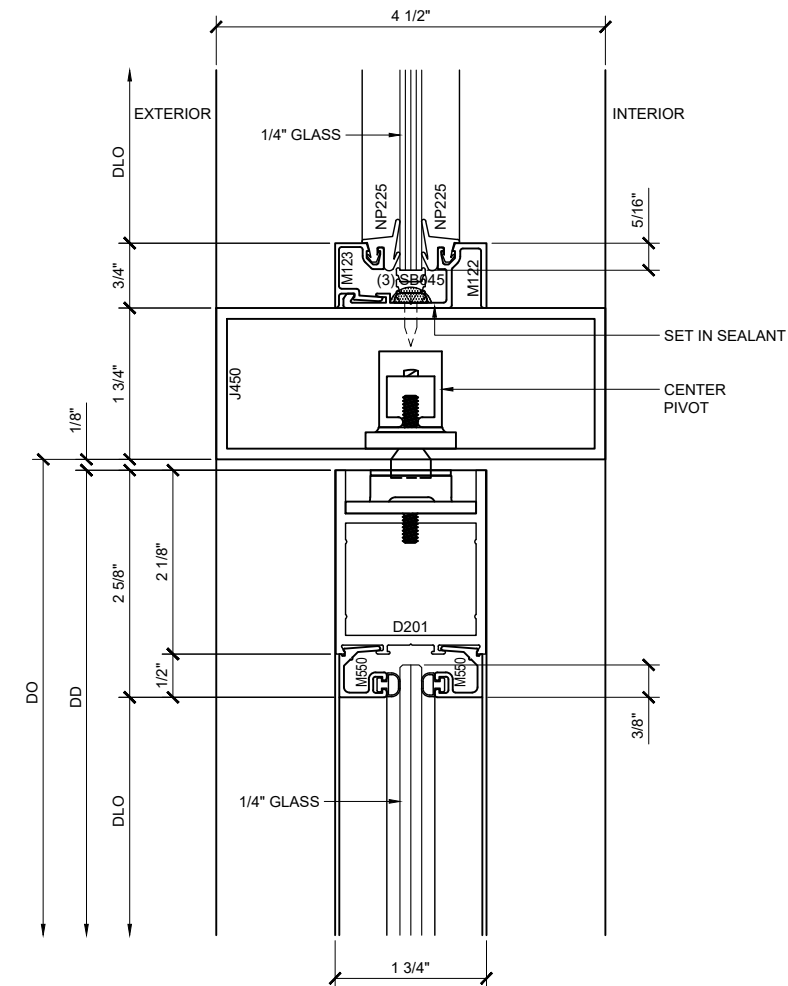
SECTION DETAIL @ DOOR HEAD WITH PIVOT ②
