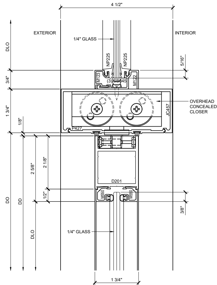
SECTION DETAIL @ DOOR HEAD WITH OHCC ③
