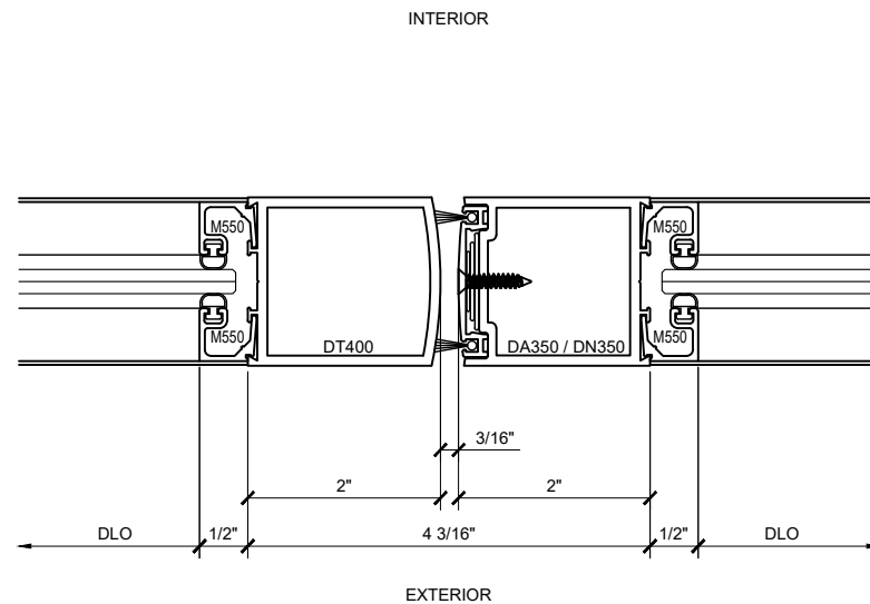
SECTION DETAIL @ MEETING STILES 9
