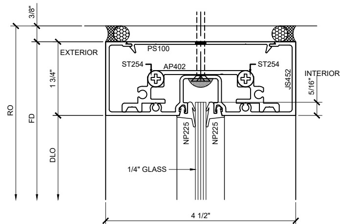
SECTION DETAIL @ STOREFRONT HEAD ①
