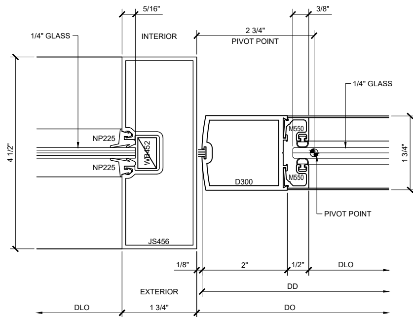
SECTION DETAIL @ DOOR JAMB 8
