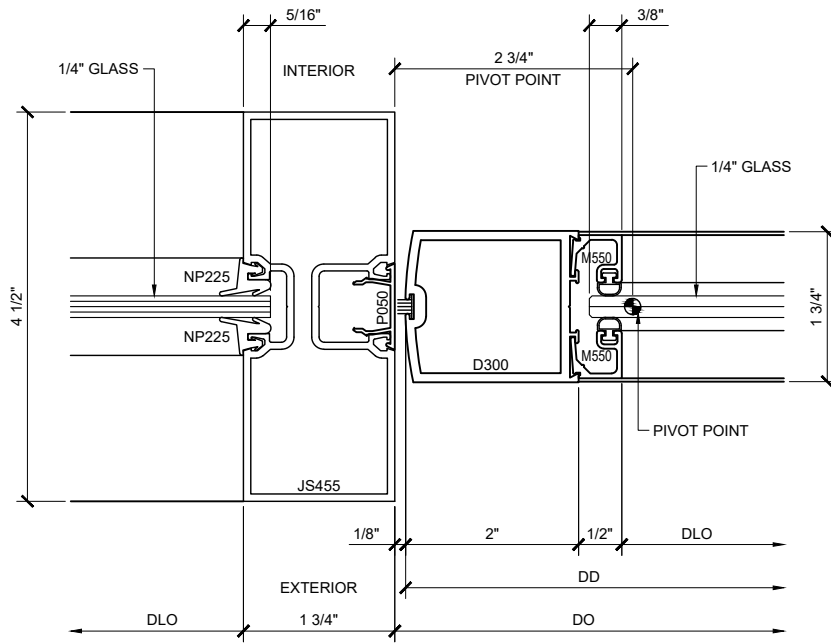
SECTION DETAIL @ VERTICAL (8A)
