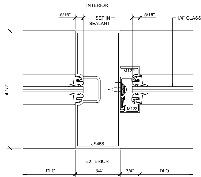
SECTION DETAIL @ DOOR JAMB (8B)
