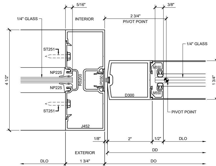
SECTION DETAIL @ MEETING STILES (8C)
