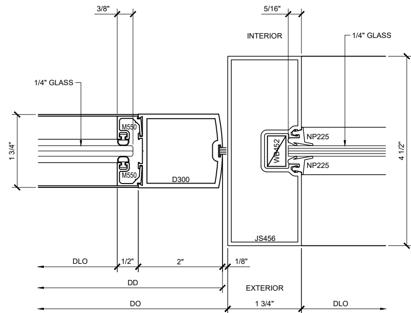
SECTION DETAIL @ DOOR JAMB 11
